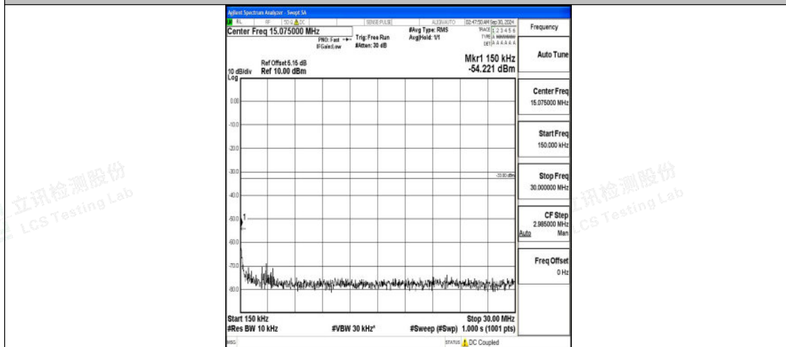
Band66_1.4MHz_QPSK_131979_1RB#0_0.15~30_0.15~30
