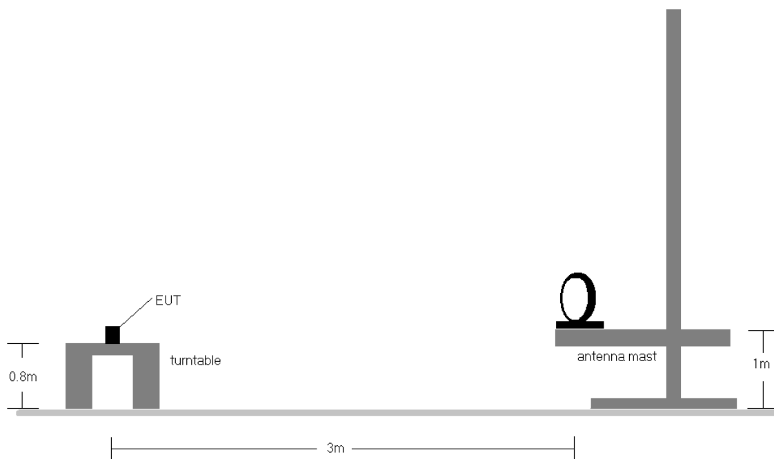
Figure 8-1. Radiated Test Setup < 30MHz
