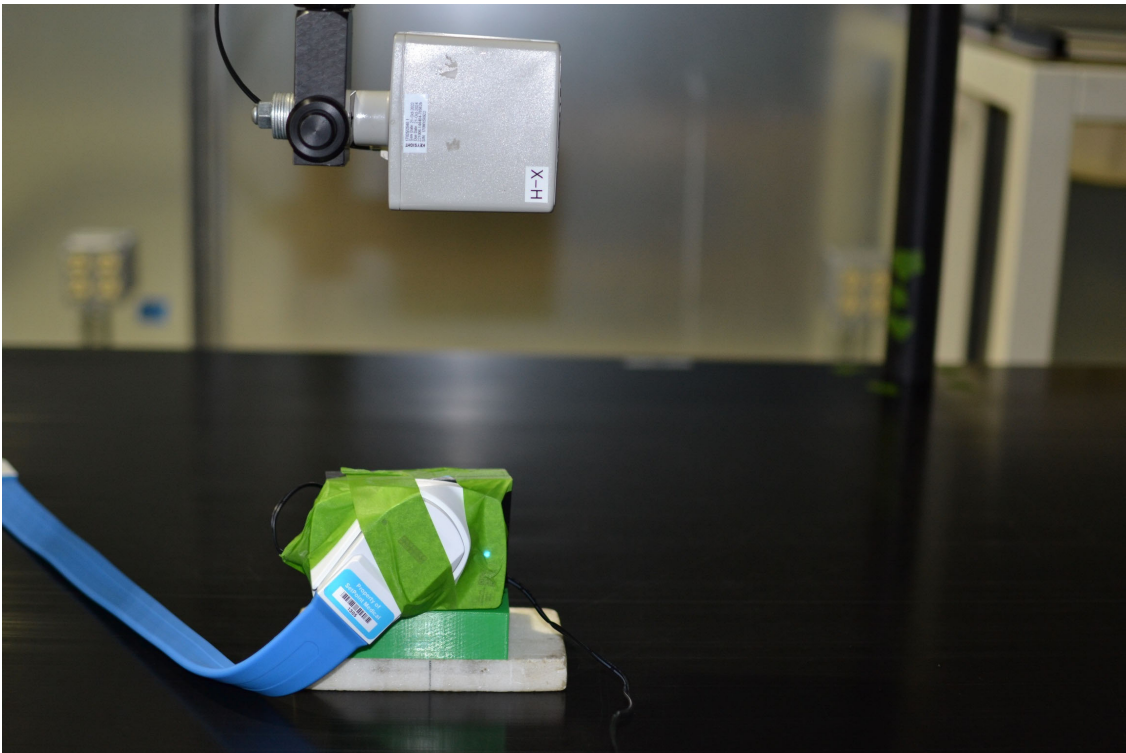
H-Field (Front)
