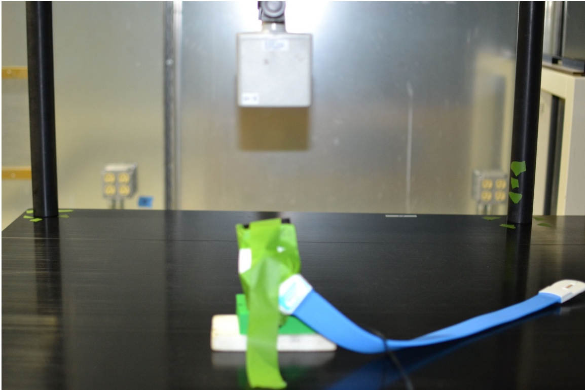
H-Field (Left)
