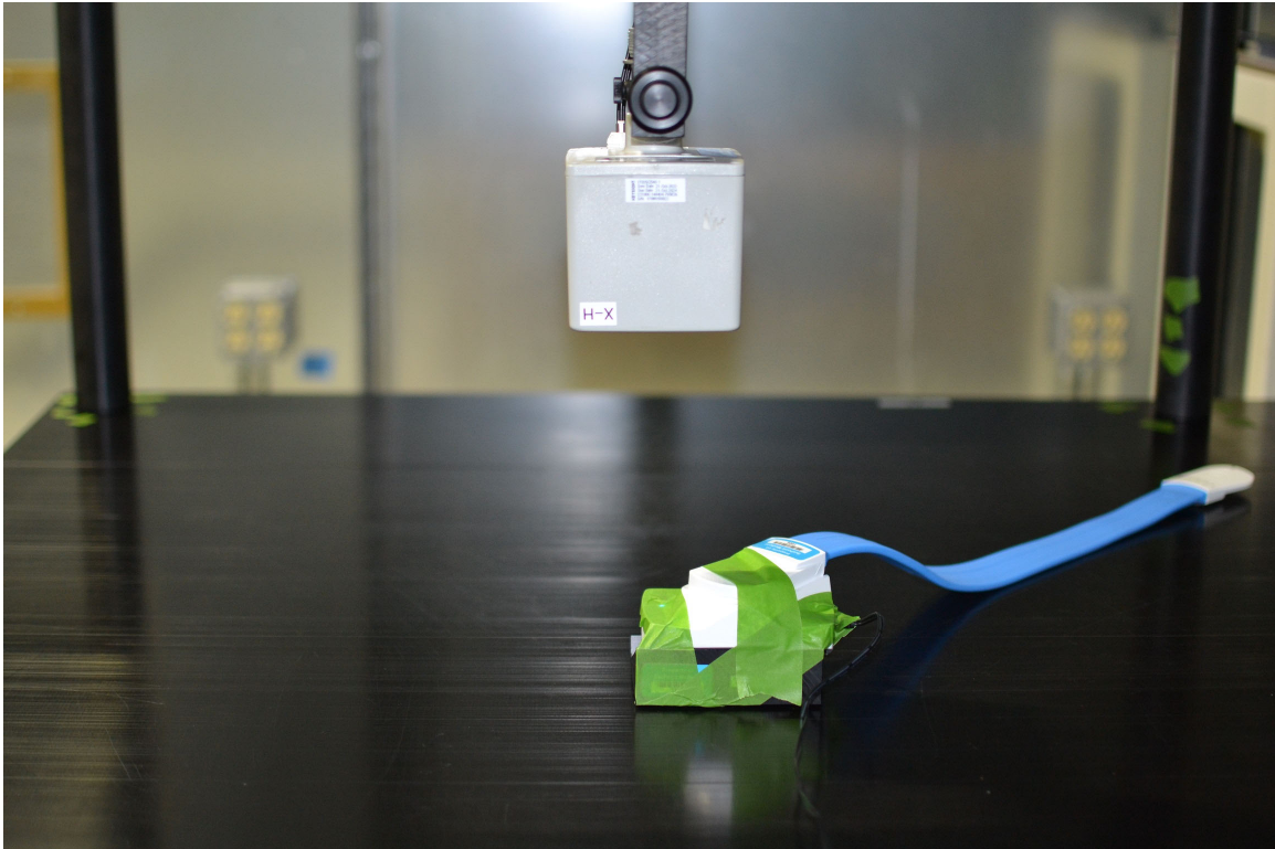
H-Field (Top)
