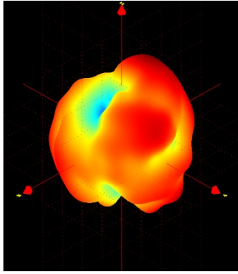
Wifi 5G 5140MHz
