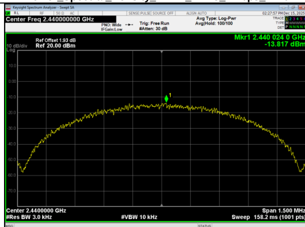
Power Spectral Density NVNT_ANT3_1Mbps_2440
