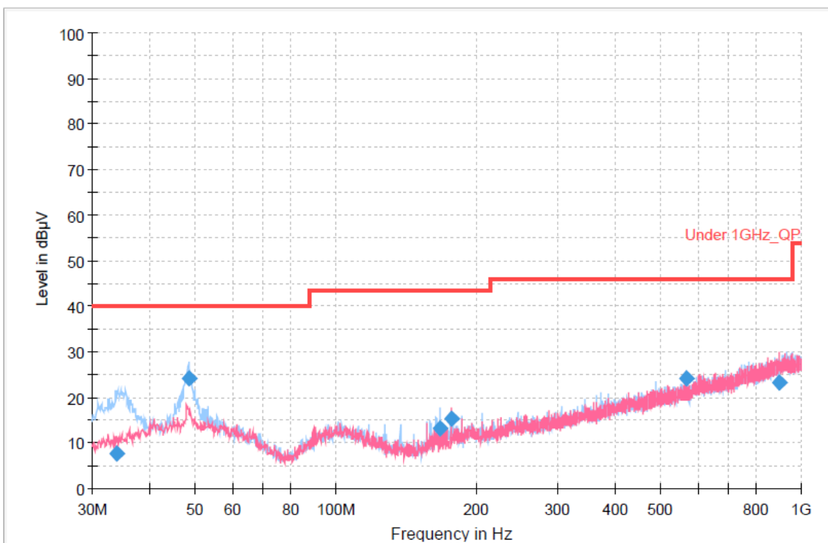
Worst case – RSE (Below 1 GHz)_TM 2
