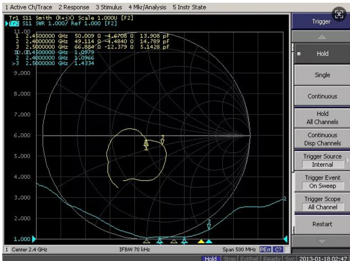
Antenna standing wave ratio and return loss
