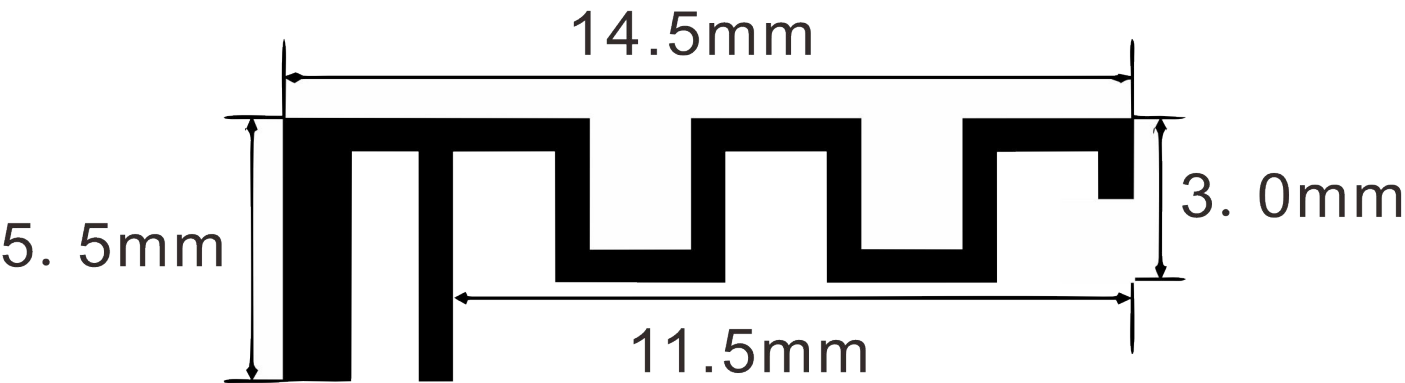
Antenna Photo & Length (mm)
