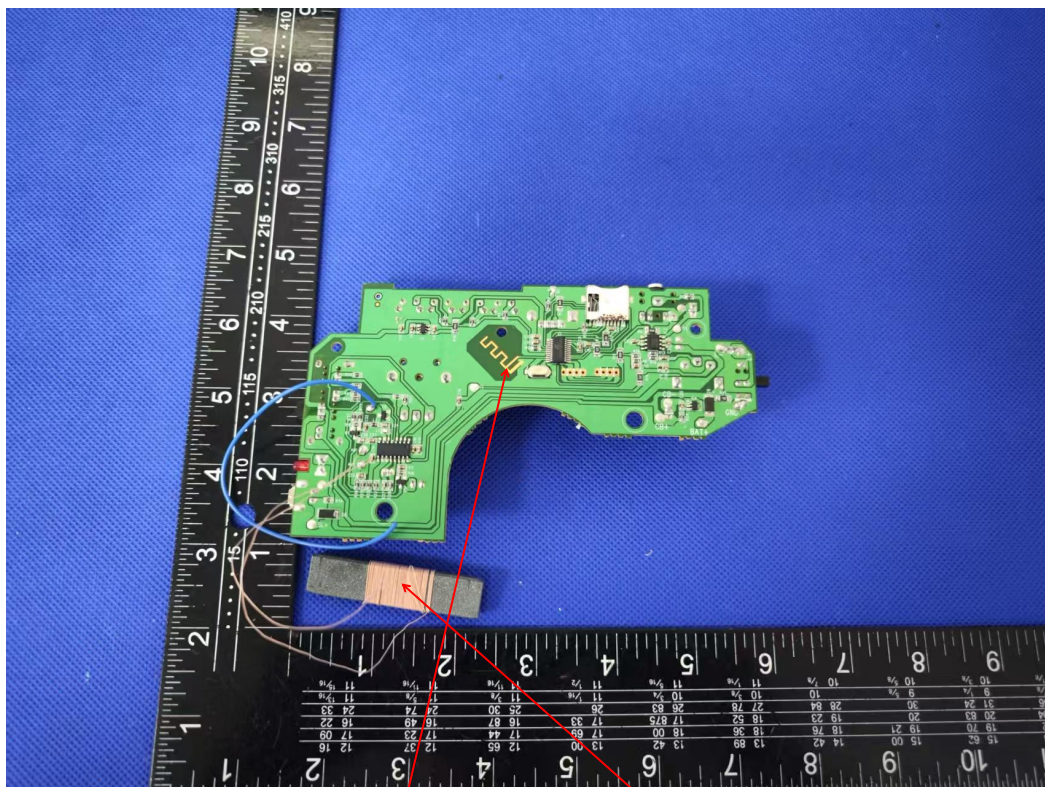
BT PCB antenna RX FM antenna
