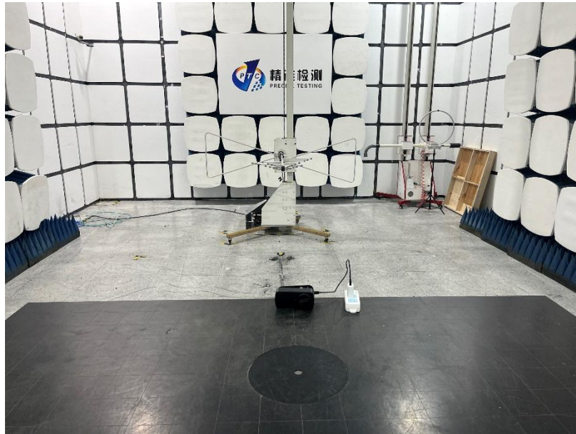
From 30MHz-1000MHz
