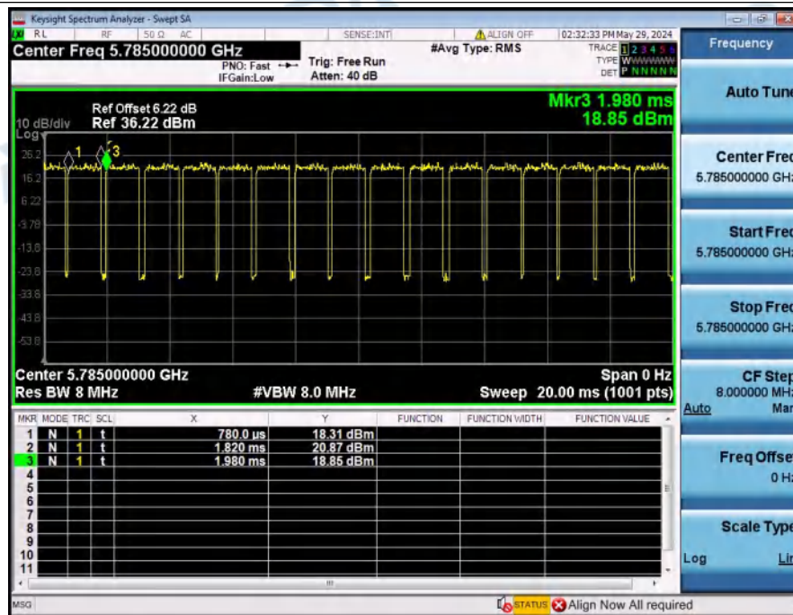
Duty_Cycle_NVNT_ANT1_802_11a_5785
