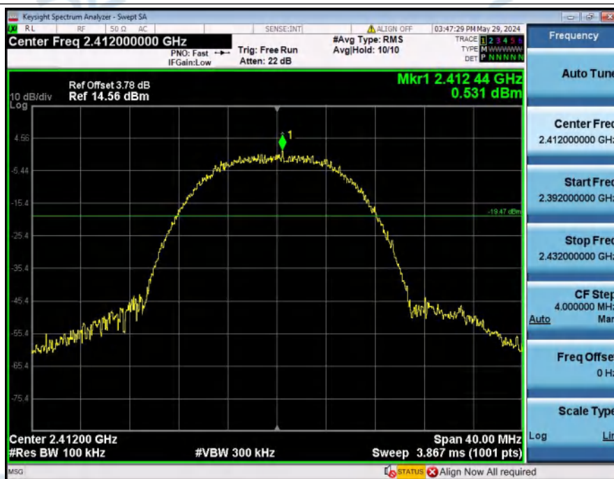
1_Reference_Level_NVNT_ANT1_802_11b_2412
