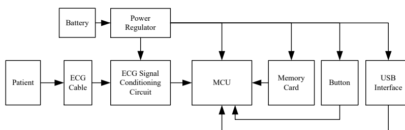
Electrical Principle Block Diagram of the Recorder
