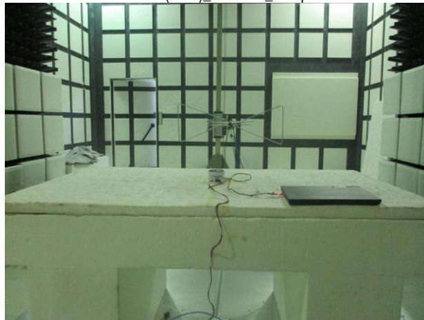
WLAN(2.4G)_Radiated_Setup
