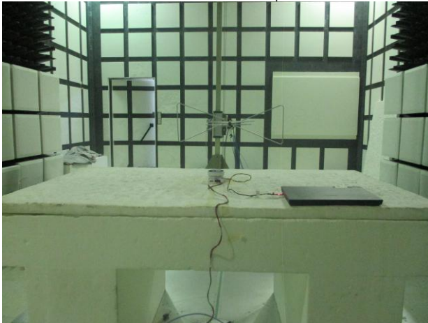
BLE_Radiated_Setup
