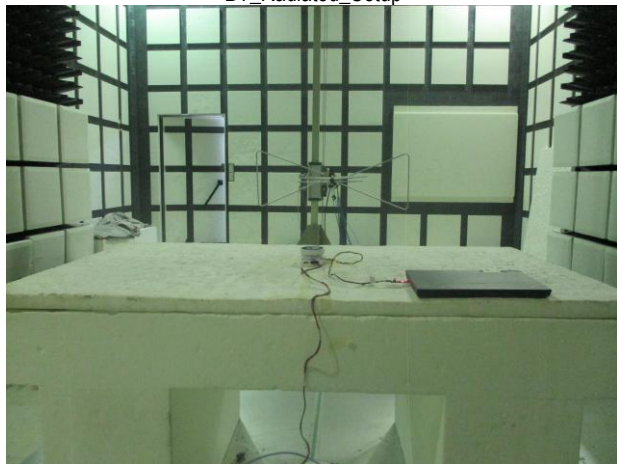
BT_Radiated_Setup
