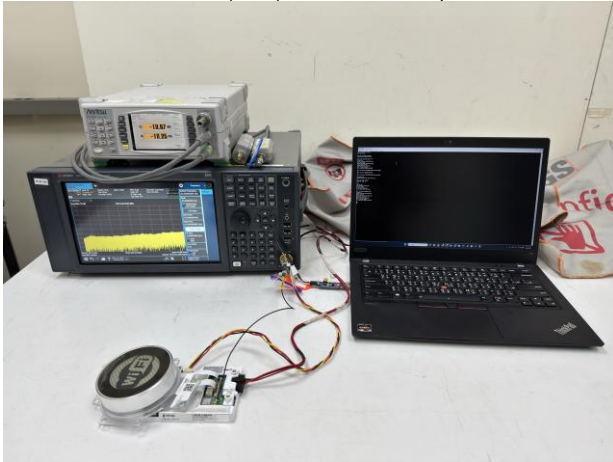
WLAN(5G)_Conducted_Setup
