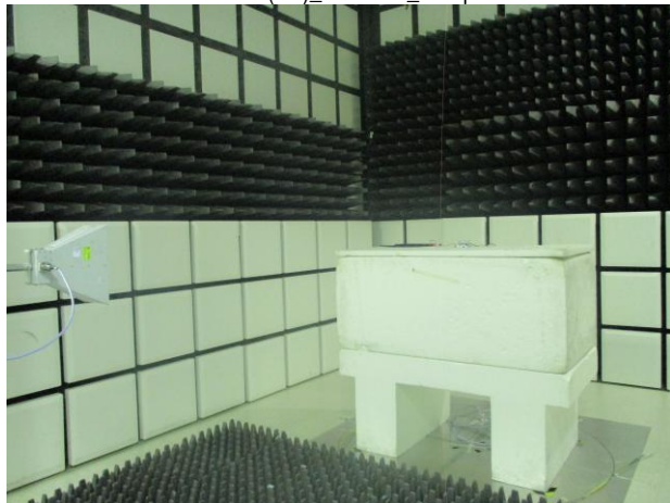
WLAN(5G)_Radiated_Setup
