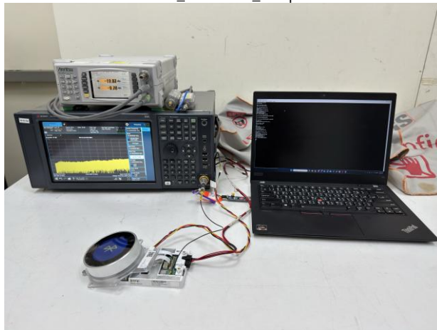
BT_Conducted_Setup
