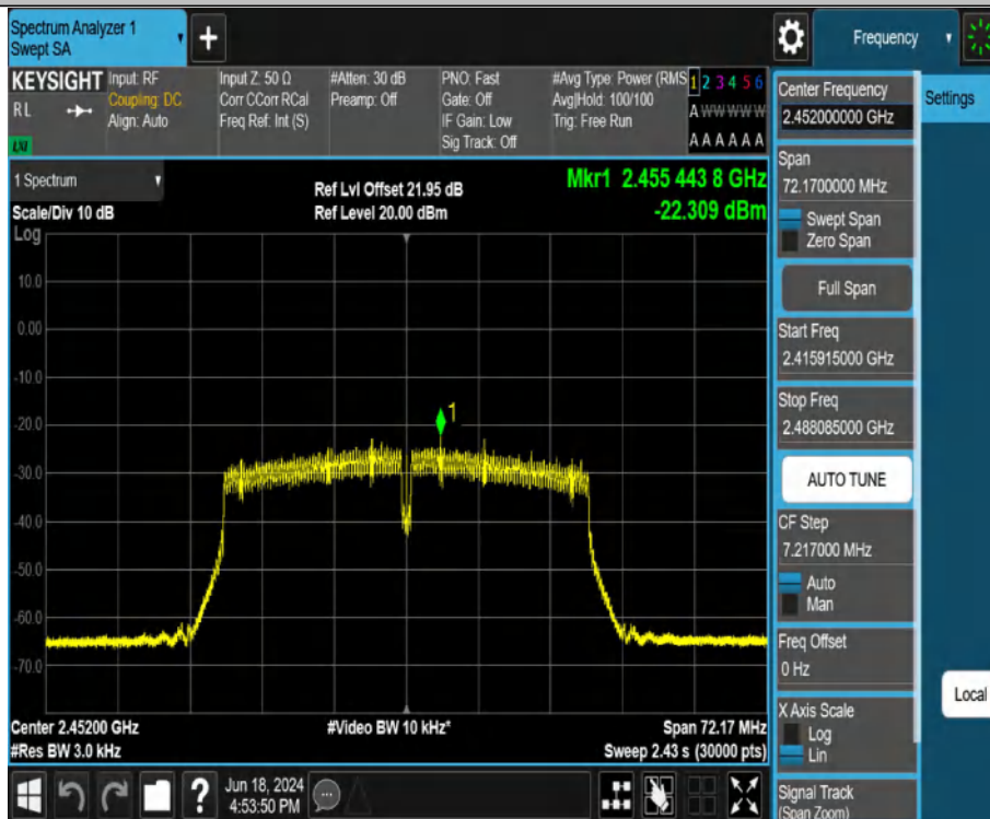
11N40SISO_Ant1_2452
