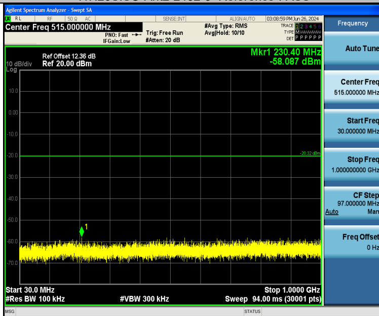
11N20SISO-Ant2-2462-30~1000-PASS
