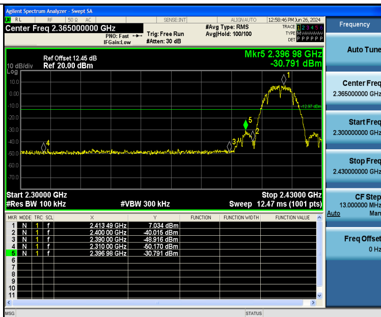
11B-Ant2-2412-PASS
