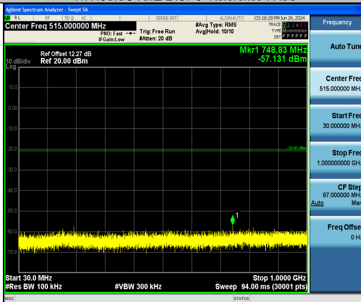
11N40SISO-Ant2-2437-30~1000-PASS
