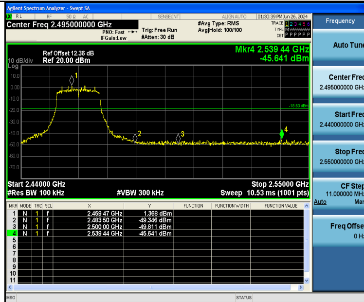
11G-Ant2-2462-PASS
