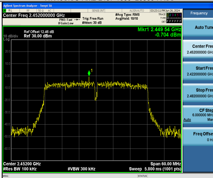
11N40SISO-Ant2-2452-0~Reference-PASS
