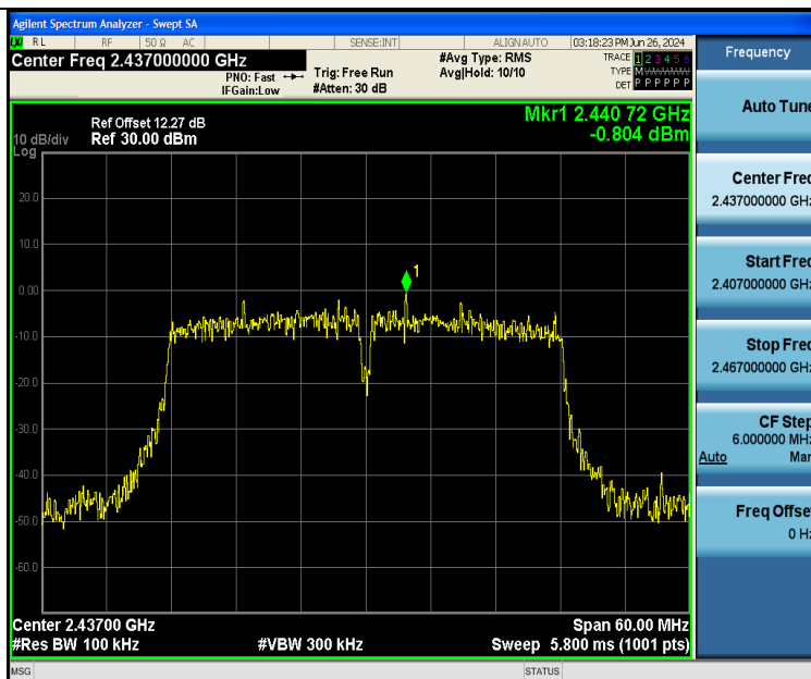
11N40SISO-Ant2-2437-0~Reference-PASS
