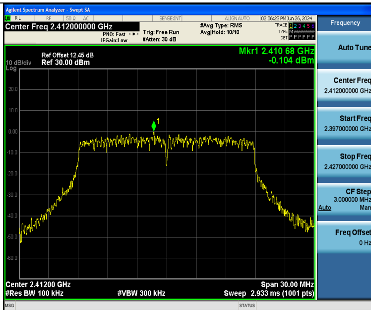
11N20SISO-Ant2-2412-0~Reference-PASS
