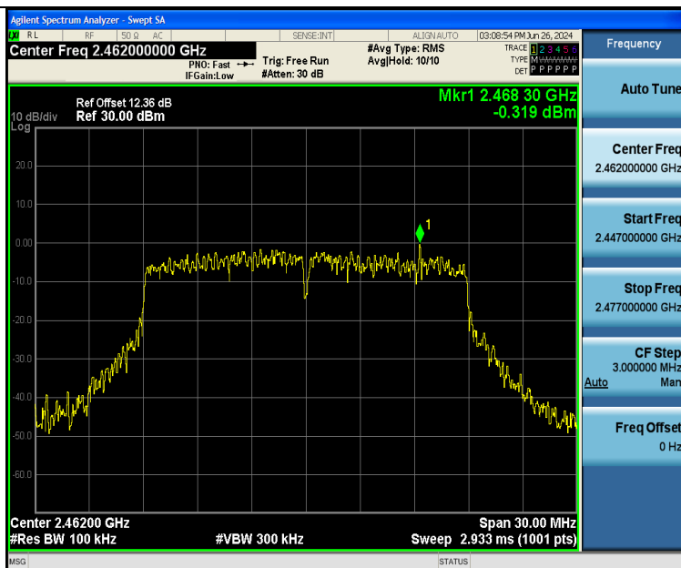
11N20SISO-Ant2-2462-0~Reference-PASS
