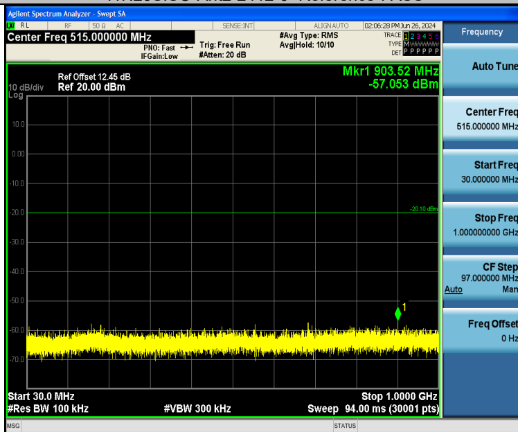
11N20SISO-Ant2-2412-30~1000-PASS
