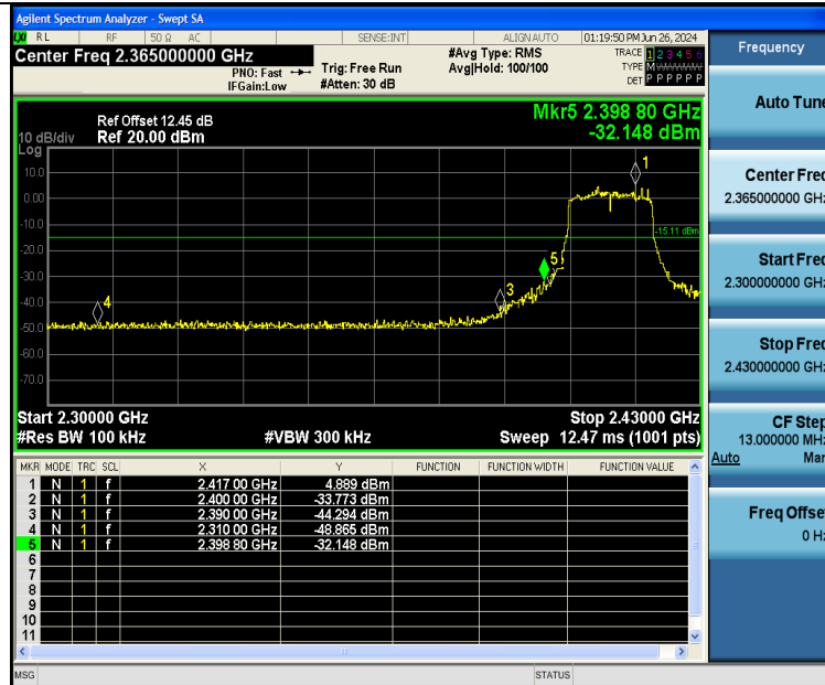
11G-Ant2-2412-PASS
