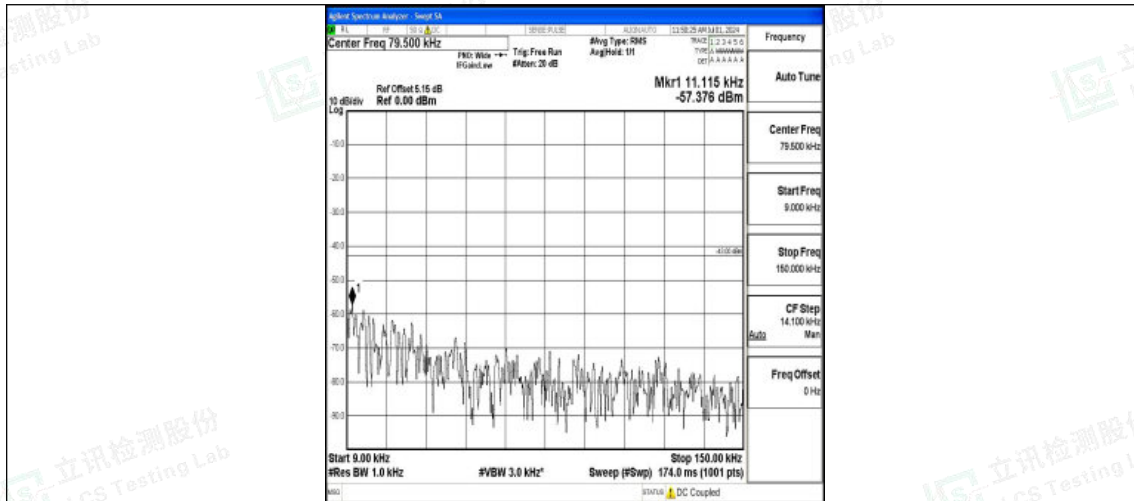
Band2_10MHz_QPSK_18900_1RB#0_0.009~0.15_0.009~0.15
