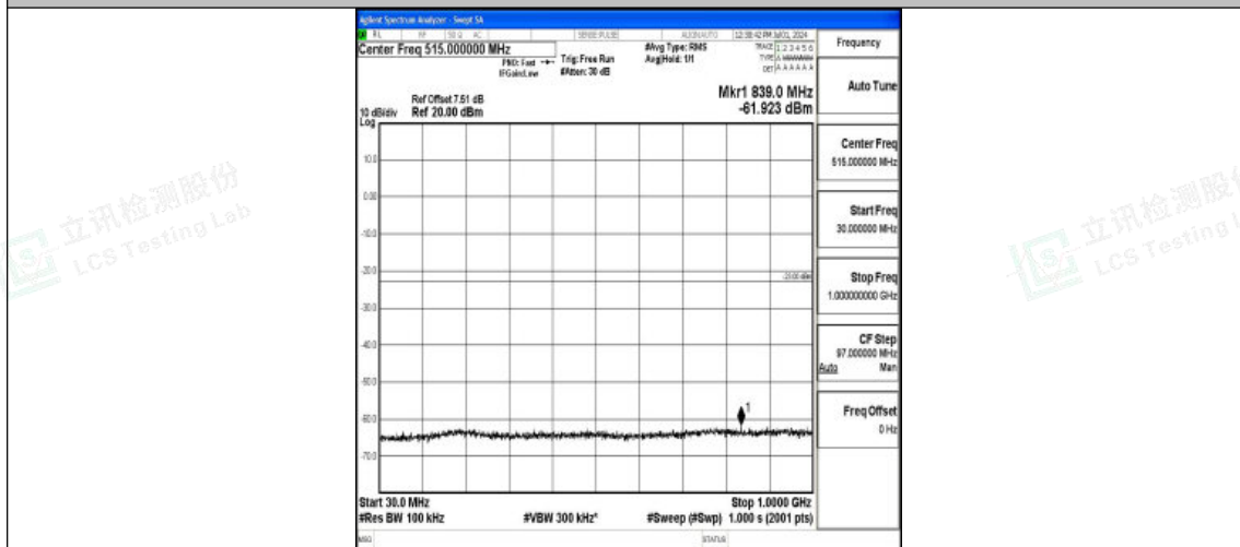
Band2_20MHz_QPSK_18900_1RB#0_30~1000_30~1000
