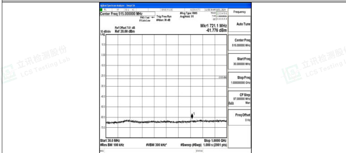
Band2_10MHz_QPSK_18900_1RB#0_30~1000_30~1000
