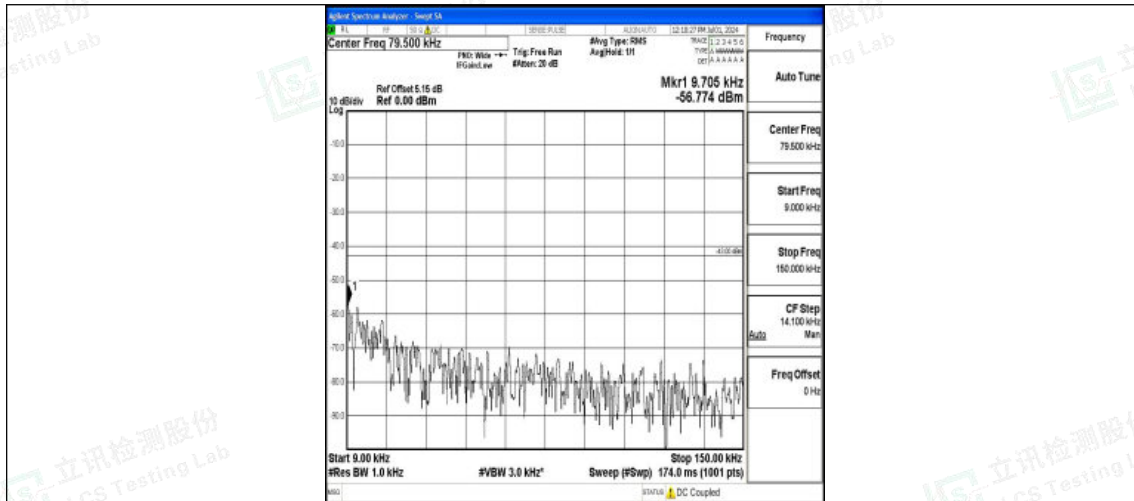
Band2_15MHz_QPSK_18900_1RB#0_0.009~0.15_0.009~0.15
