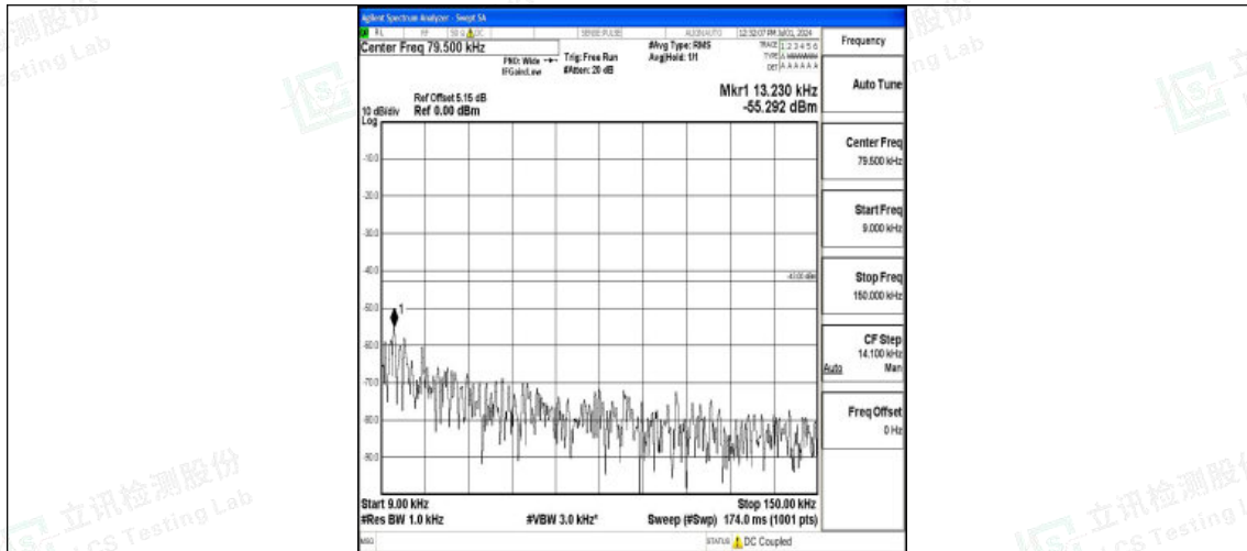
Band2_20MHz_16QAM_19100_1RB#0_0.009~0.15_0.009~0.15
