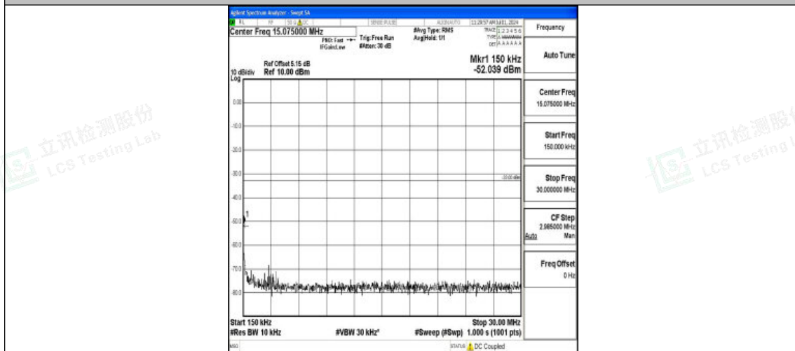
Band2_5MHz_QPSK_19175_1RB#0_0.15~30_0.15~30
