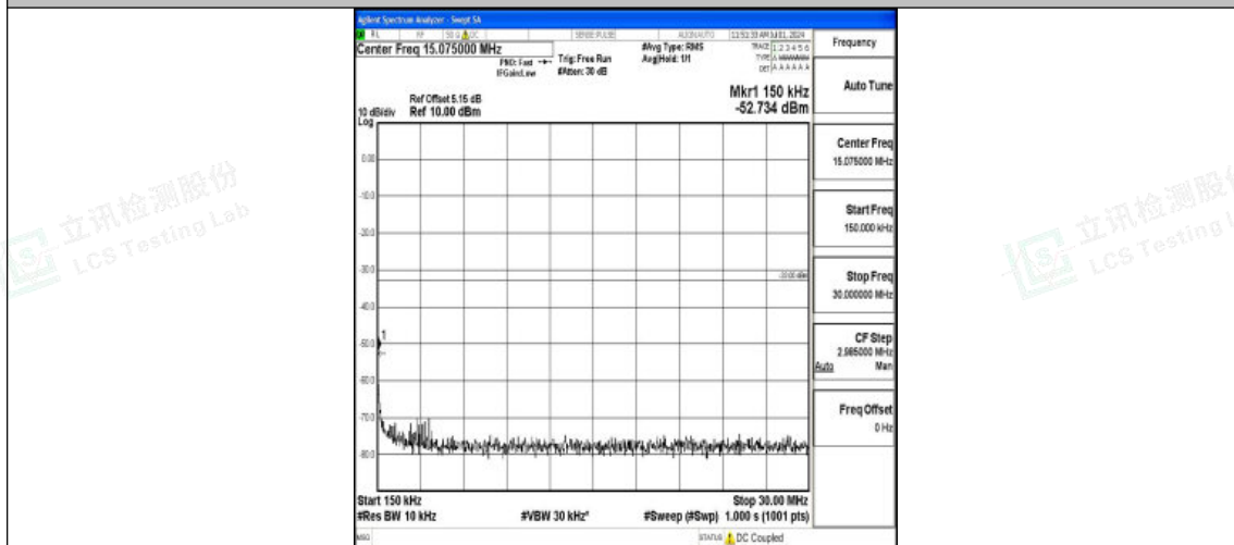
Band2_10MHz_QPSK_19150_1RB#0_0.15~30_0.15~30
