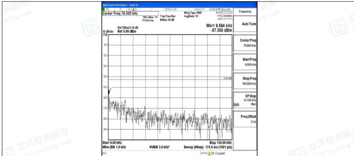
Band2_20MHz_QPSK_18900_1RB#0_0.009~0.15_0.009~0.15
