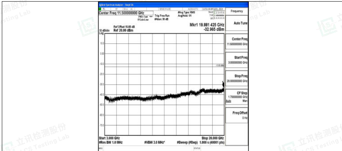
Band2_10MHz_16QAM_18900_1RB#0_3000~20000_3000~20000
