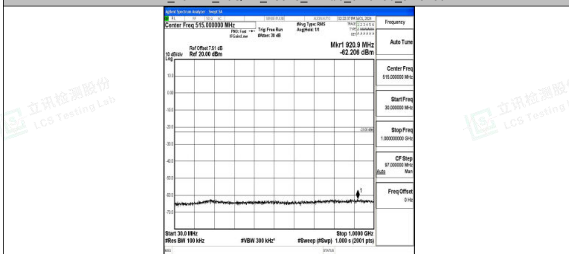
Band4_15MHz_16QAM_20325_1RB#0_30~1000_30~1000
