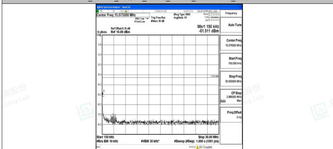
Band4_15MHz_16QAM_20325_1RB#0_0.15~30_0.15~30
