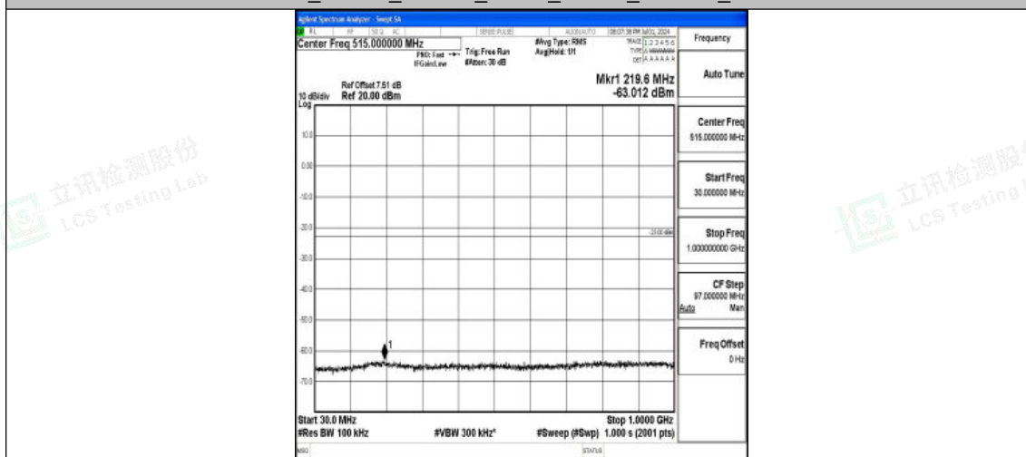
Band25_10MHz_16QAM_26640_1RB#0_30~1000_30~1000
