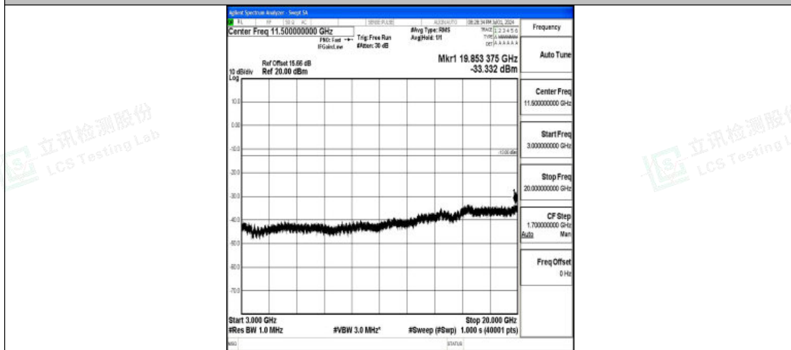
Band25_15MHz_16QAM_26115_1RB#0_3000~20000_3000~20000
