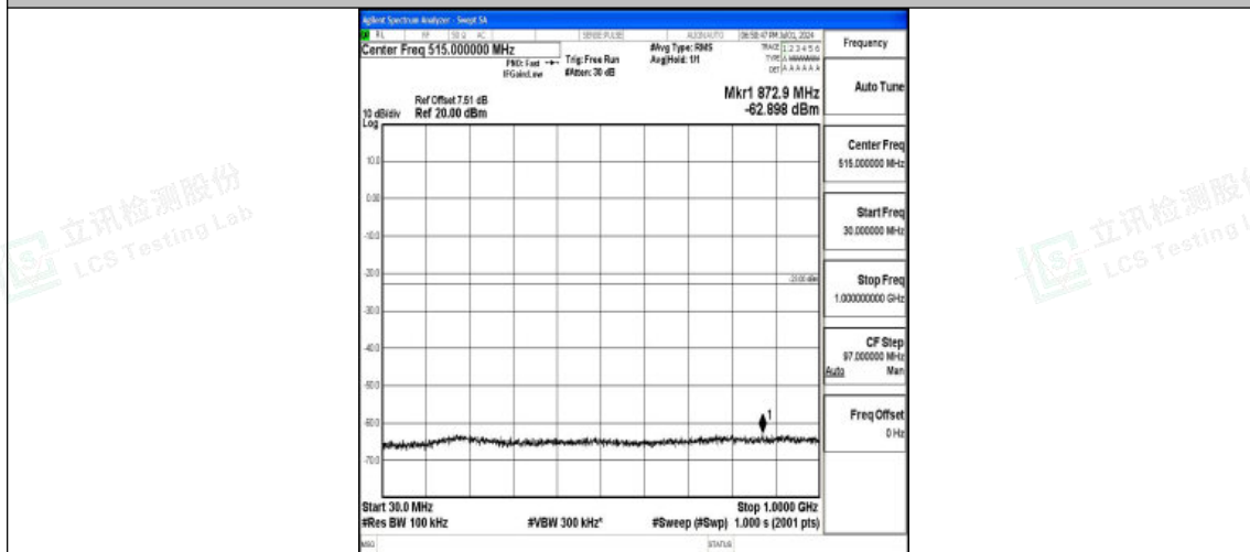
Band25_1.4MHz_16QAM_26683_1RB#0_30~1000_30~1000
