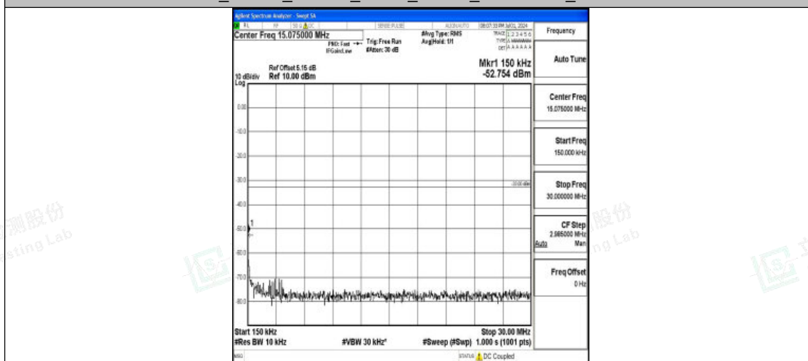
Band25_10MHz_16QAM_26640_1RB#0_0.15~30_0.15~30
