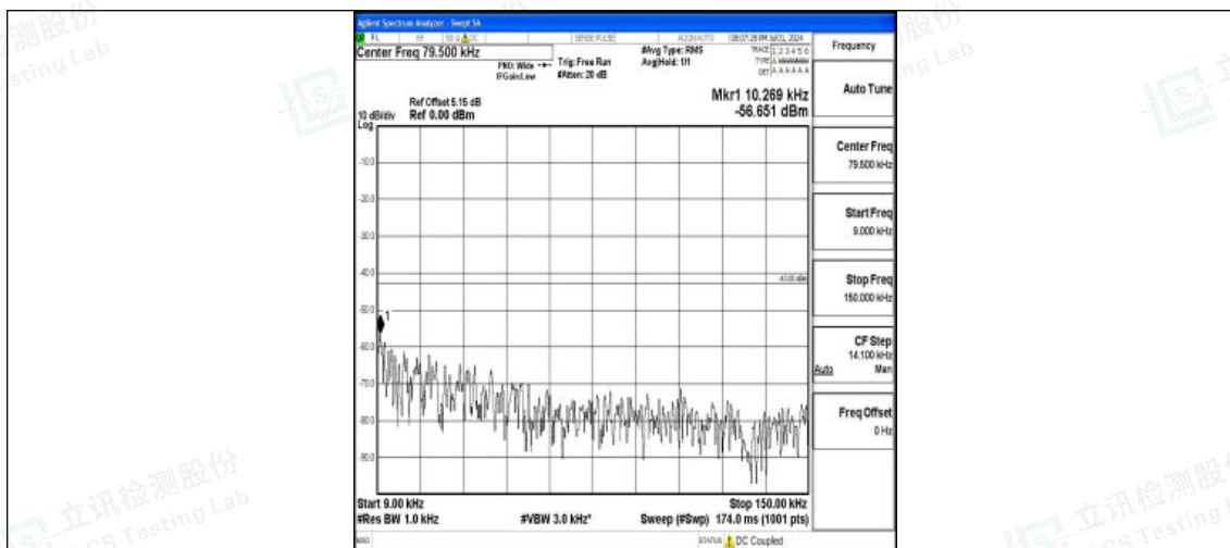
Band25_10MHz_16QAM_26640_1RB#0_0.009~0.15_0.009~0.15
