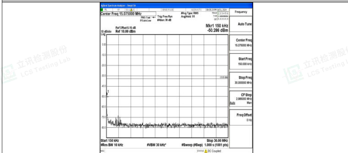
Band25_10MHz_16QAM_26090_1RB#0_0.15~30_0.15~30
