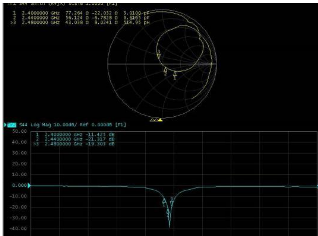
Return Loss
