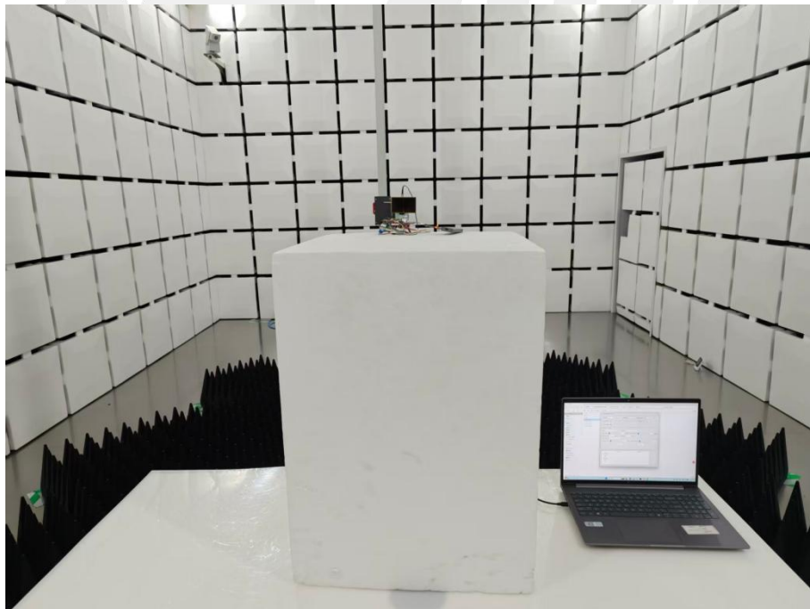
Emissions in frequency bands (18GHz~25GHz)
