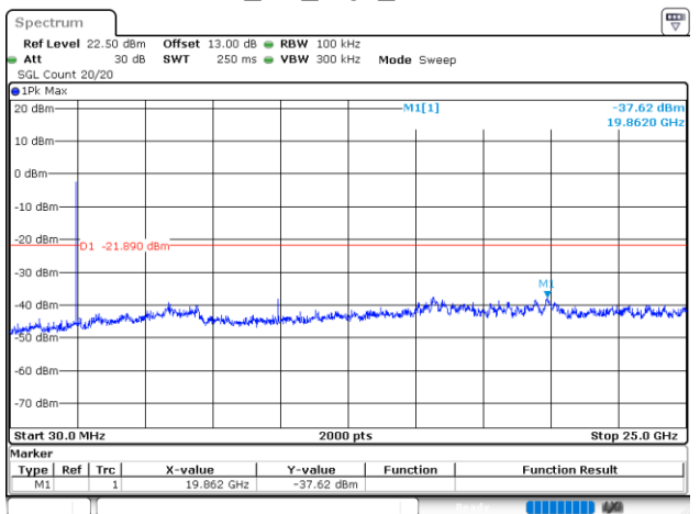
BLE_2M_High_Channel
