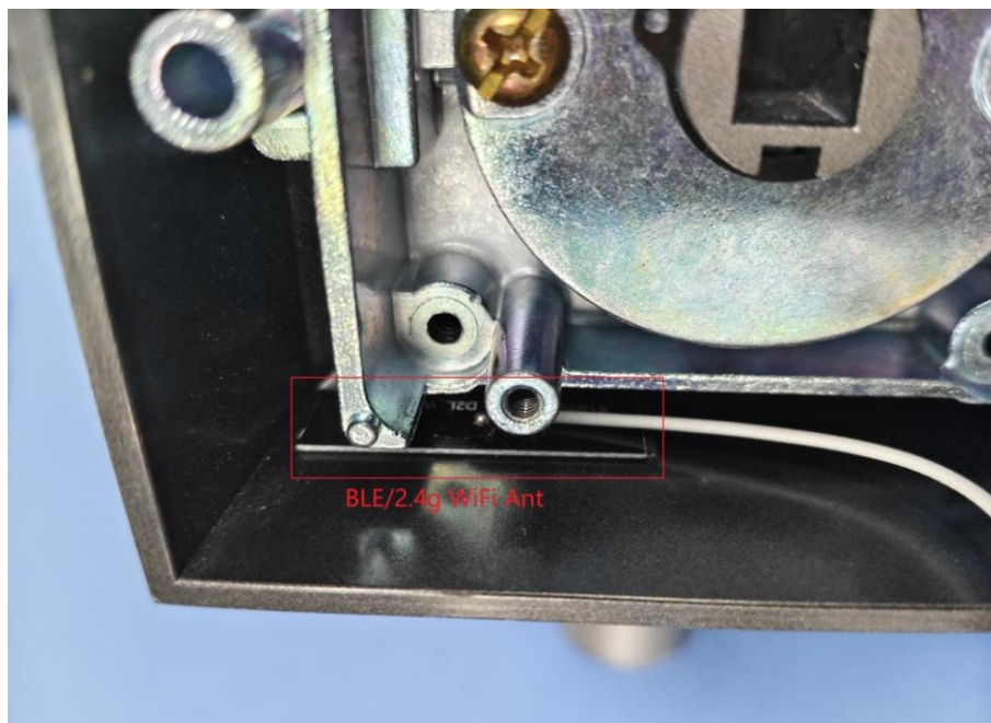
BLE(Chain 0) & 2.4G WIFI ANT
