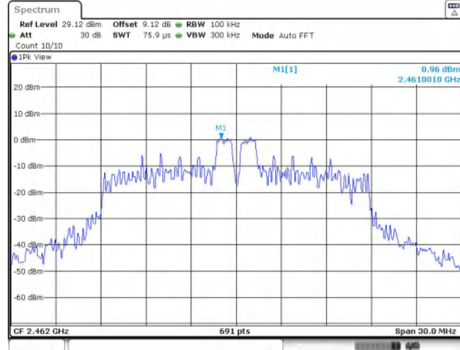
11AX20SISO_Ant1_2462_26Tone_RU4_0~Reference
