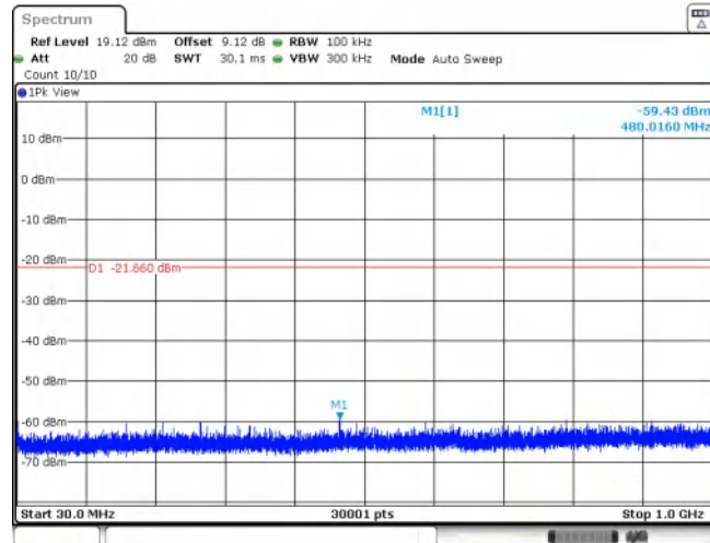
11AX20SISO_Ant1_2412_52Tone_RU39_30~1000
