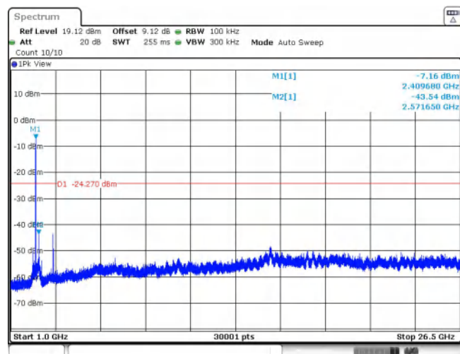
11AX20SISO_Ant1_2412_106Tone_RU53_1000~26500
