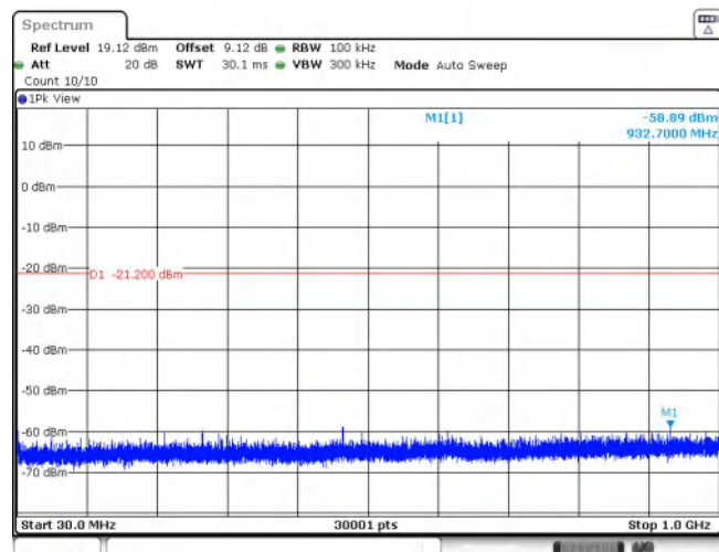
11AX20SISO_Ant1_2437_26Tone_RU8_0~Reference
