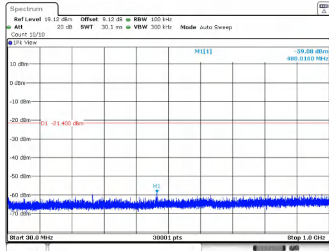
11AX20SISO_Ant1_2462_26Tone_RU8_30~1000
