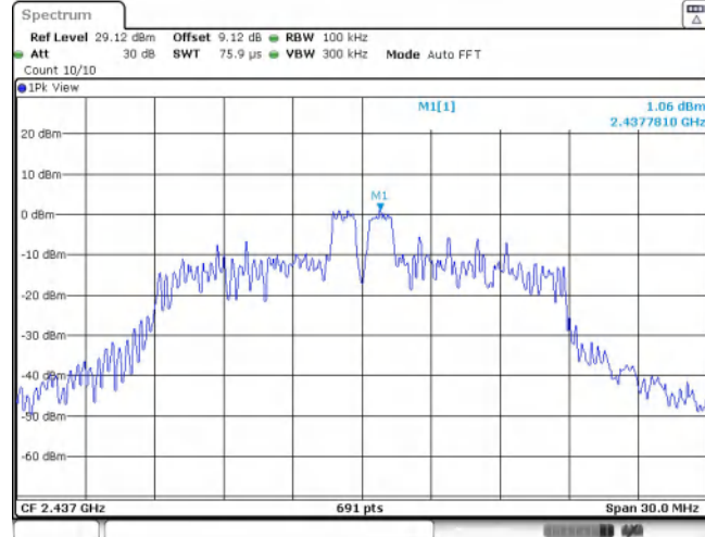
11AX20SISO_Ant1_2437_26Tone_RU4_0~Reference
