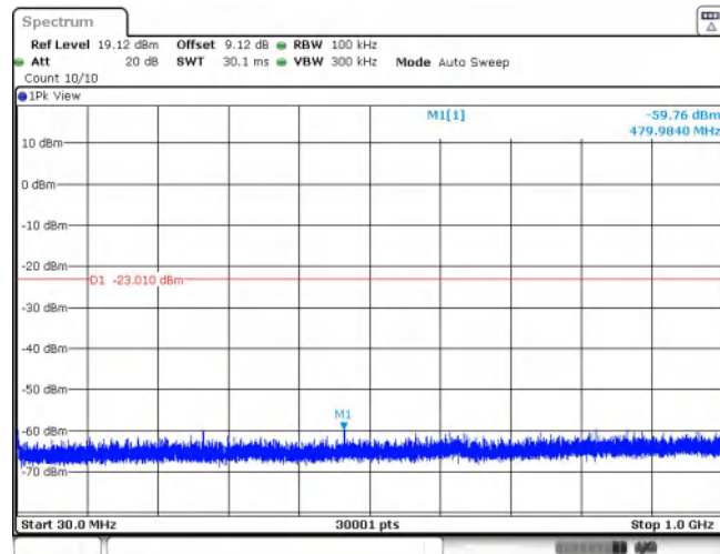
11AX20SISO_Ant1_2412_52Tone_RU37_30~1000
