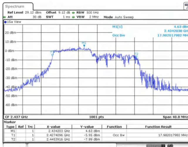
11AX20SISO_Ant1_2437_52Tone_RU40
