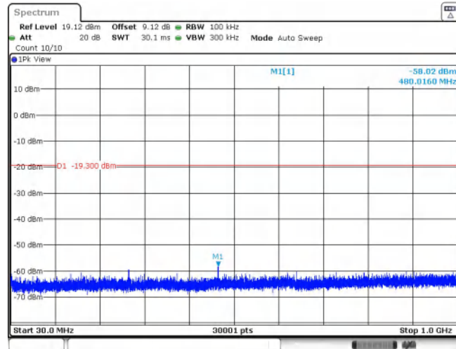
11AX20SISO_Ant1_2412_26Tone_RU4_30~1000
