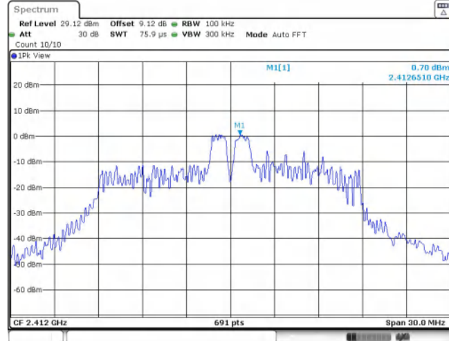
11AX20SISO_Ant1_2412_26Tone_RU_0~Reference
