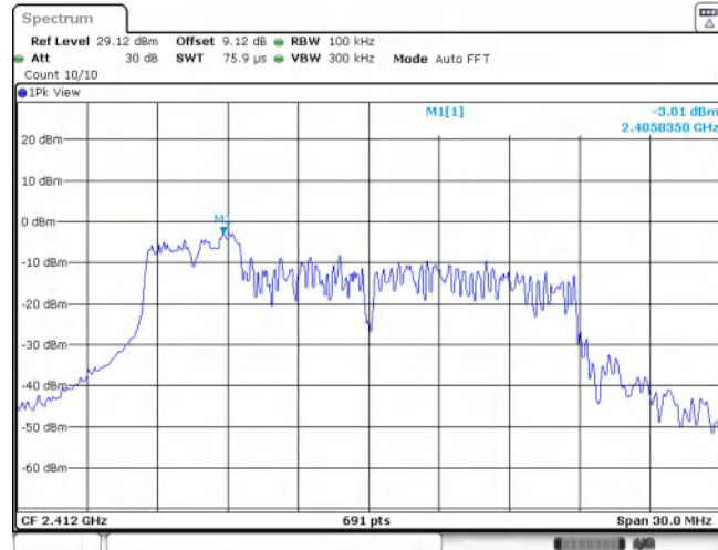
11AX20SISO_Ant1_2412_52Tone_RU37_0~Reference
