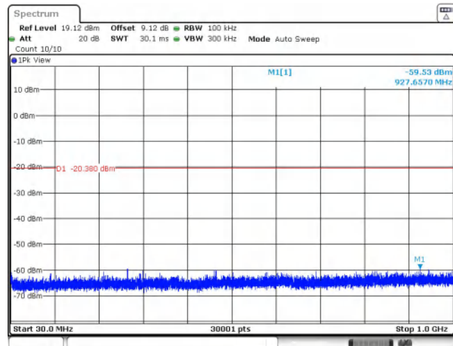
11AX20SISO_Ant1_2462_52Tone_RU39_30~1000
