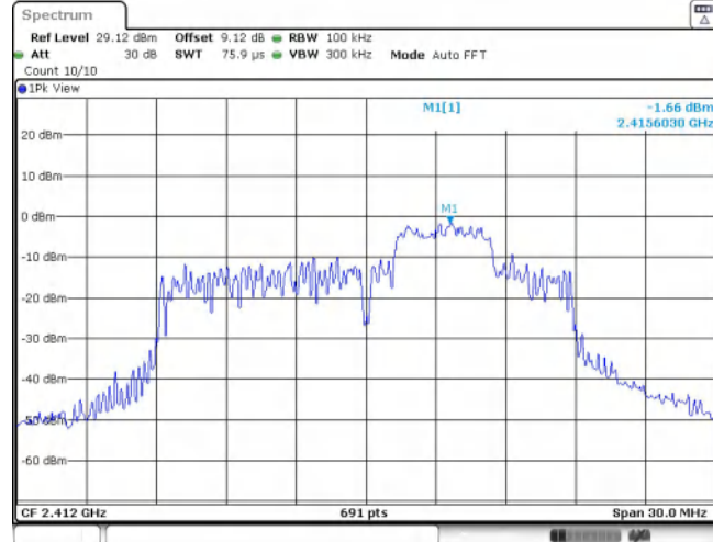
11AX20SISO_Ant1_2412_52Tone_RU39_0~Reference
