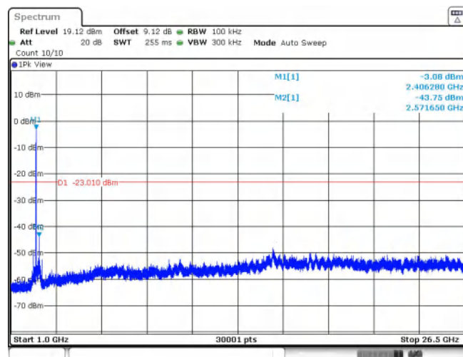
11AX20SISO_Ant1_2412_52Tone_RU37_1000~26500
