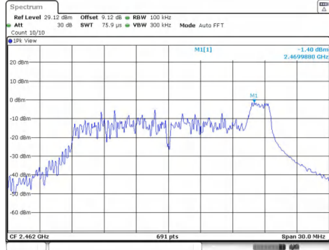
11AX20SISO_Ant1_2462_26Tone_RU8_0~Reference
