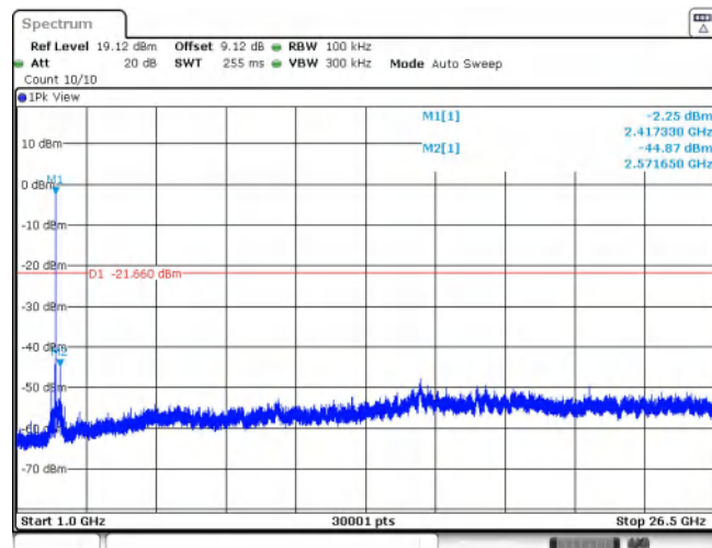
11AX20SISO_Ant1_2412_52Tone_RU39_1000~26500
