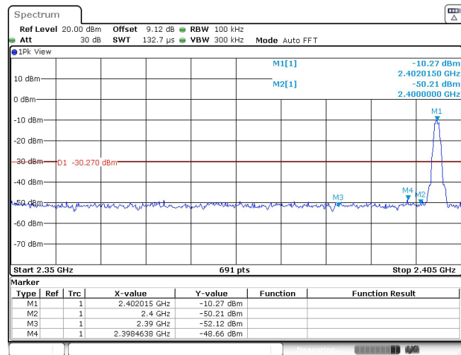
BLE_1M_Ant1_Low_2402
