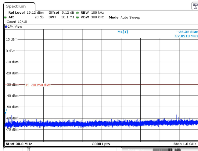
BLE_1M_Ant1_2402_0~Reference
