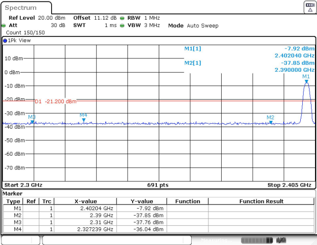
BLE_1M_Ant1_Low_2402_Peak
