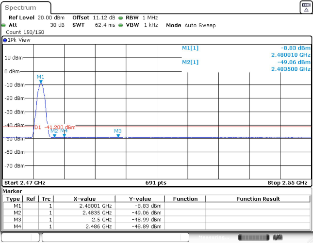
BLE_1M_Ant1_High_2480_AV
