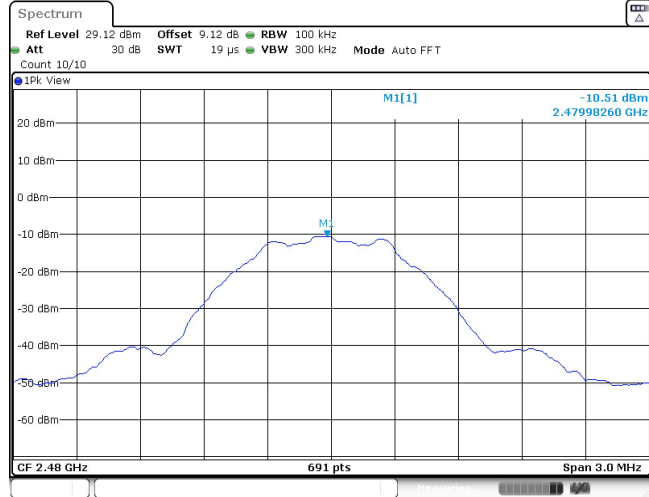
BLE_1M_Ant1_2480_0~Reference
