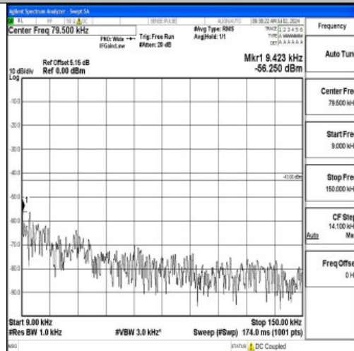
Band2_10MHz_16QAM_18650_1RB#0_0.009~0.15_0.009~0.15
