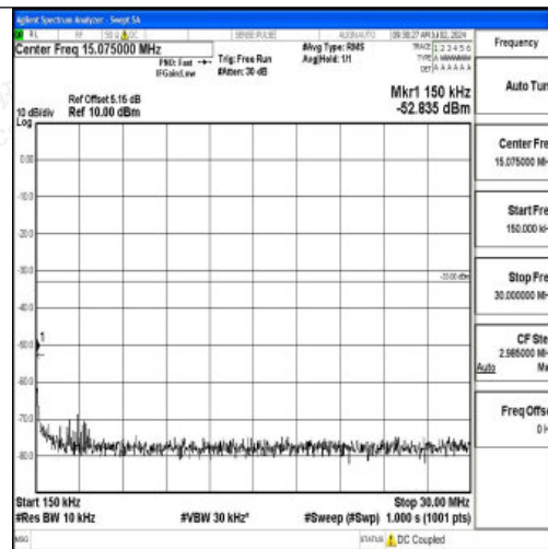
Band2_10MHz_16QAM_18650_1RB#0_0.15~30_0.15~30
