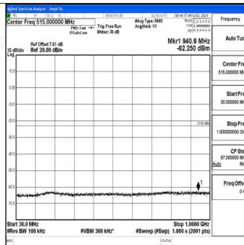
Band2_3MHz_16QAM_19185_1RB#0_30~1000_30~1000
