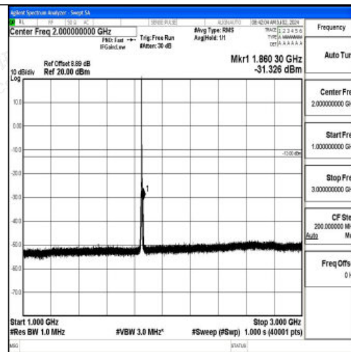
Band2_3MHz_QPSK_18615_1RB#0_1000~3000_1000~3000
