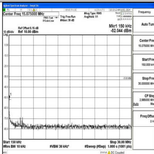
Band2_20MHz_QPSK_18700_1RB#0_0.15~30_0.15~30
