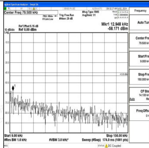
Band2_10MHz_16QAM_19150_1RB#0_0.009~0.15_0.009~0.15
