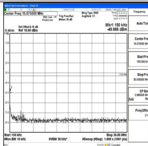
Band2_5MHz_16QAM_19175_1RB#0_0.15~30_0.15~30
