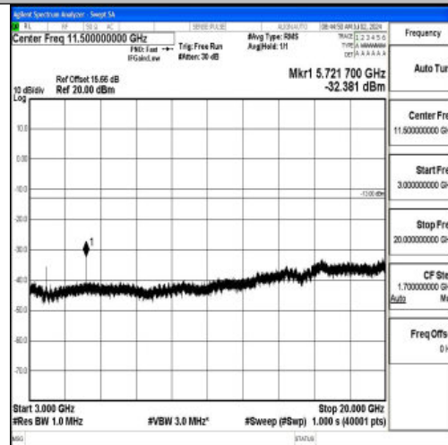
Band2_3MHz_16QAM_19185_1RB#0_3000~20000_3000~20000
