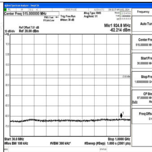
Band2_10MHz_16QAM_19150_1RB#0_30~1000_30~1000
