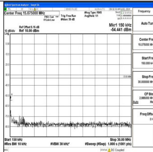
Band2_10MHz_16QAM_19150_1RB#0_0.15~30_0.15~30
