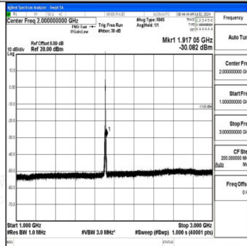
Band2_3MHz_16QAM_19185_1RB#0_1000~3000_1000~3000
