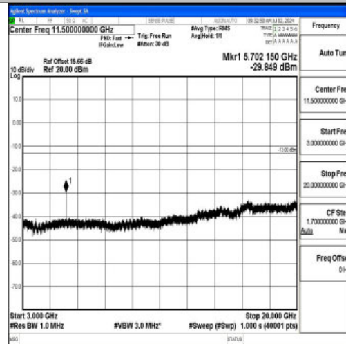
Band2_10MHz_16QAM_19150_1RB#0_3000~20000_3000~20000
