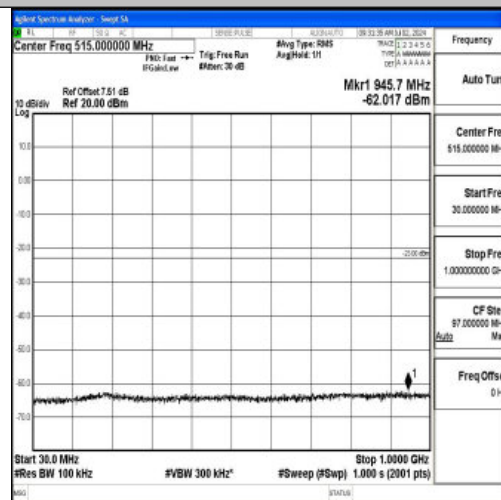
Band2_10MHz_16QAM_18900_1RB#0_30~1000_30~1000
