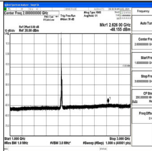
Band2_10MHz_16QAM_18650_1RB#0_1000~3000_1000~3000
