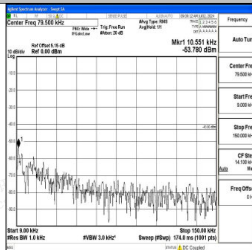
Band2_5MHz_16QAM_19175_1RB#0_0.009~0.15_0.009~0.15
