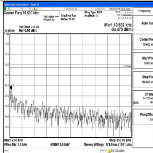
Band12_5MHz_QPSK_23035_1RB#0_0.009~0.15_0.009~0.15
