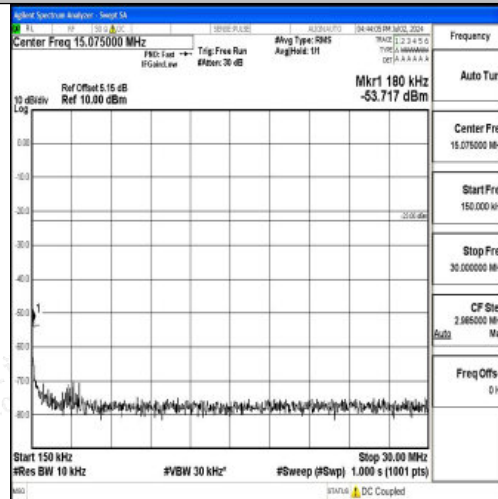
Band12_3MHz_16QAM_23025_1RB#0_0.15~30_0.15~30
