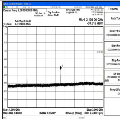
Band12_10MHz_QPSK_23095_1RB#0_1000~3000_1000~3000
