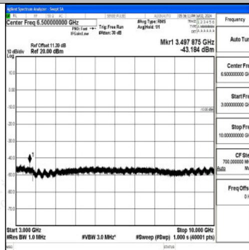
Band12_10MHz_16QAM_23060_1RB#0_3000~10000_3000~10000
