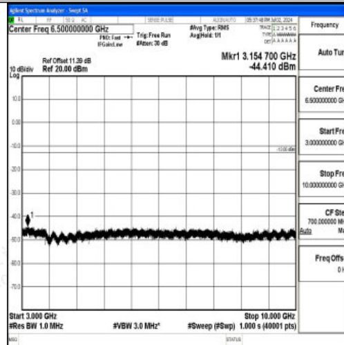
Band12_10MHz_QPSK_23130_1RB#0_3000~10000_3000~10000
