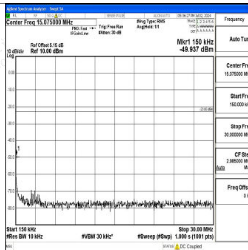
Band12_10MHz_QPSK_23095_1RB#0_0.15~30_0.15~30
