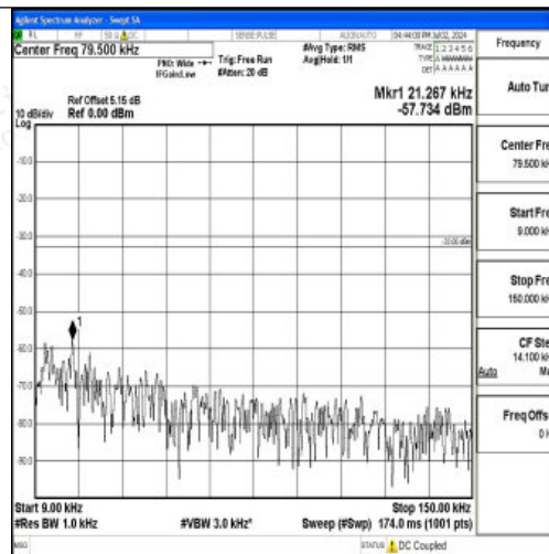
Band12_3MHz_16QAM_23025_1RB#0_0.009~0.15_0.009~0.15
