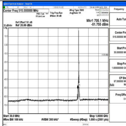
Band12_3MHz_16QAM_23165_1RB#0_30~1000_30~1000
