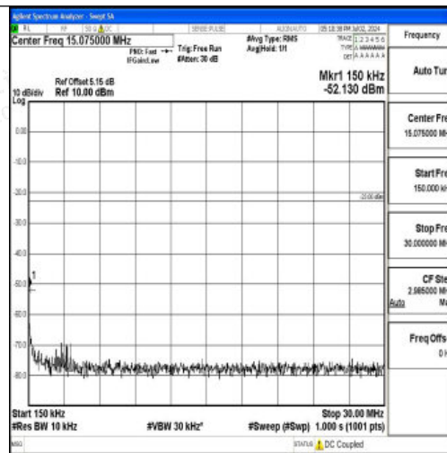
Band12_5MHz_QPSK_23095_1RB#0_0.15~30_0.15~30
