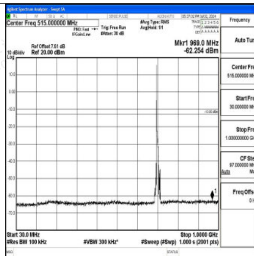
Band12_10MHz_16QAM_23095_1RB#0_30~1000_30~1000
