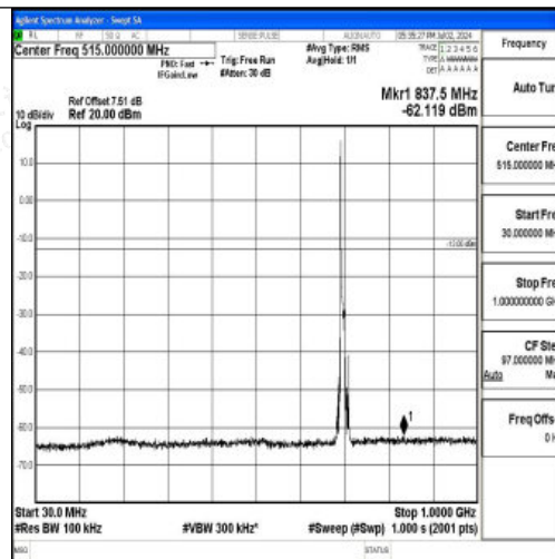
Band12_10MHz_QPSK_23060_1RB#0_30~1000_30~1000
