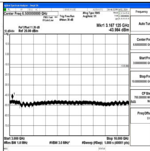
Band12_3MHz_16QAM_23165_1RB#0_3000~10000_3000~10000
