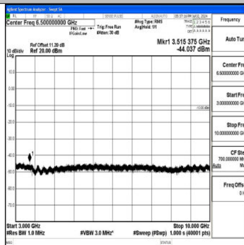
Band12_10MHz_16QAM_23095_1RB#0_3000~10000_3000~10000
