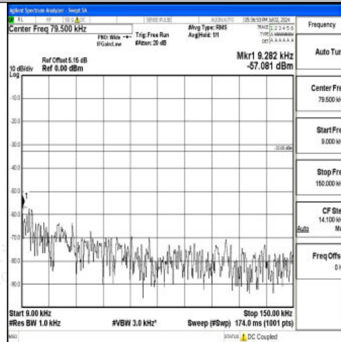
Band12_10MHz_16QAM_23095_1RB#0_0.009~0.15_0.009~0.15
