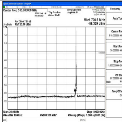
Band12_5MHz_16QAM_23155_1RB#0_30~1000_30~1000
