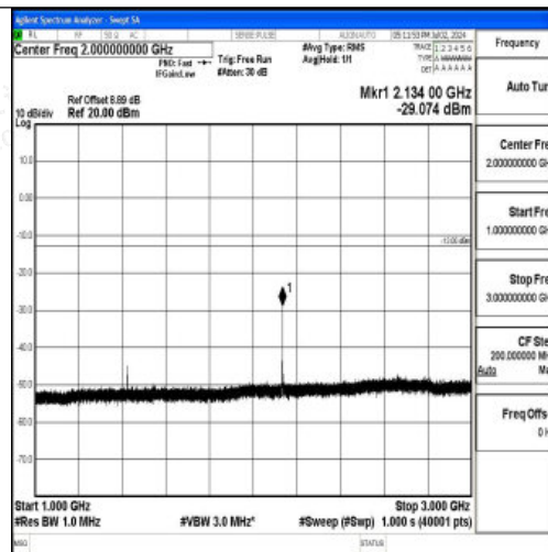
Band12_5MHz_QPSK_23155_1RB#0_1000~3000_1000~3000
