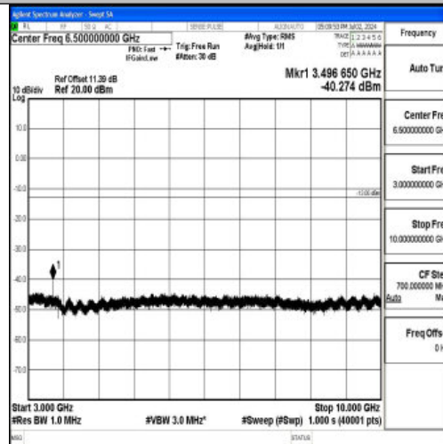
Band12_5MHz_QPSK_23035_1RB#0_3000~10000_3000~10000
