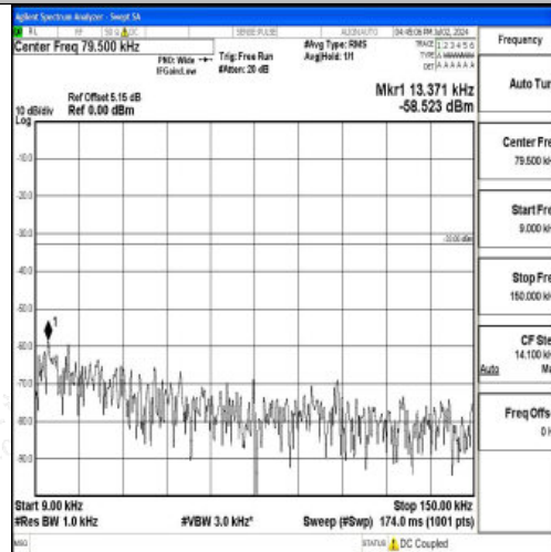
Band12_3MHz_16QAM_23095_1RB#0_0.009~0.15_0.009~0.15
