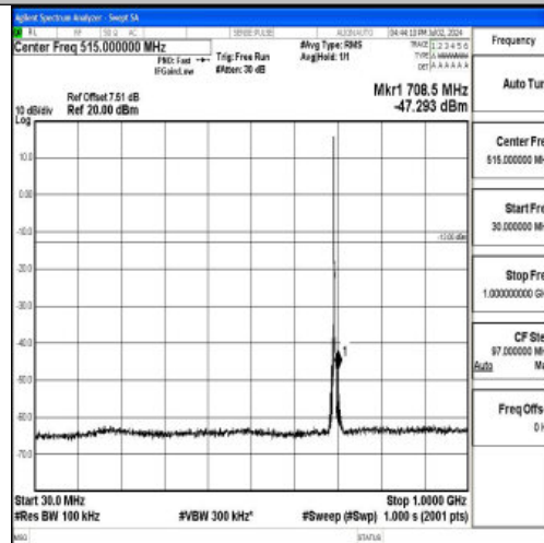
Band12_3MHz_16QAM_23025_1RB#0_30~1000_30~1000
