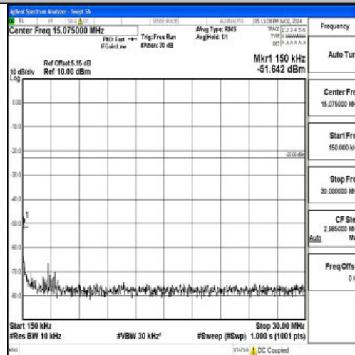
Band12_5MHz_16QAM_23095_1RB#0_0.15~30_0.15~30
