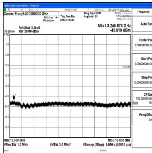
Band12_5MHz_QPSK_23095_1RB#0_3000~10000_3000~10000
