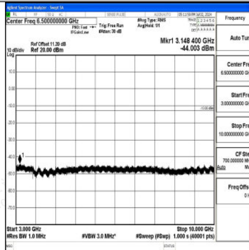
Band12_5MHz_QPSK_23155_1RB#0_3000~10000_3000~10000
