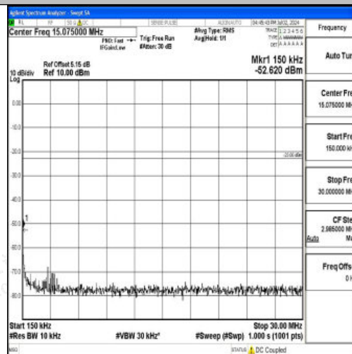
Band12_3MHz_QPSK_23165_1RB#0_0.15~30_0.15~30
