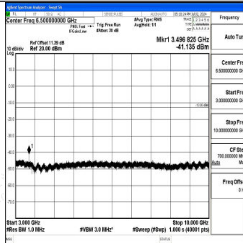
Band12_5MHz_16QAM_23035_1RB#0_3000~10000_3000~10000
