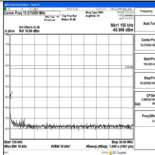
Band12_5MHz_QPSK_23155_1RB#0_0.15~30_0.15~30
