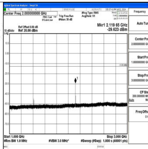
Band12_10MHz_QPSK_23130_1RB#0_1000~3000_1000~3000
