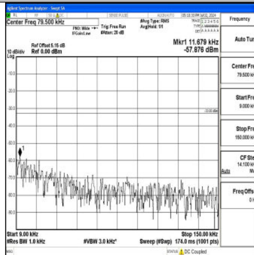
Band12_5MHz_QPSK_23095_1RB#0_0.009~0.15_0.009~0.15
