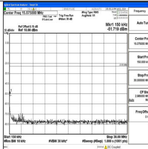
Band12_10MHz_QPSK_23060_1RB#0_0.15~30_0.15~30
