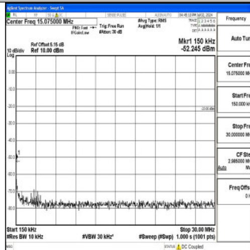
Band12_3MHz_16QAM_23095_1RB#0_0.15~30_0.15~30
