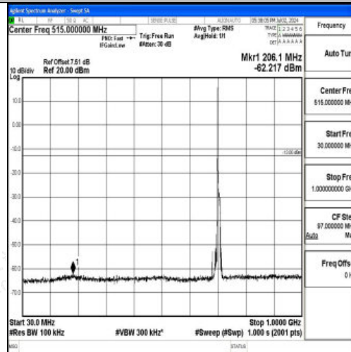
Band12_10MHz_16QAM_23130_1RB#0_30~1000_30~1000
