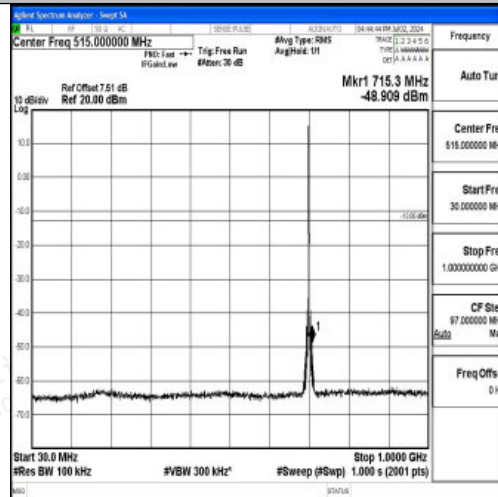
Band12_3MHz_QPSK_23095_1RB#0_30~1000_30~1000
