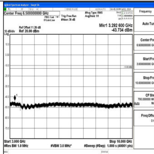
Band12_3MHz_16QAM_23095_1RB#0_3000~10000_3000~10000
