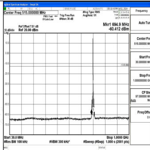
Band12_5MHz_QPSK_23095_1RB#0_30~1000_30~1000
