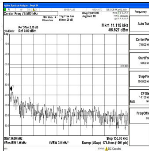
Band12_10MHz_QPSK_23130_1RB#0_0.009~0.15_0.009~0.15
