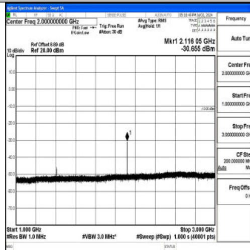
Band12_5MHz_QPSK_23095_1RB#0_1000~3000_1000~3000
