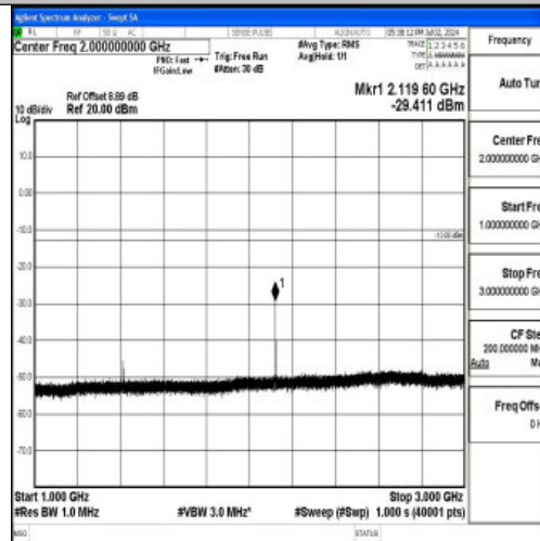
Band12_10MHz_16QAM_23130_1RB#0_1000~3000_1000~3000
