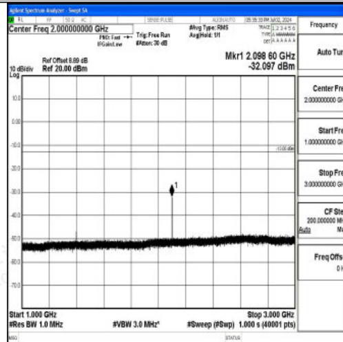
Band12_10MHz_QPSK_23060_1RB#0_1000~3000_1000~3000
