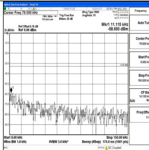
Band12_10MHz_QPSK_23060_1RB#0_0.009~0.15_0.009~0.15
