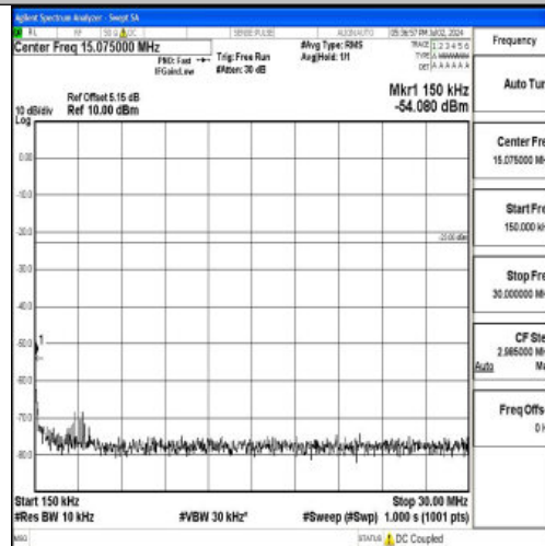
Band12_10MHz_16QAM_23095_1RB#0_0.15~30_0.15~30
