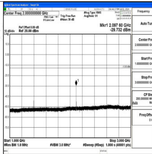
Band12_3MHz_16QAM_23025_1RB#0_1000~3000_1000~3000
