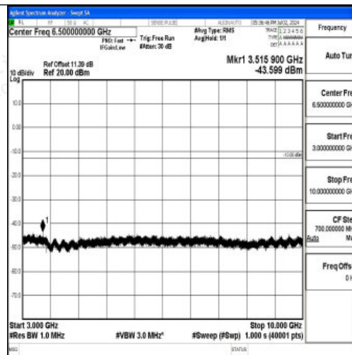
Band12_10MHz_QPSK_23095_1RB#0_3000~10000_3000~10000
