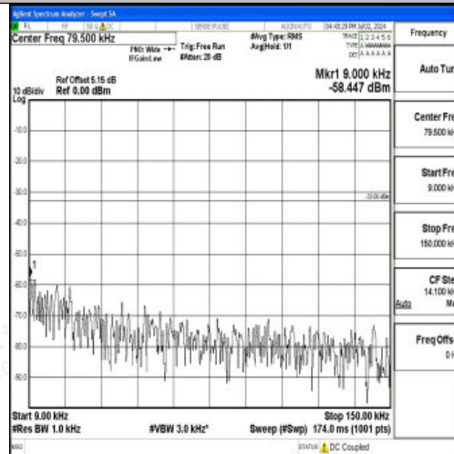
Band12_3MHz_QPSK_23025_1RB#0_0.009~0.15_0.009~0.15
