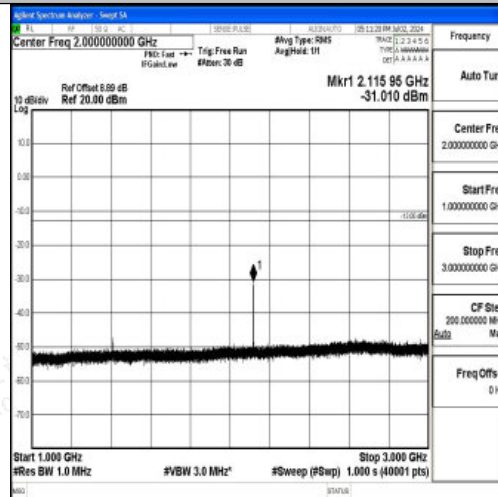
Band12_5MHz_16QAM_23095_1RB#0_1000~3000_1000~3000
