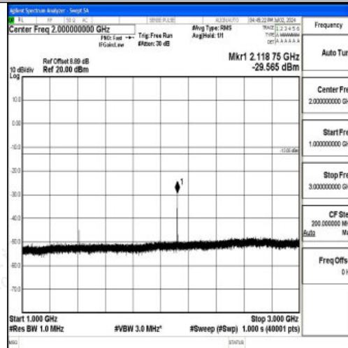
Band12_3MHz_16QAM_23095_1RB#0_1000~3000_1000~3000
