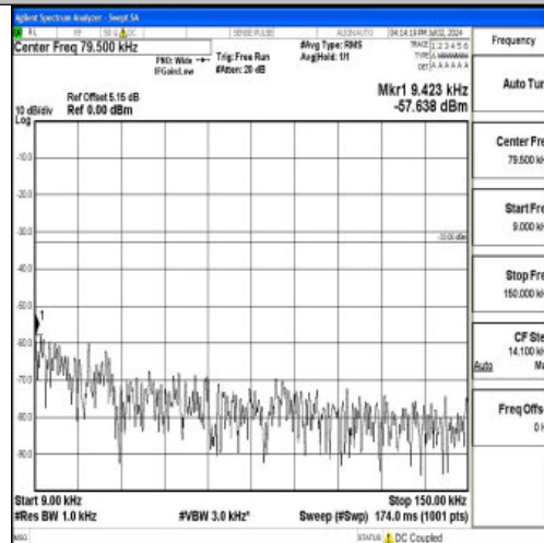
Band12_1.4MHz_16QAM_23173_1RB#0_0.009~0.15_0.009~0.15
