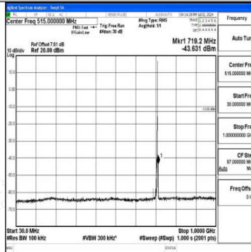
Band12_1.4MHz_16QAM_23173_1RB#0_30~1000_30~1000
