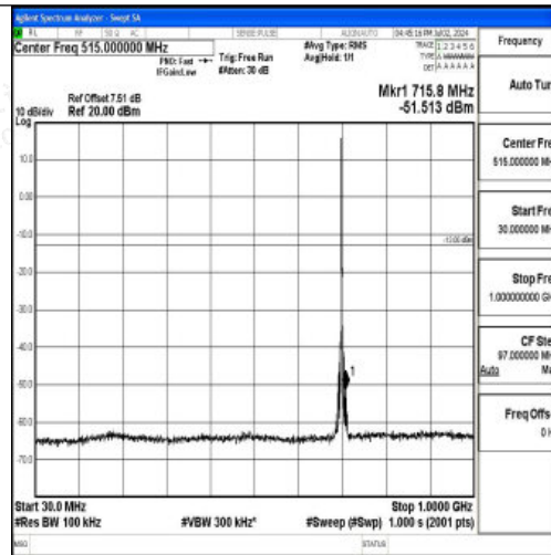
Band12_3MHz_16QAM_23095_1RB#0_30~1000_30~1000
