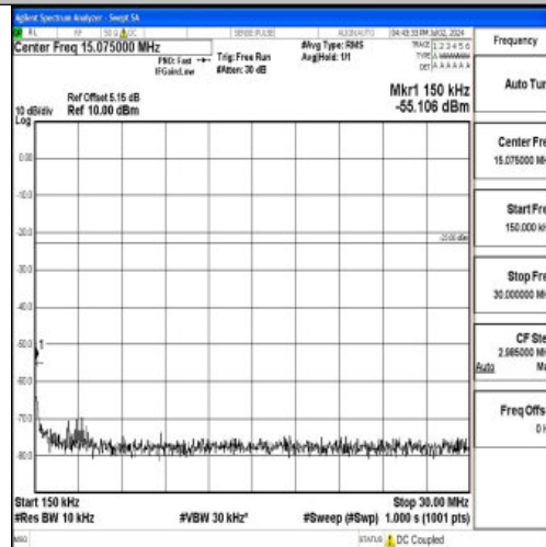
Band12_3MHz_QPSK_23025_1RB#0_0.15~30_0.15~30
