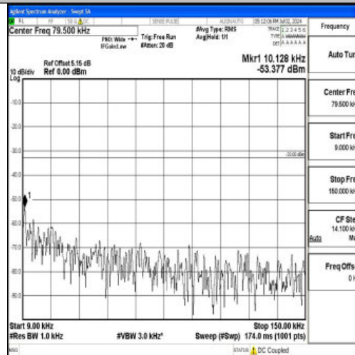
Band12_5MHz_16QAM_23155_1RB#0_0.009~0.15_0.009~0.15
