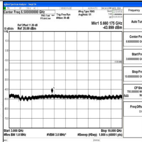
Band12_1.4MHz_QPSK_23173_1RB#0_3000~10000_3000~10000
