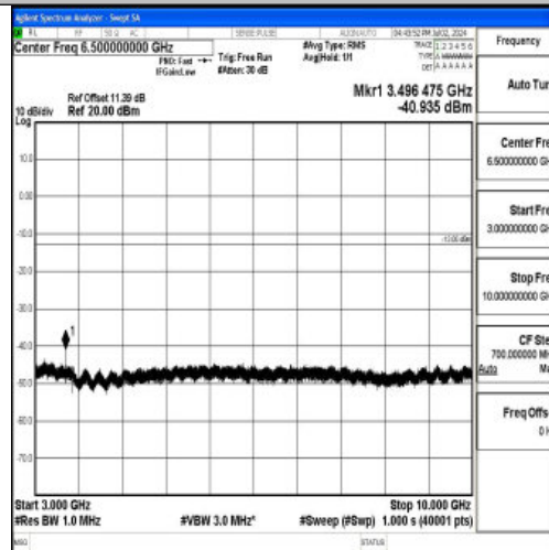
Band12_3MHz_QPSK_23025_1RB#0_3000~10000_3000~10000
