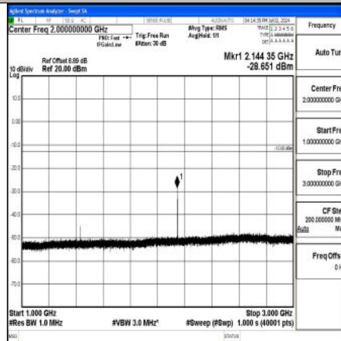
Band12_1.4MHz_16QAM_23173_1RB#0_1000~3000_1000~3000
