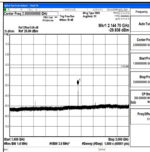
Band12_1.4MHz_QPSK_23173_1RB#0_1000~3000_1000~3000
