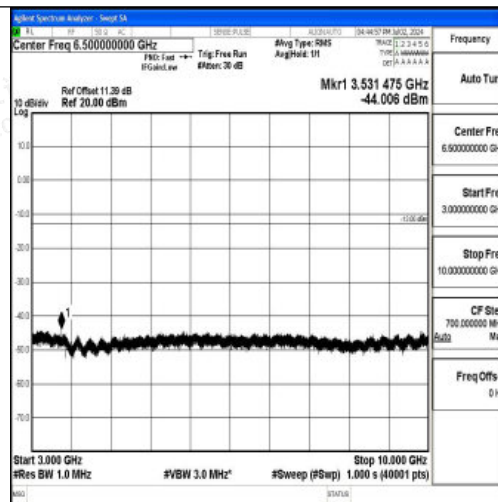
Band12_3MHz_QPSK_23095_1RB#0_3000~10000_3000~10000
