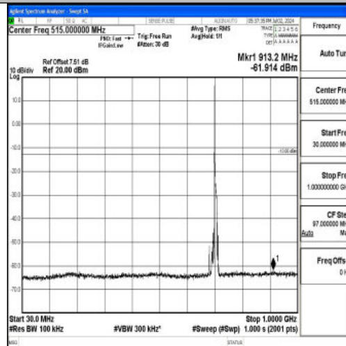
Band12_10MHz_QPSK_23130_1RB#0_30~1000_30~1000
