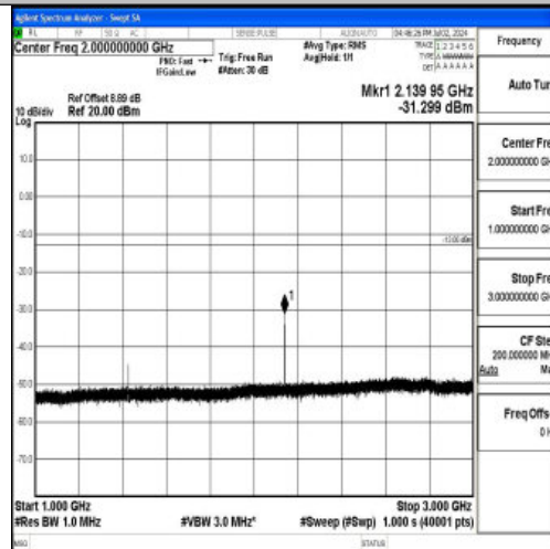
Band12_3MHz_16QAM_23165_1RB#0_1000~3000_1000~3000
