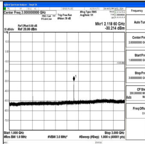
Band12_3MHz_QPSK_23095_1RB#0_1000~3000_1000~3000
