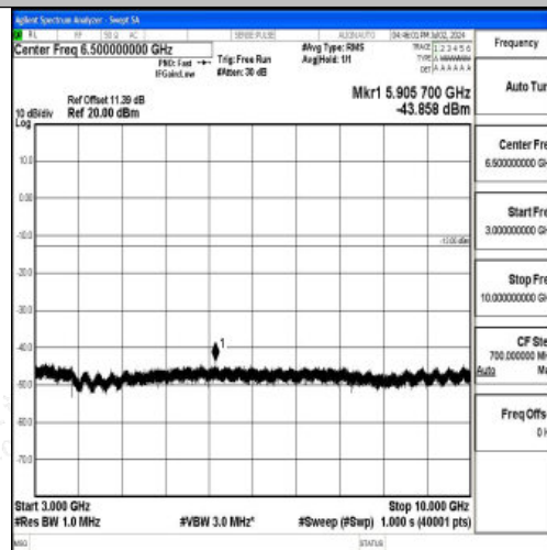
Band12_3MHz_QPSK_23165_1RB#0_3000~10000_3000~10000
