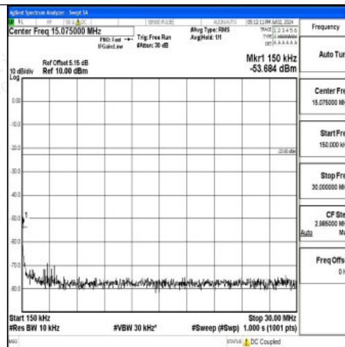
Band12_5MHz_16QAM_23155_1RB#0_0.15~30_0.15~30
