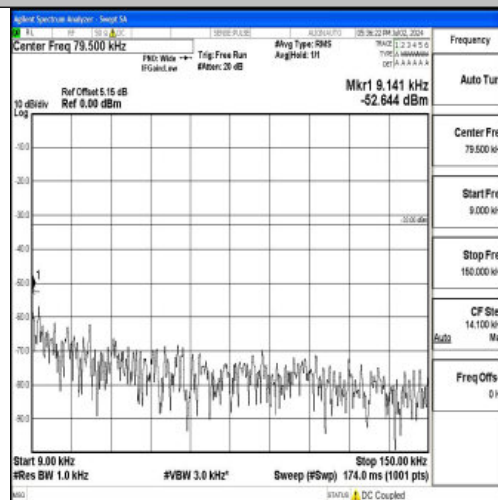
Band12_10MHz_QPSK_23095_1RB#0_0.009~0.15_0.009~0.15
