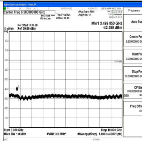
Band12_10MHz_QPSK_23060_1RB#0_3000~10000_3000~10000
