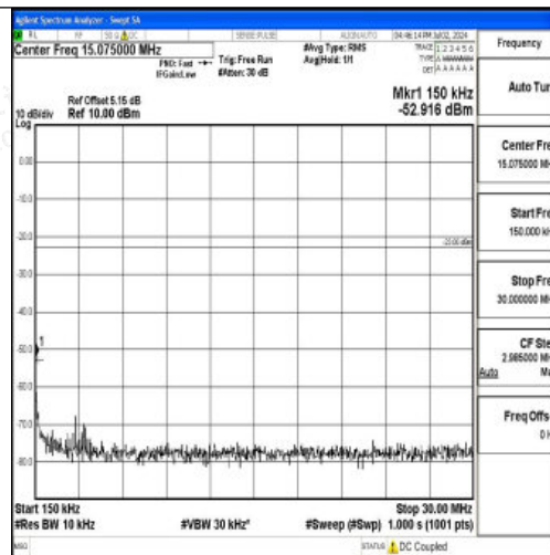
Band12_3MHz_16QAM_23165_1RB#0_0.15~30_0.15~30
