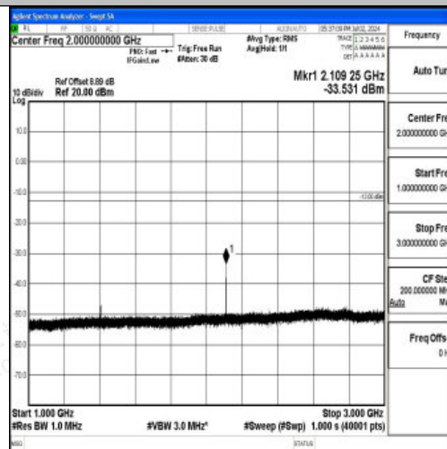
Band12_10MHz_16QAM_23095_1RB#0_1000~3000_1000~3000
