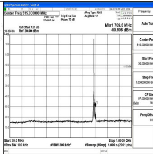
Band12_3MHz_QPSK_23025_1RB#0_30~1000_30~1000
