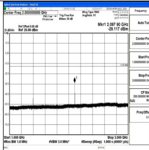
Band12_5MHz_QPSK_23035_1RB#0_1000~3000_1000~3000
