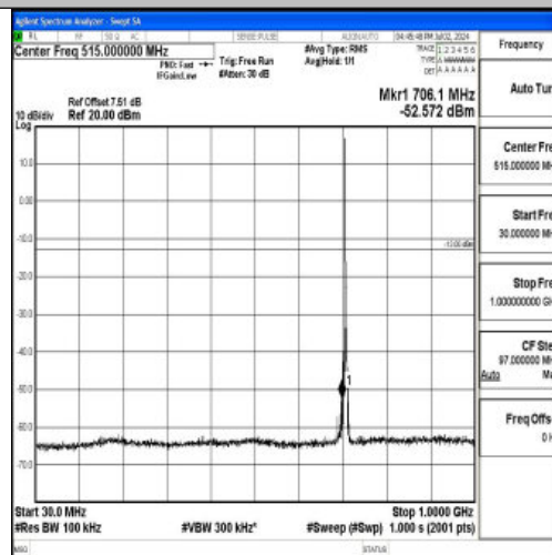
Band12_3MHz_QPSK_23165_1RB#0_30~1000_30~1000
