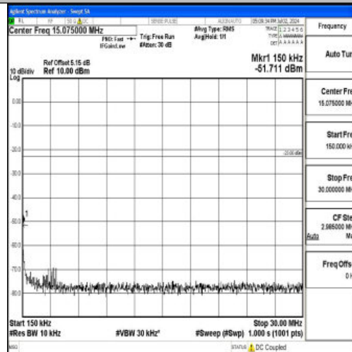
Band12_5MHz_QPSK_23035_1RB#0_0.15~30_0.15~30
