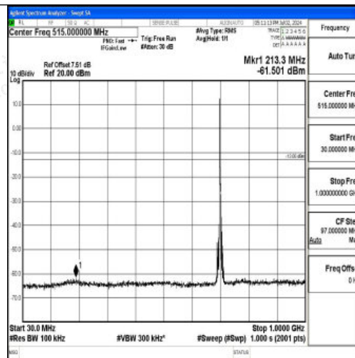
Band12_5MHz_16QAM_23095_1RB#0_30~1000_30~1000
