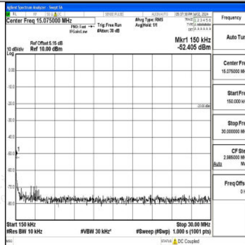
Band12_10MHz_QPSK_23130_1RB#0_0.15~30_0.15~30
