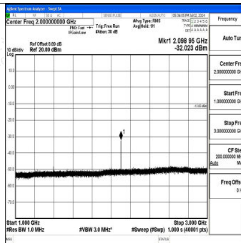
Band12_10MHz_16QAM_23060_1RB#0_1000~3000_1000~3000
