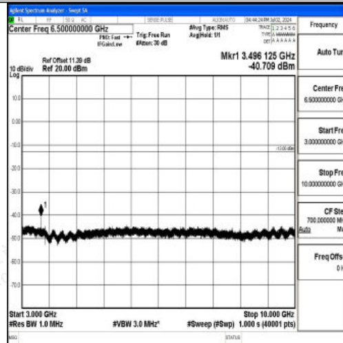
Band12_3MHz_16QAM_23025_1RB#0_3000~10000_3000~10000
