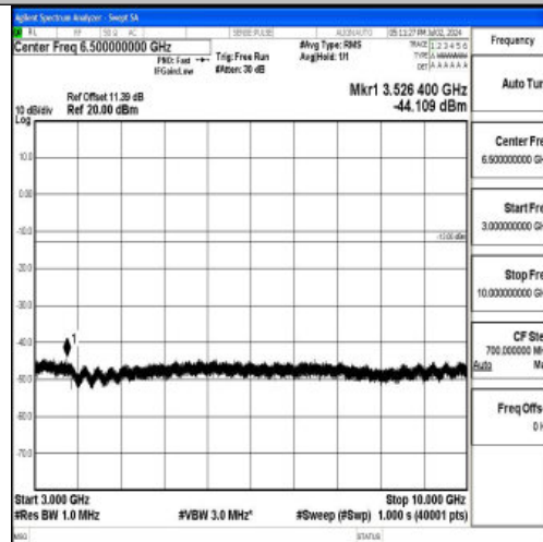
Band12_5MHz_16QAM_23095_1RB#0_3000~10000_3000~10000
