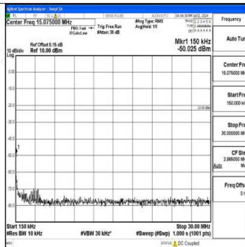
Band12_3MHz_QPSK_23095_1RB#0_0.15~30_0.15~30
