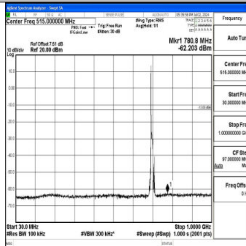
Band12_10MHz_16QAM_23060_1RB#0_30~1000_30~1000
