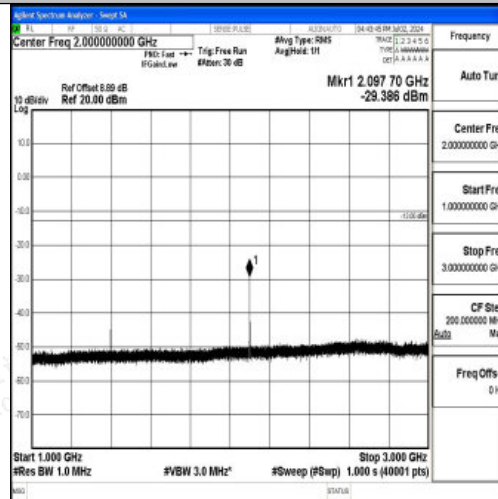
Band12_3MHz_QPSK_23025_1RB#0_1000~3000_1000~3000
