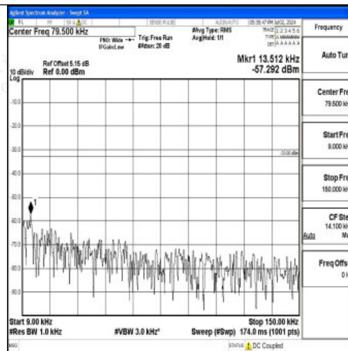
Band12_10MHz_16QAM_23060_1RB#0_0.009~0.15_0.009~0.15
