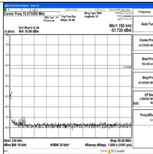
Band12_1.4MHz_16QAM_23173_1RB#0_0.15~30_0.15~30
