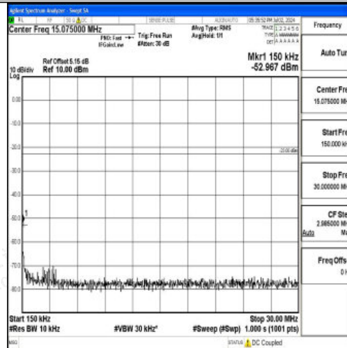
Band12_10MHz_16QAM_23060_1RB#0_0.15~30_0.15~30
