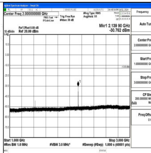
Band12_3MHz_QPSK_23165_1RB#0_1000~3000_1000~3000
