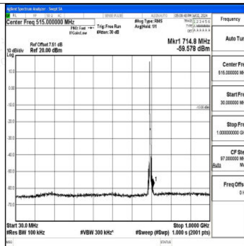
Band12_5MHz_QPSK_23035_1RB#0_30~1000_30~1000
