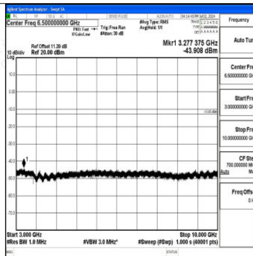
Band12_1.4MHz_16QAM_23173_1RB#0_3000~10000_3000~10000
