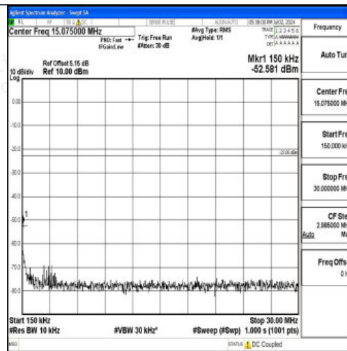
Band12_10MHz_16QAM_23130_1RB#0_0.15~30_0.15~30
