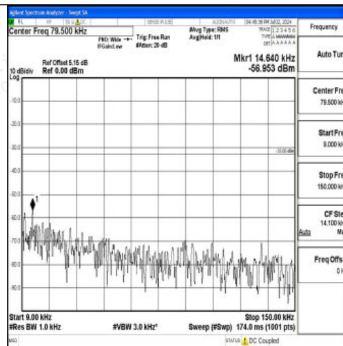
Band12_3MHz_QPSK_23165_1RB#0_0.009~0.15_0.009~0.15
