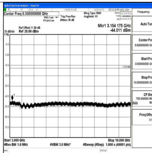
Band12_5MHz_16QAM_23155_1RB#0_3000~10000_3000~10000
