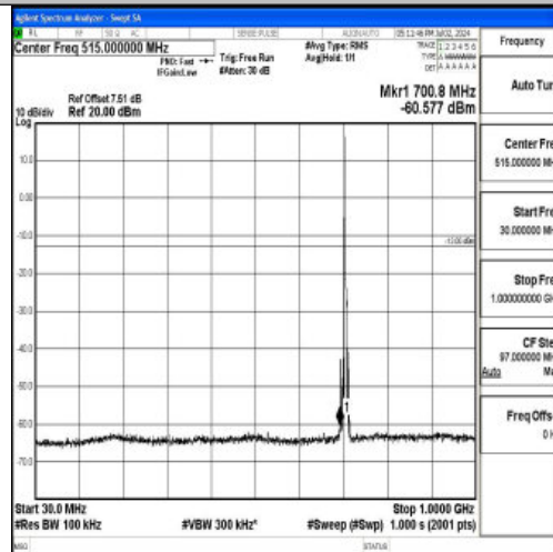
Band12_5MHz_QPSK_23155_1RB#0_30~1000_30~1000
