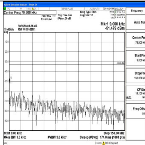
Band12_3MHz_QPSK_23095_1RB#0_0.009~0.15_0.009~0.15
