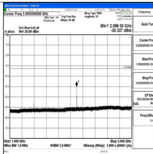
Band12_5MHz_16QAM_23035_1RB#0_1000~3000_1000~3000
