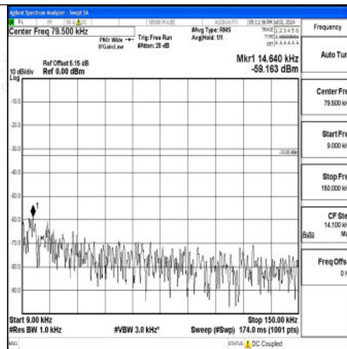
Band12_5MHz_QPSK_23155_1RB#0_0.009~0.15_0.009~0.15
