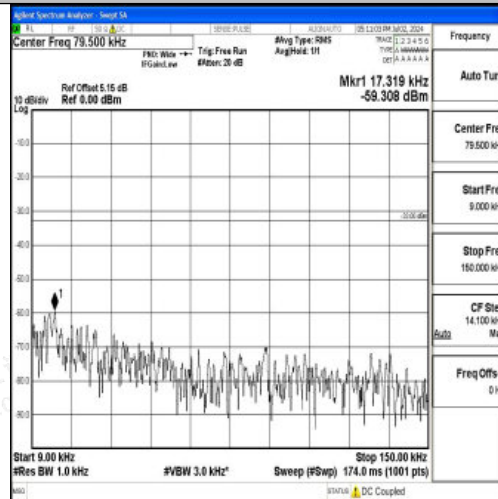
Band12_5MHz_16QAM_23095_1RB#0_0.009~0.15_0.009~0.15
