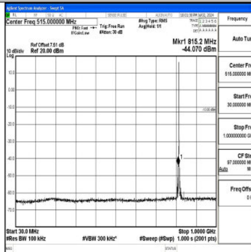
Band26_1.4MHz_16QAM_26740_1RB#0_30~1000_30~1000
