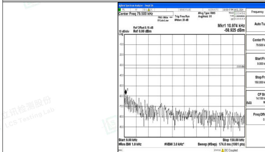
Band26_1.4MHz_QPSK_26740_1RB#0_0.009~0.15_0.009~0.15
