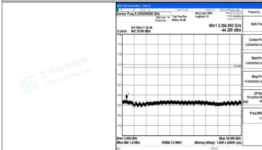
Band26_3MHz_QPSK_26740_1RB#0_3000~10000_3000~10000
