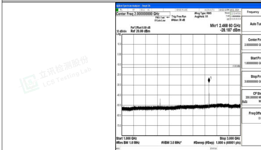
Band26_1.4MHz_QPSK_26783_1RB#0_1000~3000_1000~3000
