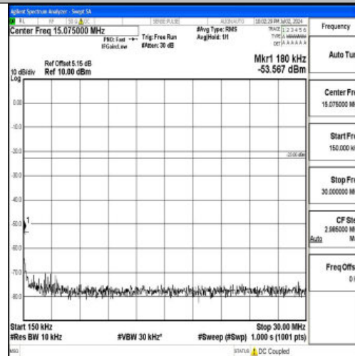
Band26_1.4MHz_16QAM_26783_1RB#0_0.15~30_0.15~30
