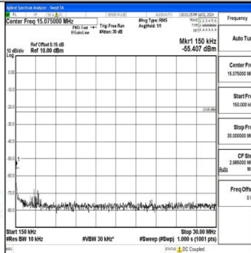
Band26_1.4MHz_16QAM_26740_1RB#0_0.15~30_0.15~30
