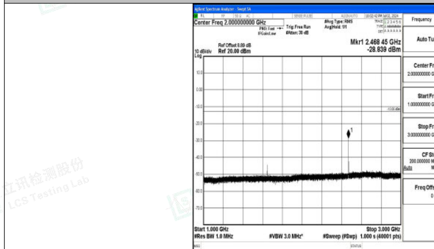
Band26_1.4MHz_16QAM_26783_1RB#0_1000~3000_1000~3000
