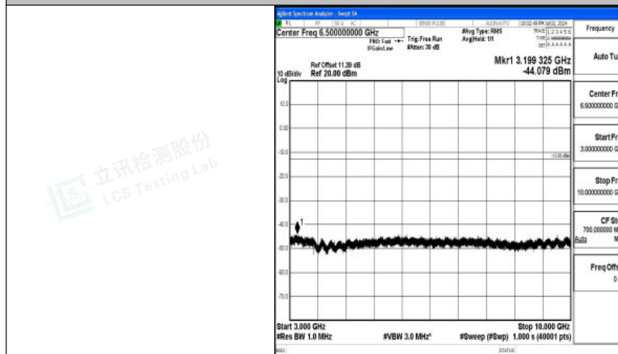
Band26_1.4MHz_16QAM_26783_1RB#0_3000~10000_3000~10000
