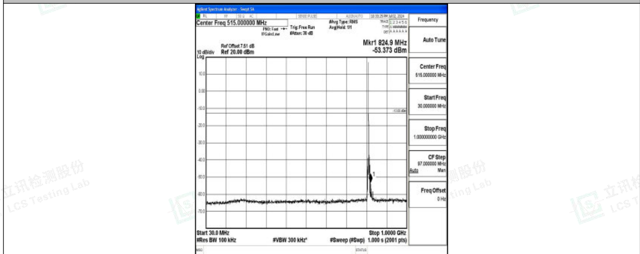
Band26_3MHz_16QAM_26705_1RB#0_30~1000_30~1000
