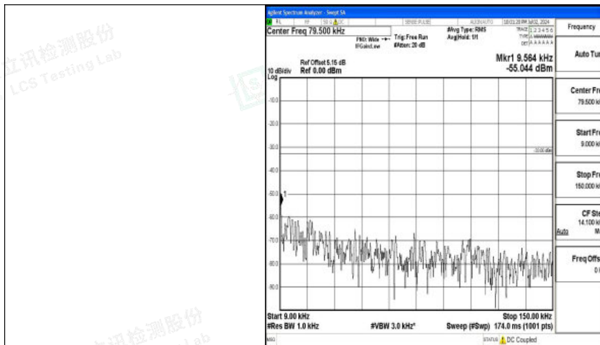
Band26_1.4MHz_16QAM_26740_1RB#0_0.009~0.15_0.009~0.15
