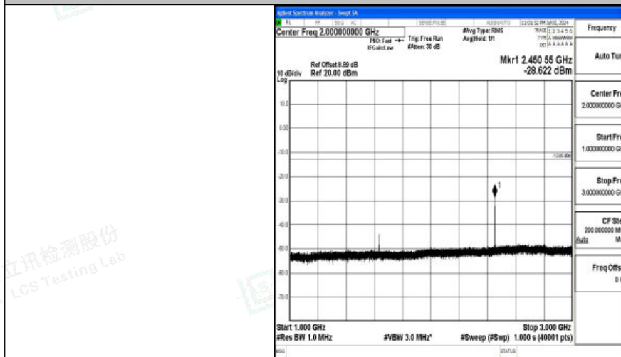
Band26_5MHz_QPSK_26740_1RB#0_1000~3000_1000~3000
