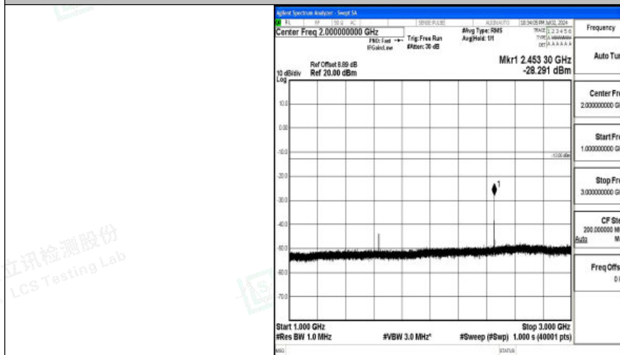
Band26_3MHz_QPSK_26740_1RB#0_1000~3000_1000~3000
