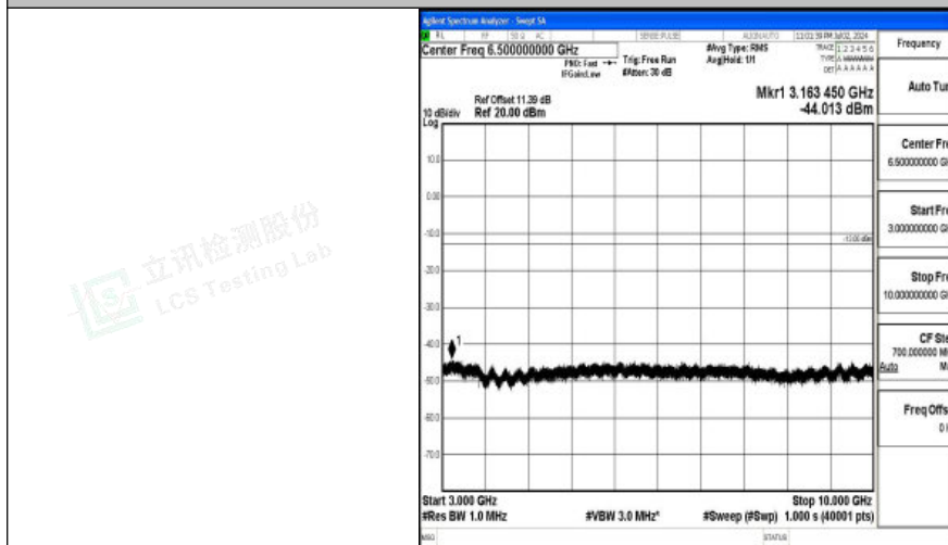
Band26_5MHz_QPSK_26740_1RB#0_3000~10000_3000~10000
