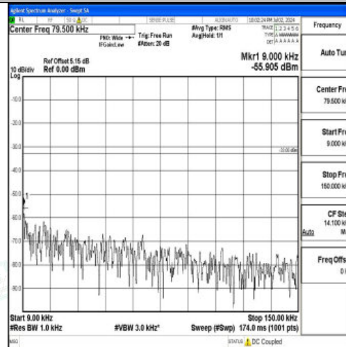
Band26_1.4MHz_16QAM_26783_1RB#0_0.009~0.15_0.009~0.15
