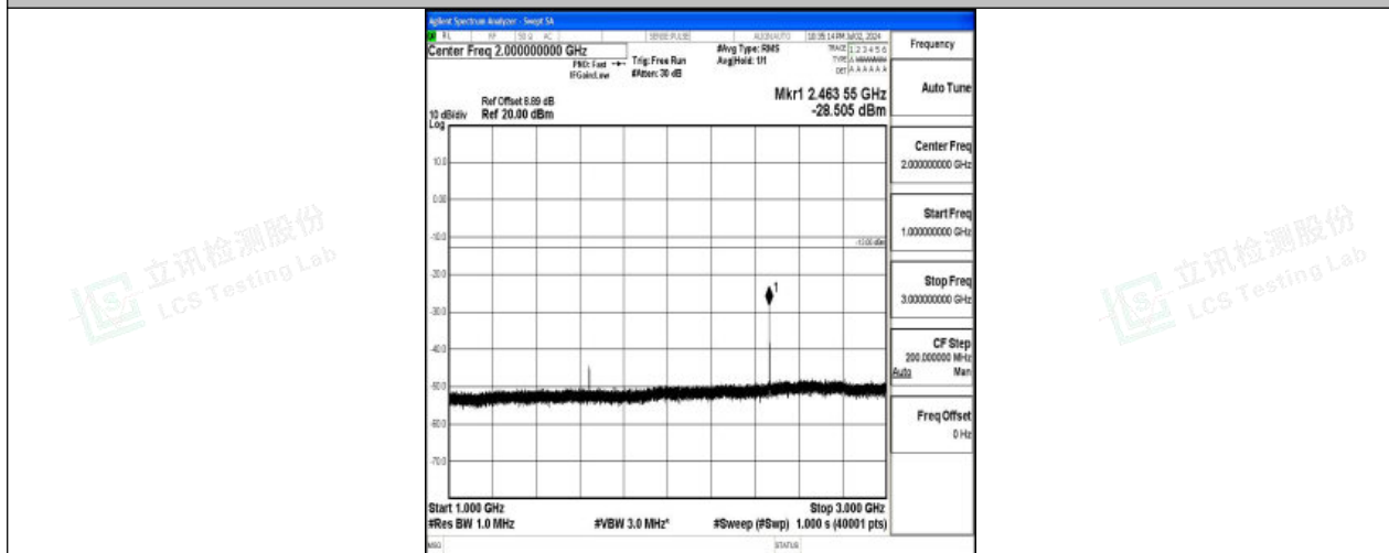
Band26_3MHz_QPSK_26775_1RB#0_1000~3000_1000~3000
