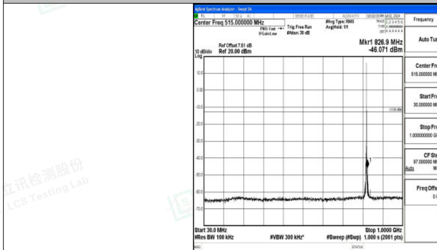
Band26_1.4MHz_QPSK_26783_1RB#0_30~1000_30~1000
