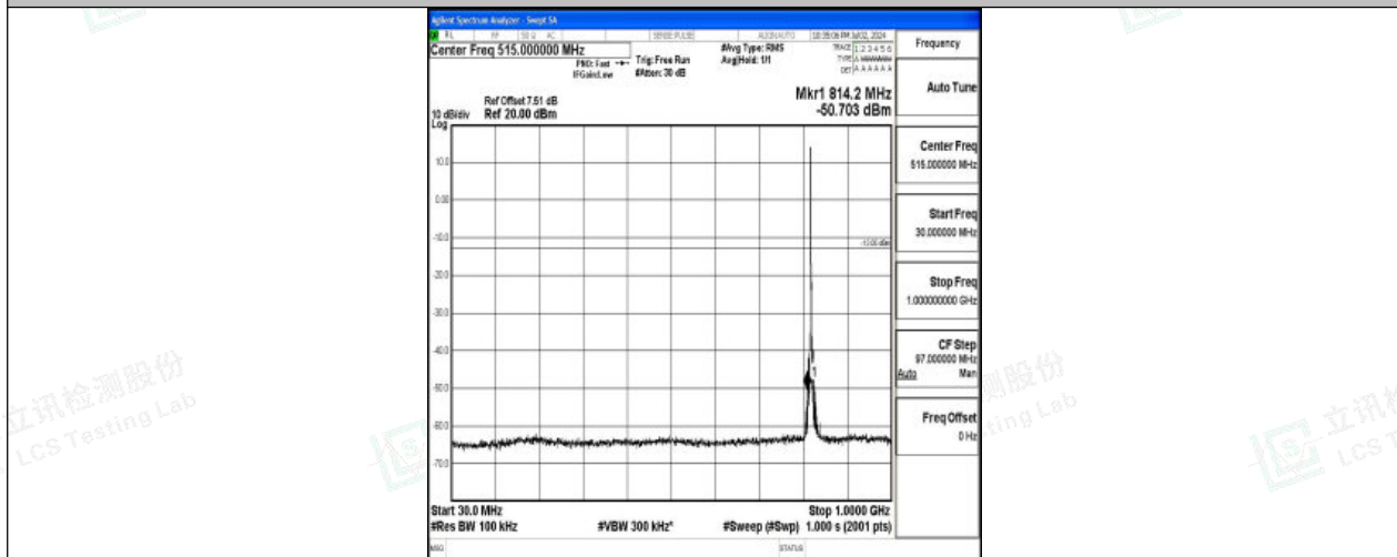
Band26_3MHz_QPSK_26775_1RB#0_30~1000_30~1000
