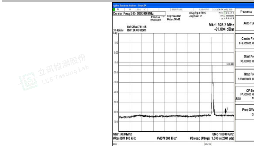
Band26_10MHz_QPSK_26740_1RB#0_30~1000_30~1000
