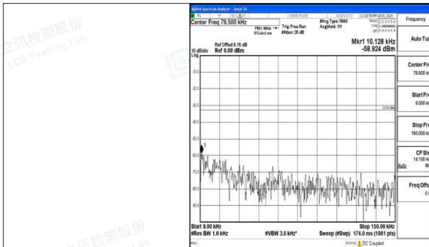
Band26_10MHz_QPSK_26740_1RB#0_0.009~0.15_0.009~0.15
