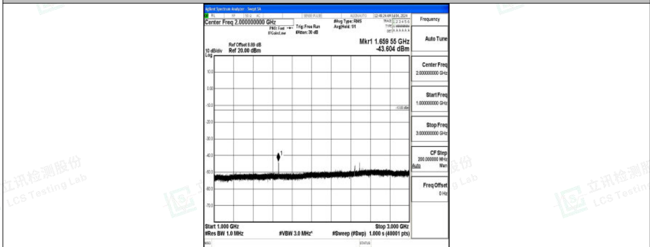
Band26_15MHz_QPSK_26915_1RB#0_1000~3000_1000~3000
