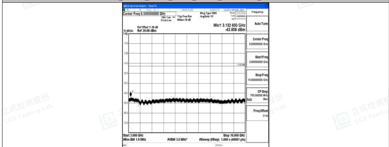
Band26_10MHz_QPSK_26840_1RB#0_3000~10000_3000~10000
