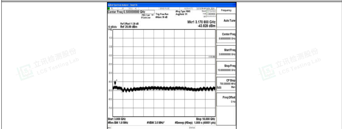
Band26_10MHz_16QAM_26990_1RB#0_3000~10000_3000~10000
