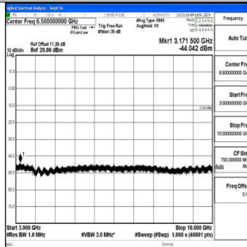
Band26_15MHz_16QAM_26965_1RB#0_3000~10000_3000~10000
