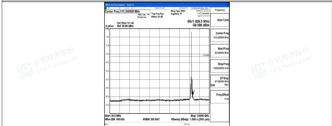
Band26_5MHz_QPSK_26815_1RB#0_30~1000_30~1000
