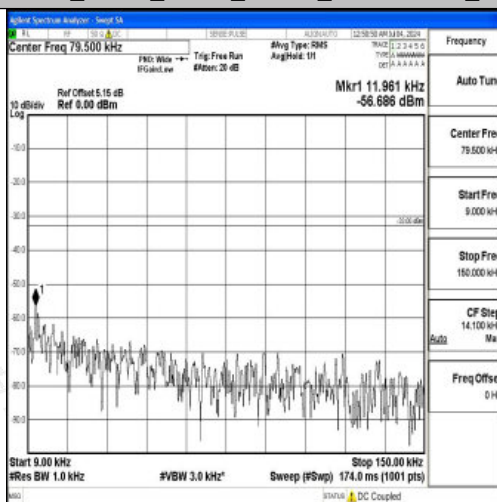
Band26_15MHz_16QAM_26965_1RB#0_0.009~0.15_0.009~0.15
