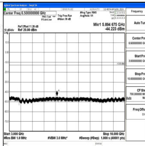
Band26_15MHz_16QAM_26865_1RB#0_3000~10000_3000~10000
