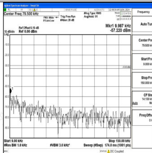
Band26_15MHz_QPSK_26915_1RB#0_0.009~0.15_0.009~0.15
