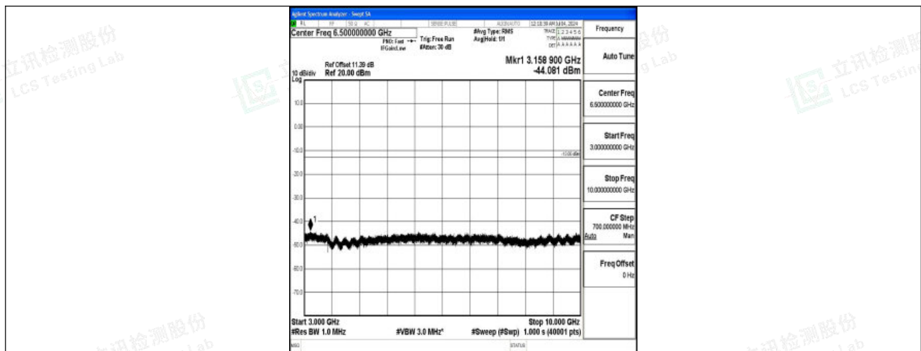
Band26_5MHz_QPSK_27015_1RB#0_3000~10000_3000~10000
