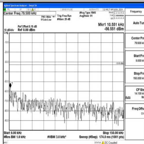
Band26_15MHz_16QAM_26865_1RB#0_0.009~0.15_0.009~0.15
