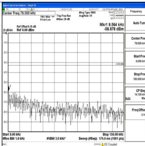
Band26_15MHz_QPSK_26865_1RB#0_0.009~0.15_0.009~0.15
