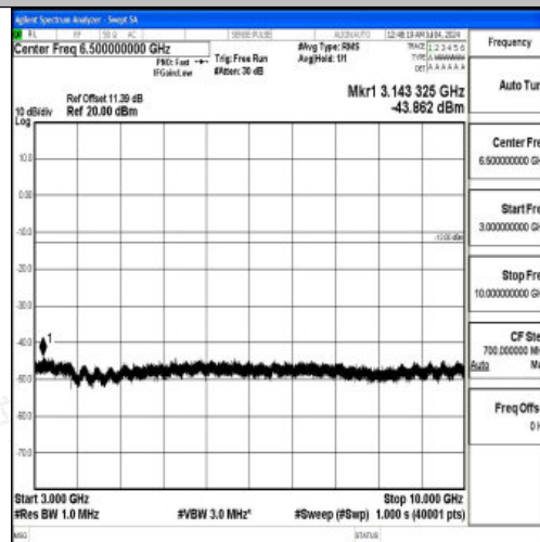
Band26_15MHz_QPSK_26865_1RB#0_3000~10000_3000~10000
