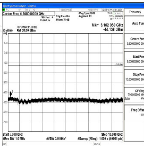
Band26_15MHz_QPSK_26965_1RB#0_3000~10000_3000~10000
