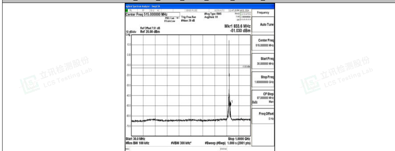
Band26_3MHz_QPSK_26805_1RB#0_30~1000_30~1000
