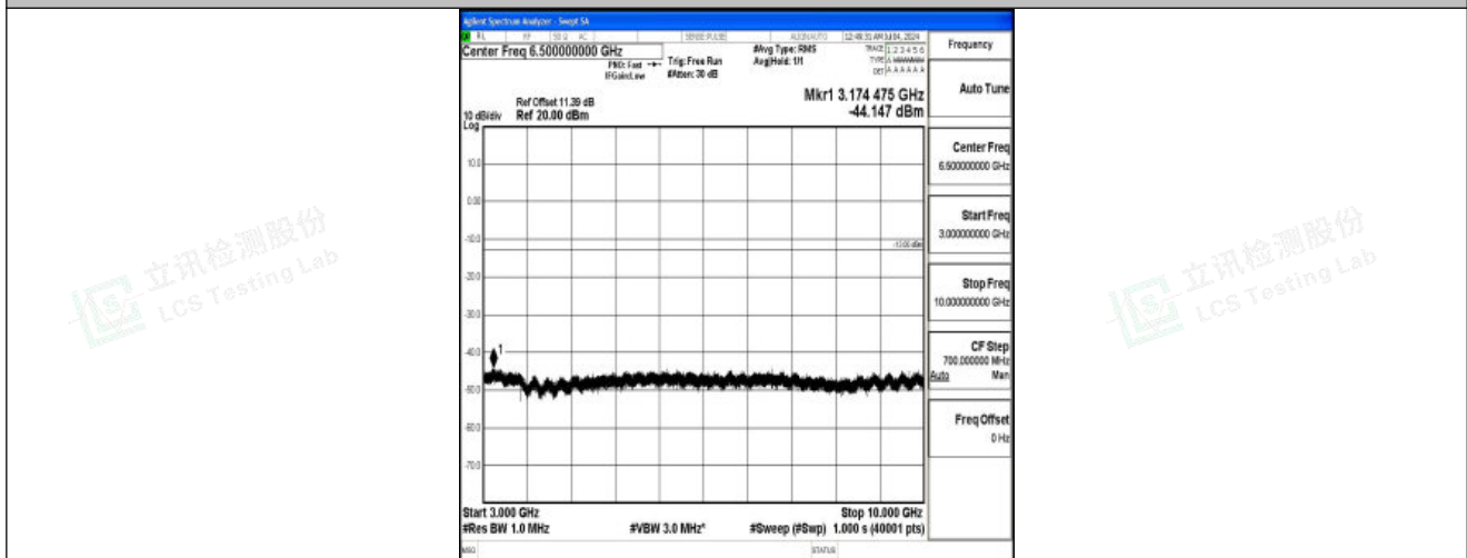
Band26_15MHz_QPSK_26915_1RB#0_3000~10000_3000~10000
