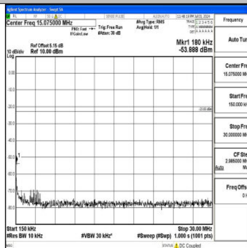
Band26_3MHz_QPSK_26915_1RB#0_0.15~30_0.15~30
