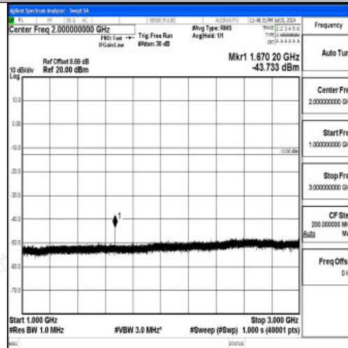
Band26_3MHz_QPSK_26915_1RB#0_1000~3000_1000~3000
