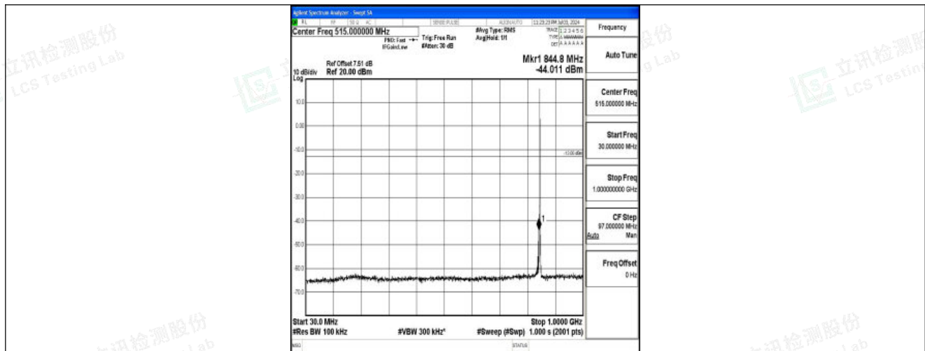
Band26_1.4MHz_16QAM_27033_1RB#0_30~1000_30~1000
