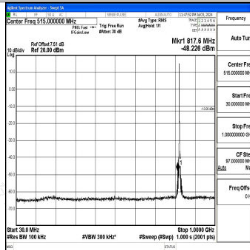
Band26_3MHz_16QAM_26805_1RB#0_30~1000_30~1000
