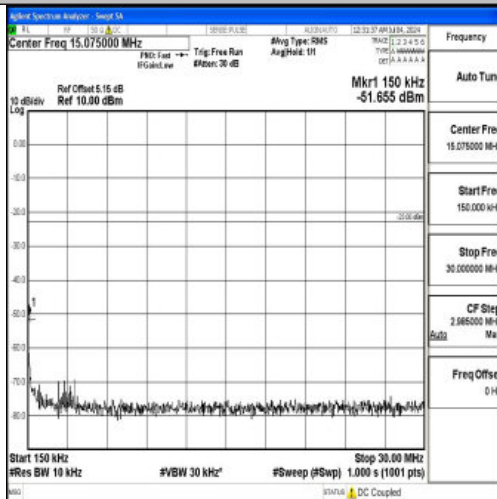
Band26_10MHz_16QAM_26990_1RB#0_0.15~30_0.15~30
