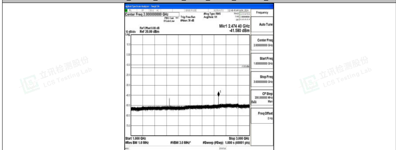
Band26_15MHz_16QAM_26865_1RB#0_1000~3000_1000~3000
