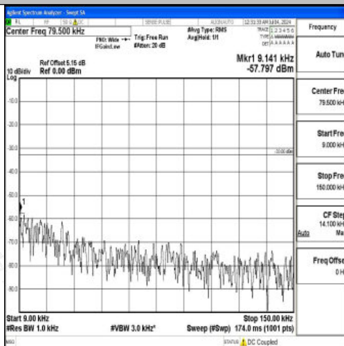
Band26_10MHz_16QAM_26990_1RB#0_0.009~0.15_0.009~0.15
