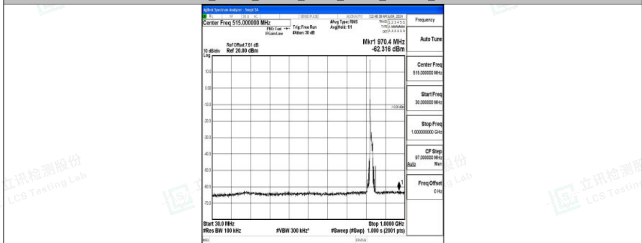
Band26_15MHz_16QAM_26865_1RB#0_30~1000_30~1000
