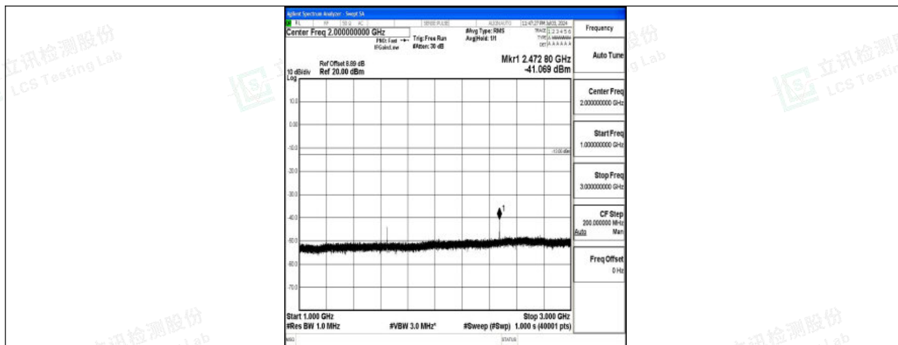
Band26_3MHz_QPSK_26805_1RB#0_1000~3000_1000~3000
