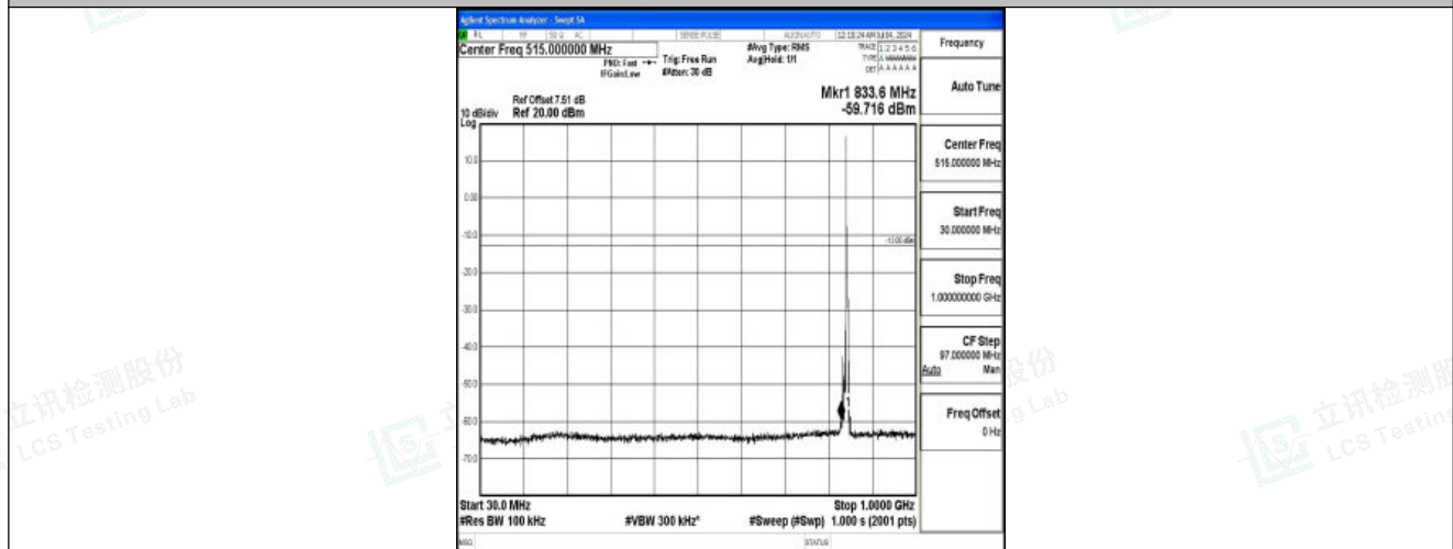
Band26_5MHz_QPSK_27015_1RB#0_30~1000_30~1000
