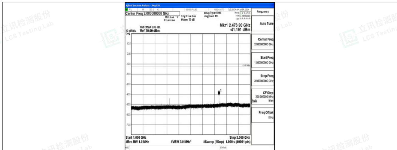
Band26_10MHz_QPSK_26840_1RB#0_1000~3000_1000~3000
