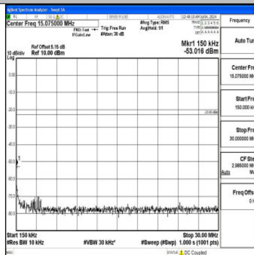
Band26_15MHz_QPSK_26915_1RB#0_0.15~30_0.15~30
