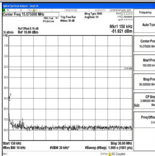
Band26_15MHz_16QAM_26965_1RB#0_0.15~30_0.15~30
