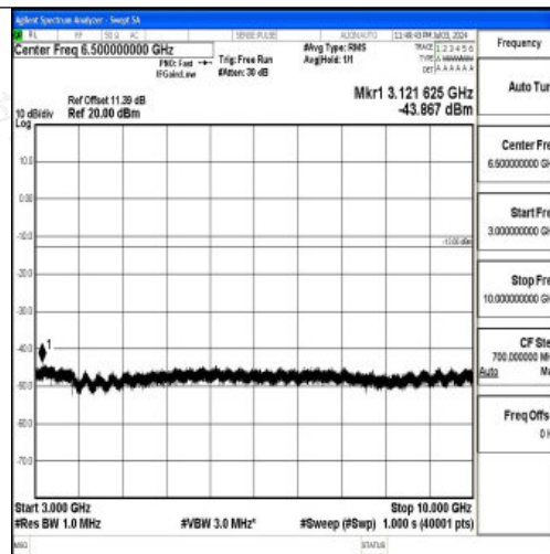
Band26_3MHz_QPSK_27025_1RB#0_3000~10000_3000~10000
