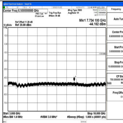
Band26_3MHz_QPSK_26915_1RB#0_3000~10000_3000~10000
