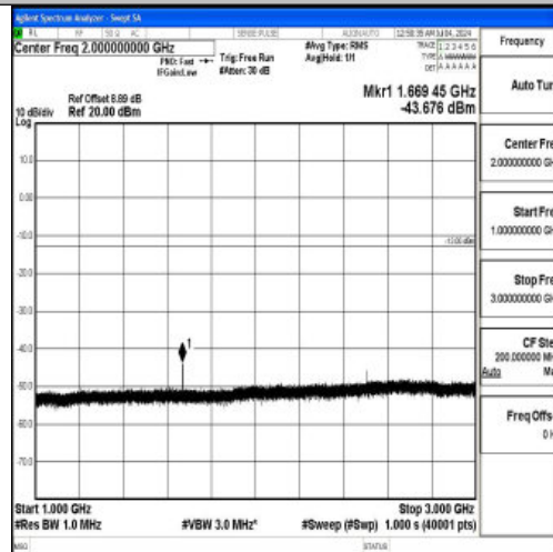
Band26_15MHz_QPSK_26965_1RB#0_1000~3000_1000~3000
