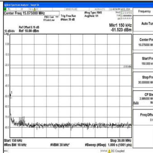
Band26_3MHz_16QAM_27025_1RB#0_0.15~30_0.15~30
