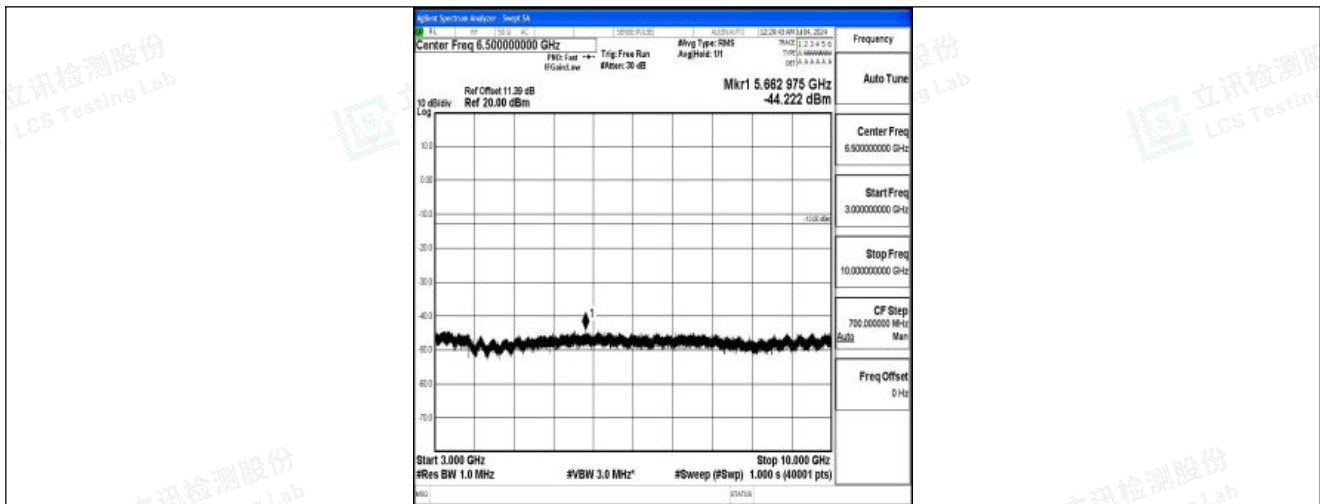
Band26_10MHz_16QAM_26840_1RB#0_3000~10000_3000~10000
