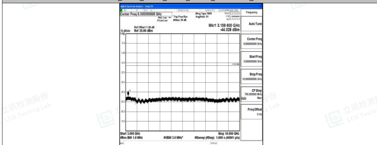
Band26_3MHz_QPSK_26805_1RB#0_3000~10000_3000~10000
