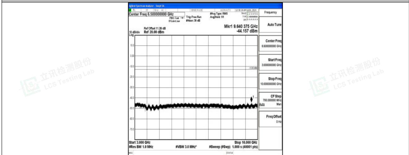
Band26_10MHz_QPSK_26915_1RB#0_3000~10000_3000~10000
