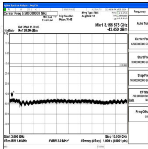
Band26_3MHz_16QAM_26805_1RB#0_3000~10000_3000~10000
