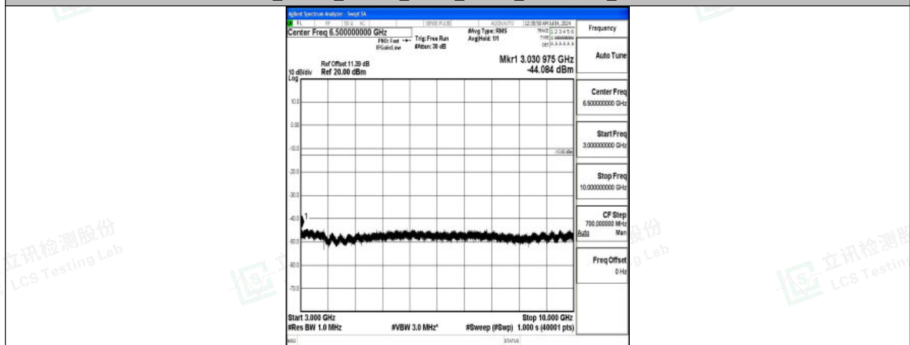
Band26_10MHz_16QAM_26915_1RB#0_3000~10000_3000~10000
