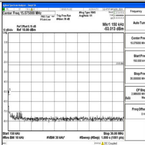
Band26_15MHz_QPSK_26865_1RB#0_0.15~30_0.15~30
