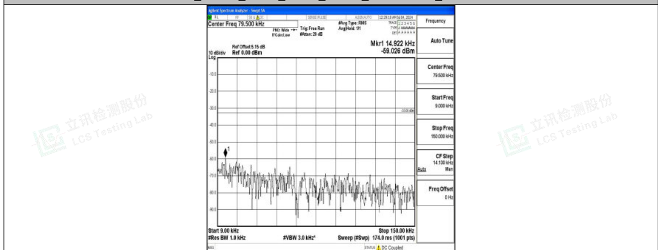
Band26_10MHz_16QAM_26840_1RB#0_0.009~0.15_0.009~0.15
