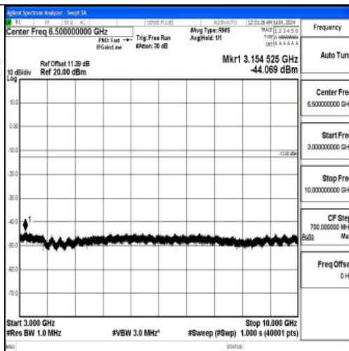
Band26_10MHz_QPSK_26990_1RB#0_3000~10000_3000~10000
