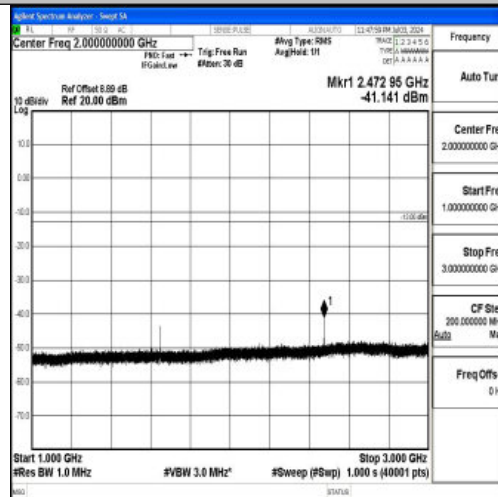
Band26_3MHz_16QAM_26805_1RB#0_1000~3000_1000~3000
