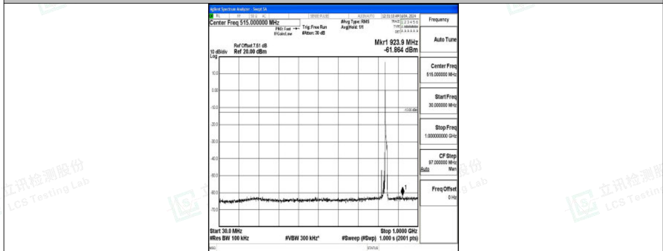
Band26_10MHz_QPSK_26990_1RB#0_30~1000_30~1000
