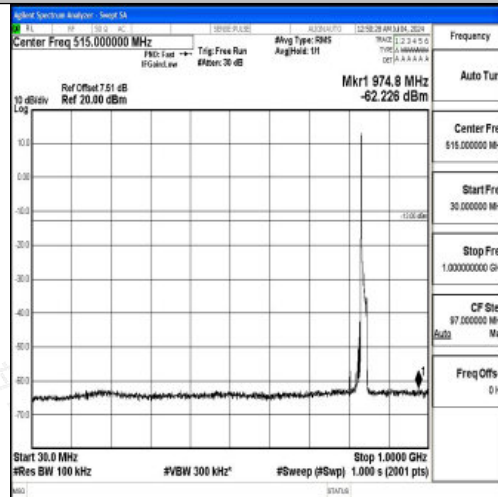
Band26_15MHz_QPSK_26965_1RB#0_30~1000_30~1000
