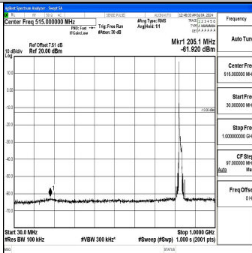
Band26_15MHz_QPSK_26865_1RB#0_30~1000_30~1000
