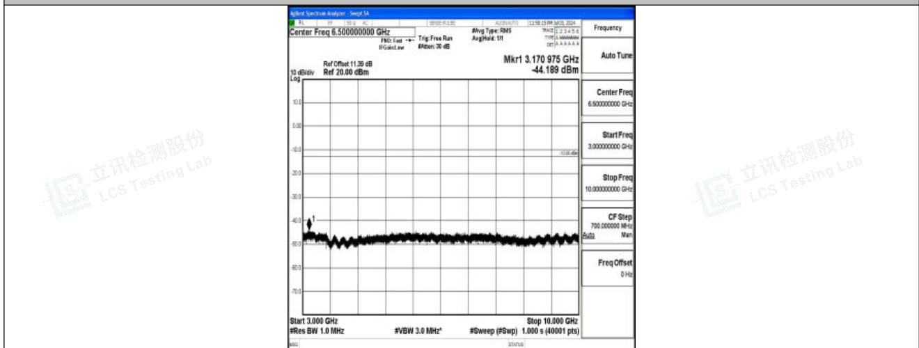
Band26_3MHz_16QAM_27025_1RB#0_3000~10000_3000~10000
