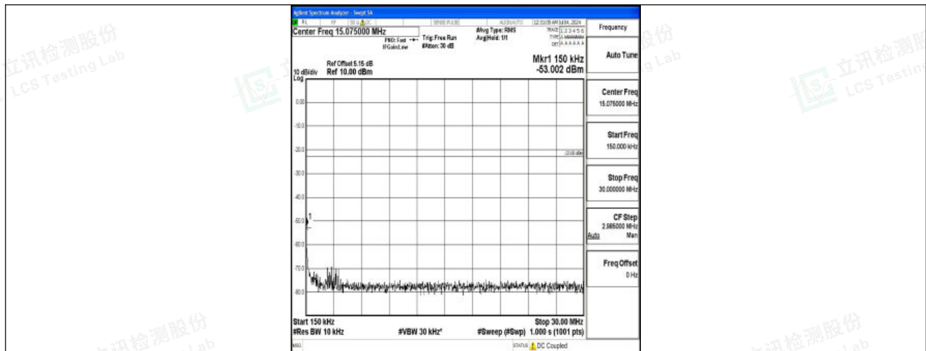
Band26_10MHz_QPSK_26990_1RB#0_0.15~30_0.15~30
