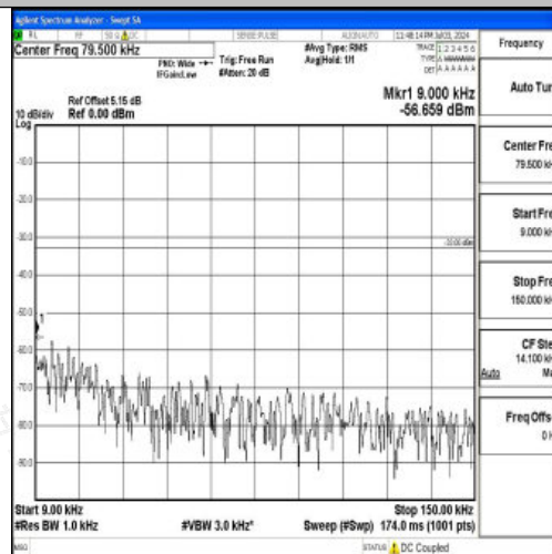
Band26_3MHz_QPSK_26915_1RB#0_0.009~0.15_0.009~0.15
