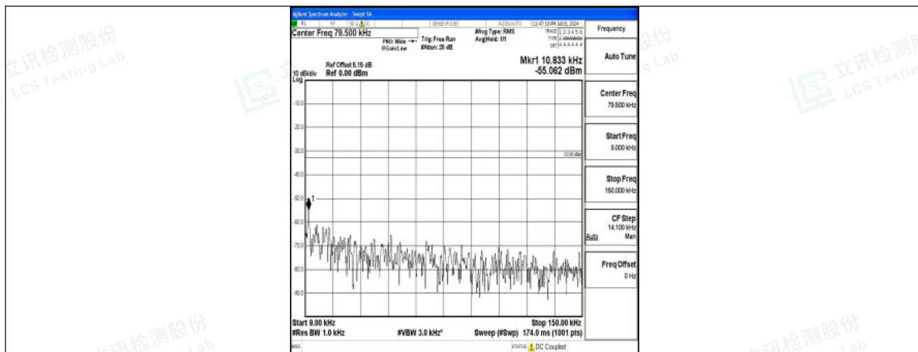
Band26_3MHz_QPSK_26805_1RB#0_0.009~0.15_0.009~0.15
