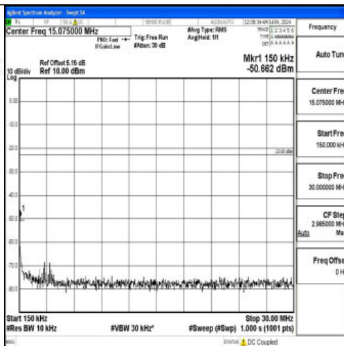
Band26_5MHz_16QAM_26815_1RB#0_0.15~30_0.15~30
