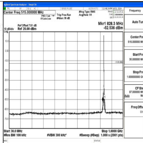
Band26_3MHz_QPSK_26915_1RB#0_30~1000_30~1000
