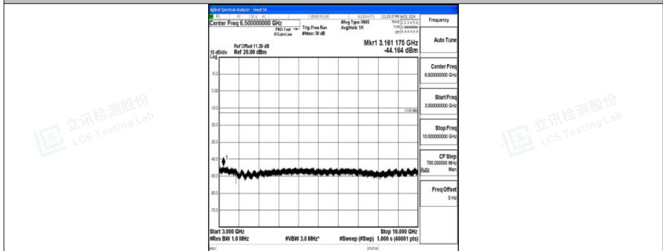
Band26_1.4MHz_16QAM_27033_1RB#0_3000~10000_3000~10000
