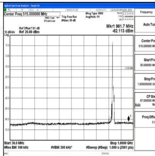
Band26_15MHz_16QAM_26965_1RB#0_30~1000_30~1000
