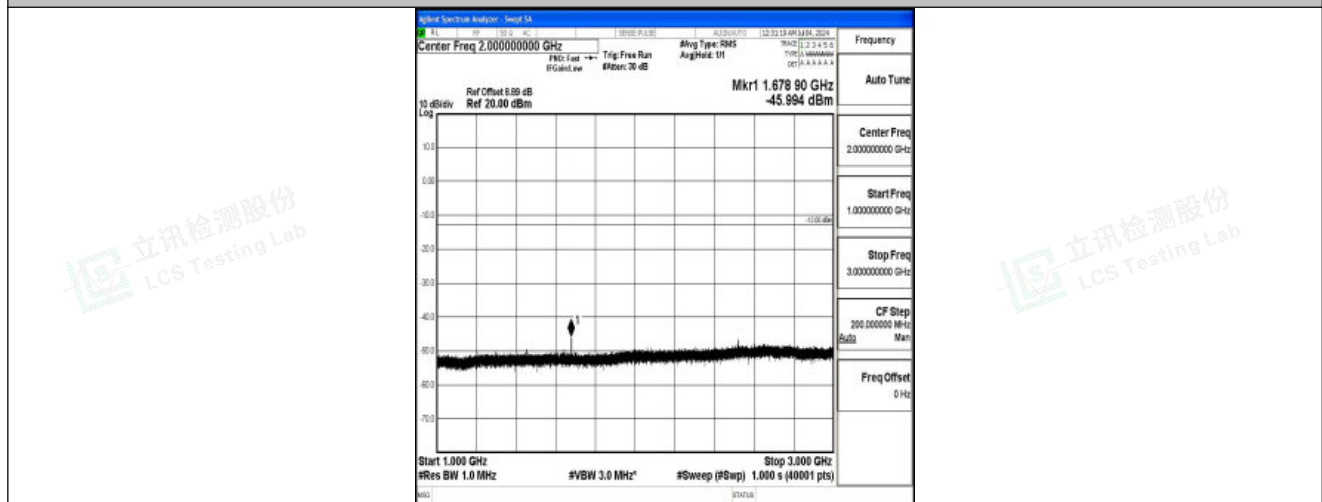
Band26_10MHz_QPSK_26990_1RB#0_1000~3000_1000~3000
