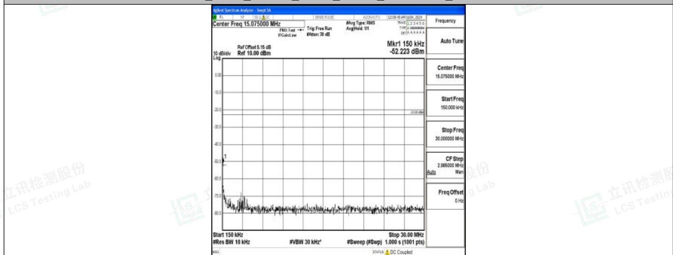
Band26_5MHz_16QAM_26915_1RB#0_0.15~30_0.15~30
