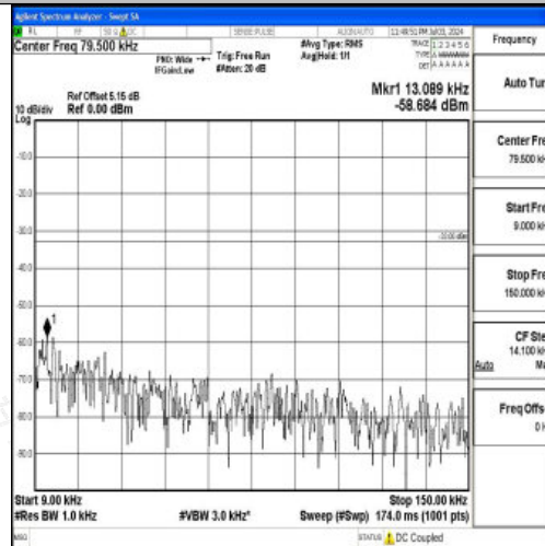
Band26_3MHz_16QAM_27025_1RB#0_0.009~0.15_0.009~0.15
