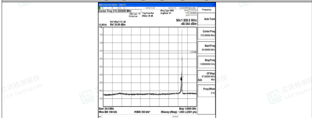
Band26_3MHz_QPSK_27025_1RB#0_30~1000_30~1000
