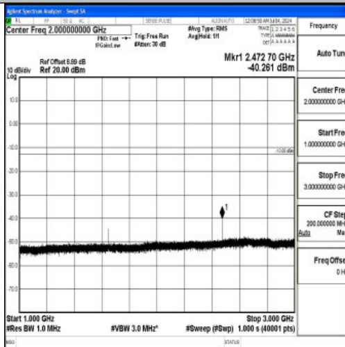
Band26_5MHz_16QAM_26815_1RB#0_1000~3000_1000~3000
