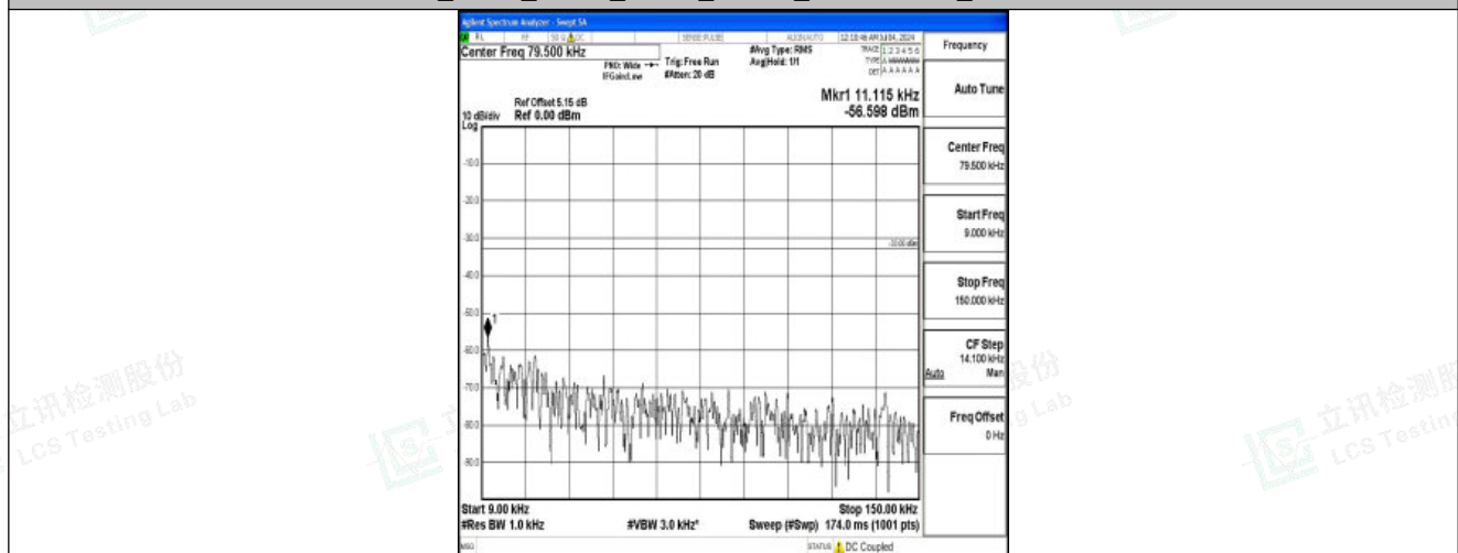
Band26_5MHz_16QAM_27015_1RB#0_0.009~0.15_0.009~0.15
