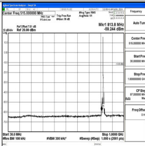
Band26_5MHz_16QAM_26815_1RB#0_30~1000_30~1000
