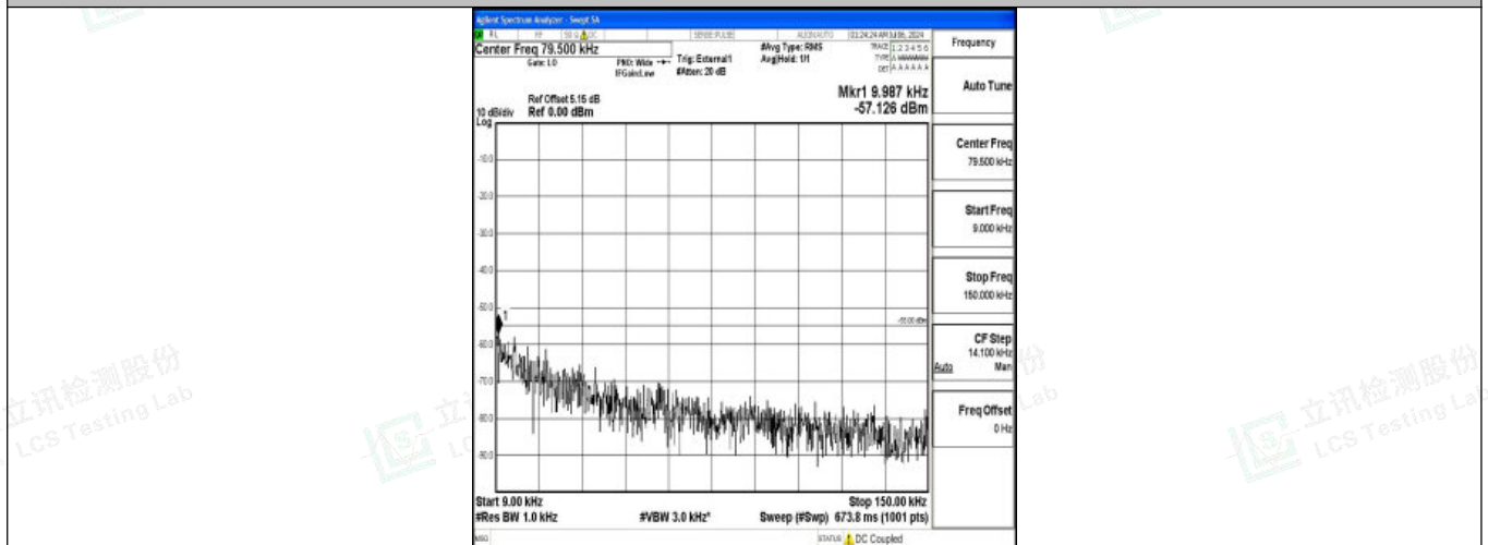
Band38_15MHz_QPSK_37825_1RB#0_0.009~0.15_0.009~0.15
