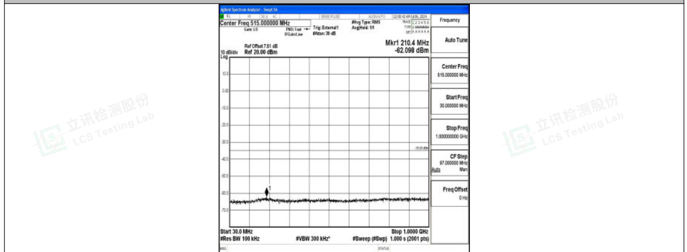
Band38_10MHz_QPSK_38200_1RB#0_30~1000_30~1000
