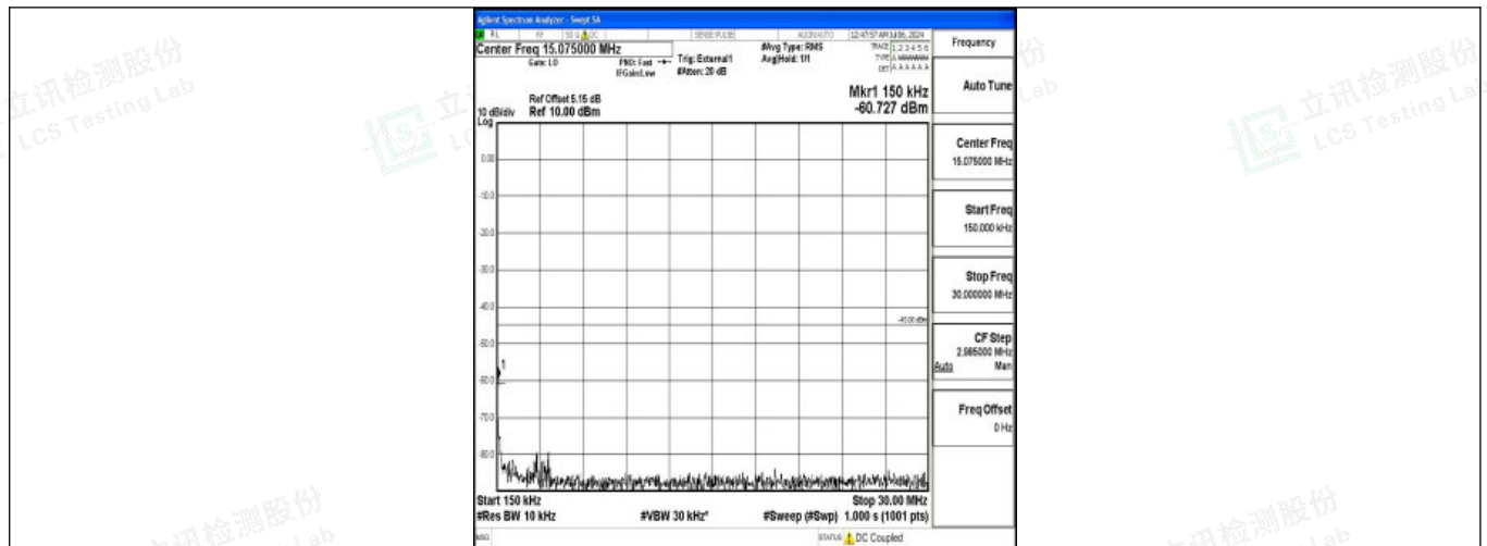
Band38_20MHz_16QAM_38150_1RB#0_0.15~30_0.15~30
