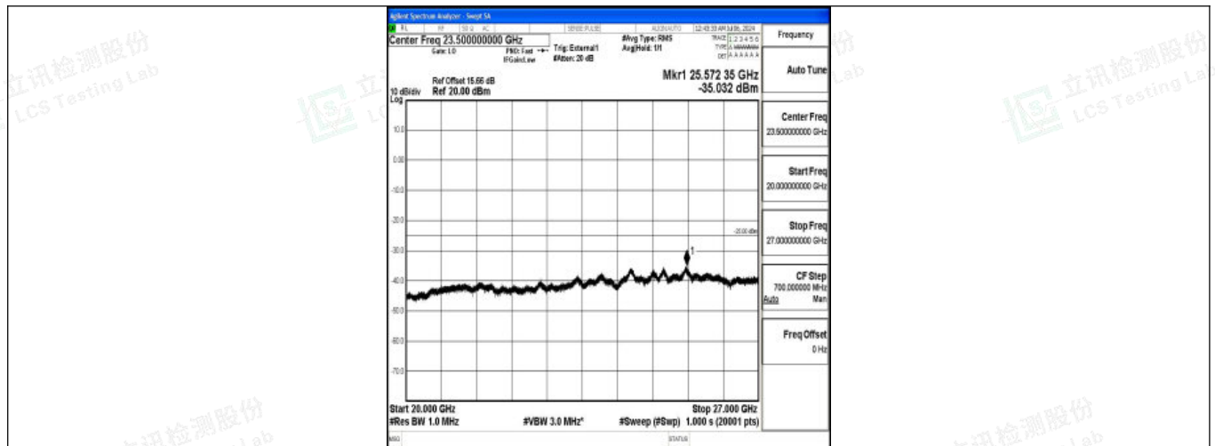
Band38_20MHz_QPSK_38000_1RB#0_20000~27000_20000~27000
