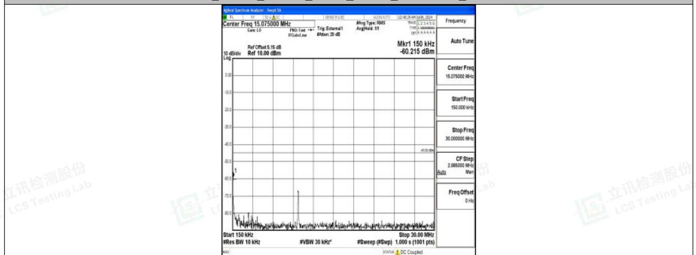
Band38_20MHz_16QAM_37850_1RB#0_0.15~30_0.15~30
