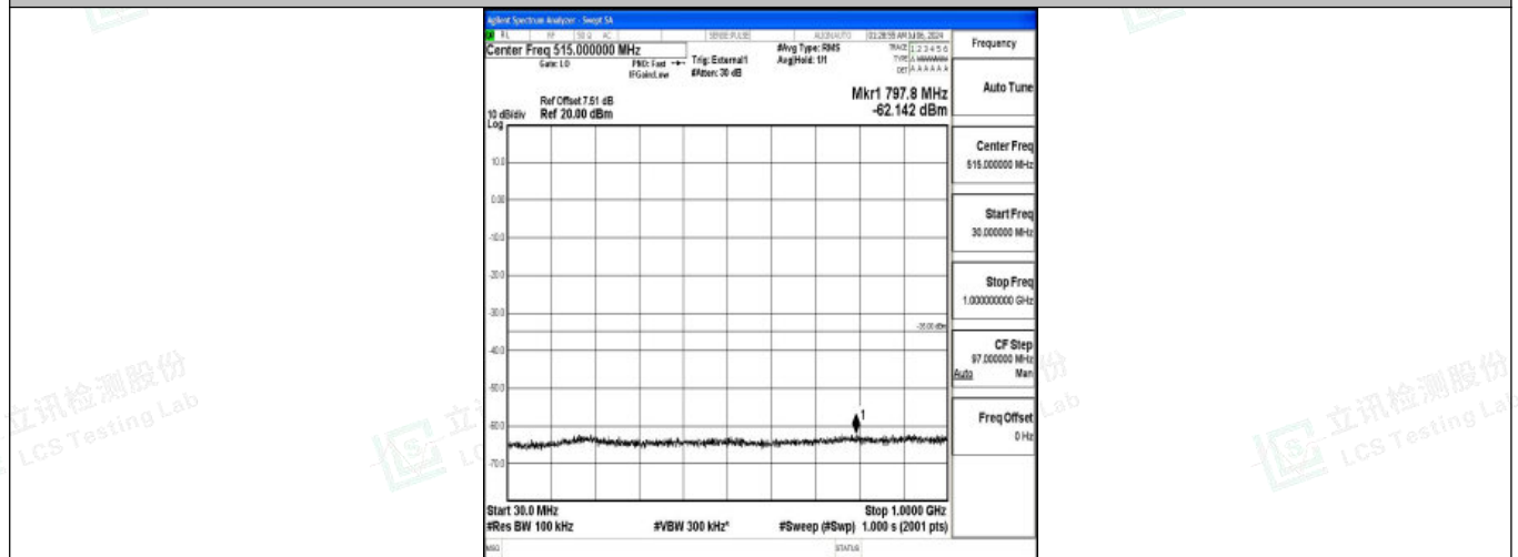
Band38_15MHz_QPSK_38000_1RB#0_30~1000_30~1000
