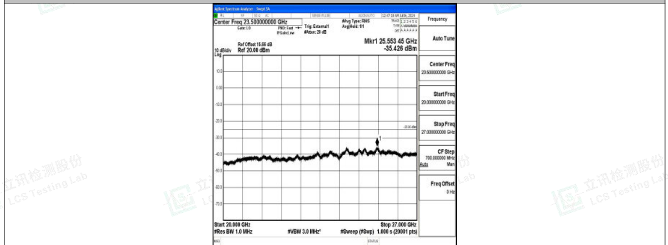
Band38_20MHz_QPSK_38150_1RB#0_20000~27000_20000~27000
