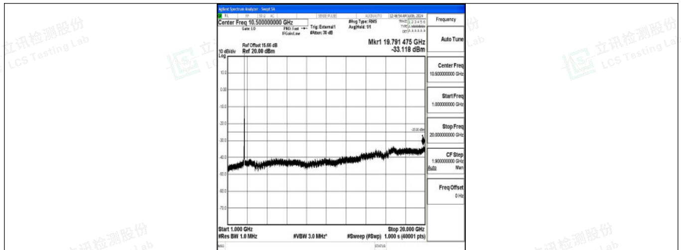
Band38_20MHz_QPSK_38150_1RB#0_1000~20000_1000~20000
