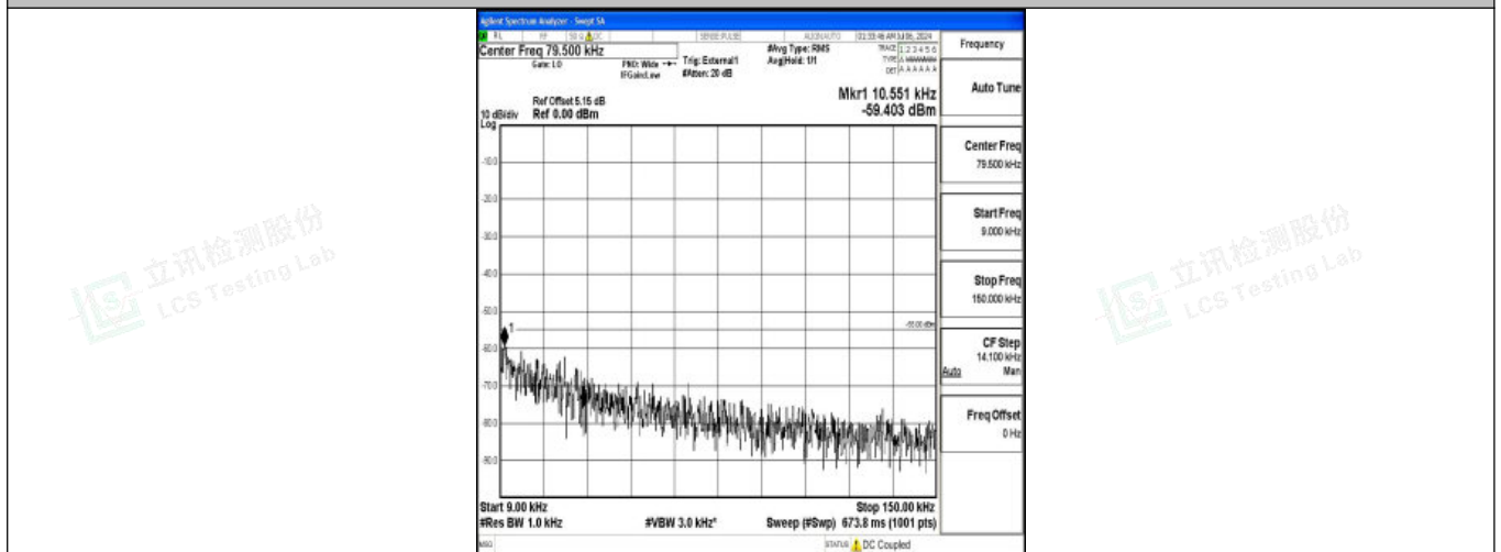
Band38_15MHz_16QAM_38175_1RB#0_0.009~0.15_0.009~0.15
