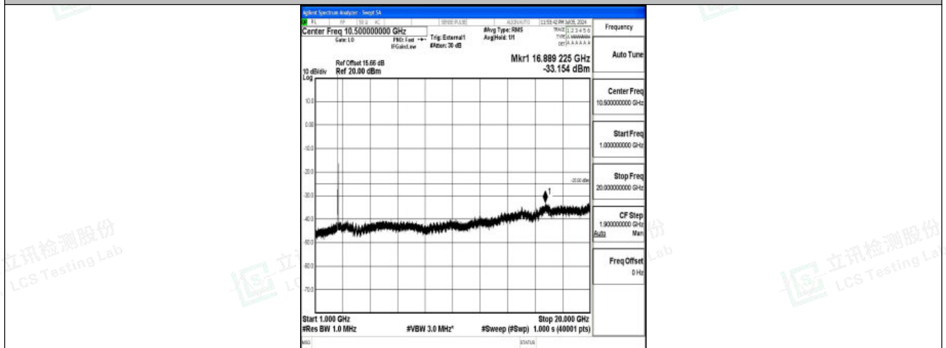
Band38_10MHz_QPSK_37800_1RB#0_1000~20000_1000~20000
