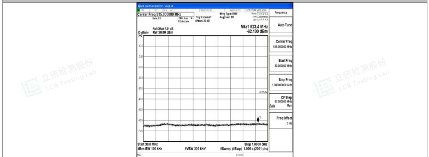
Band38_10MHz_16QAM_37800_1RB#0_30~1000_30~1000
