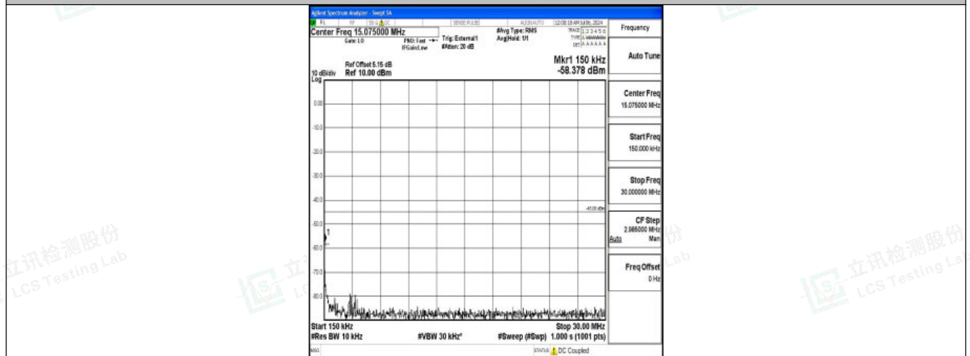
Band38_10MHz_QPSK_38200_1RB#0_0.15~30_0.15~30
