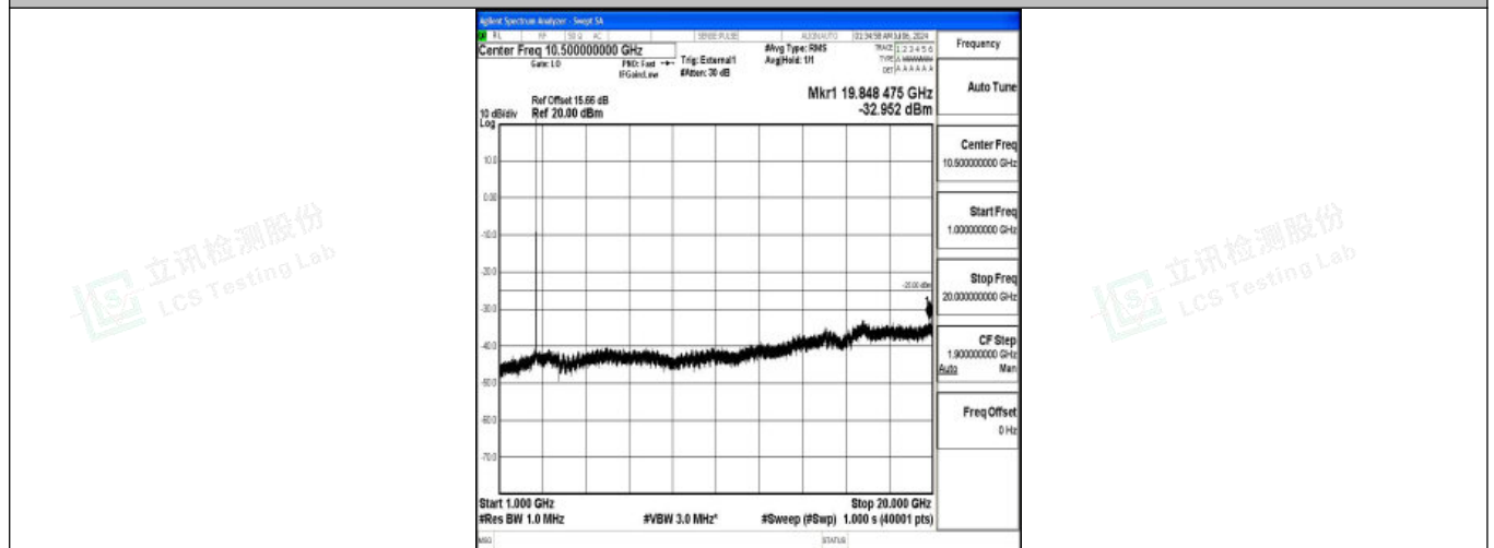
Band38_15MHz_16QAM_38175_1RB#0_1000~20000_1000~20000
