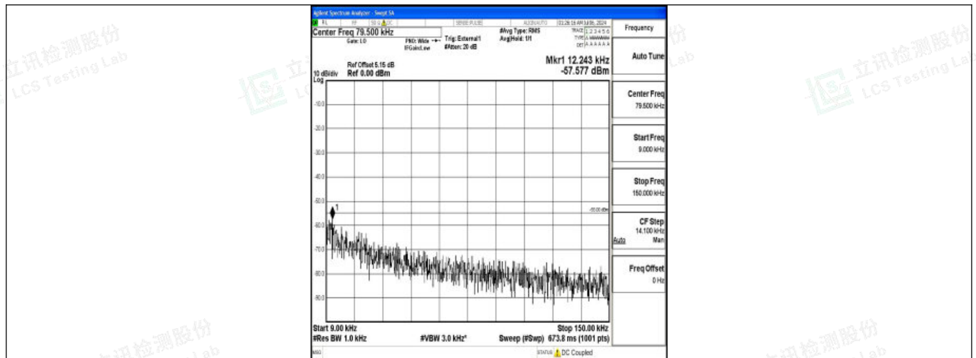
Band38_15MHz_16QAM_37825_1RB#0_0.009~0.15_0.009~0.15
