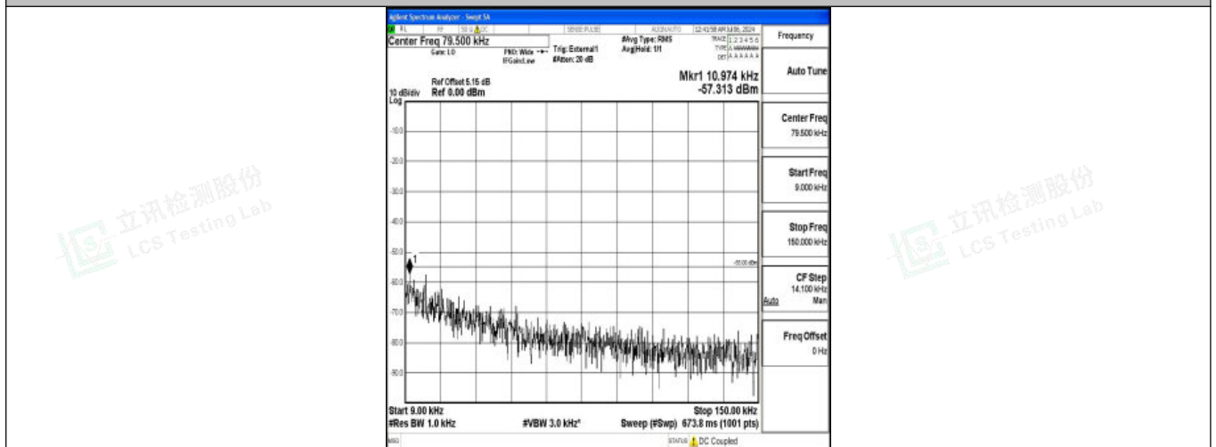
Band38_20MHz_QPSK_38000_1RB#0_0.009~0.15_0.009~0.15
