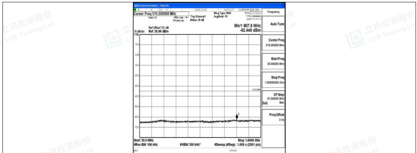
Band38_10MHz_16QAM_38000_1RB#0_30~1000_30~1000
