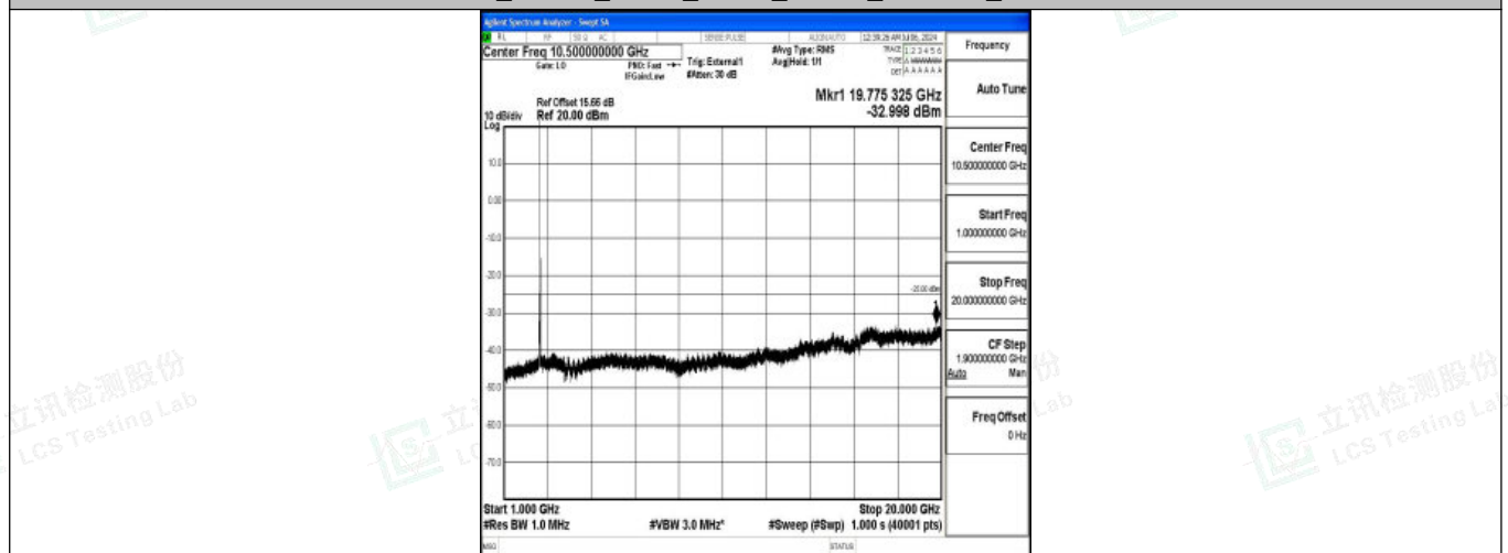
Band38_20MHz_QPSK_37850_1RB#0_1000~20000_1000~20000
