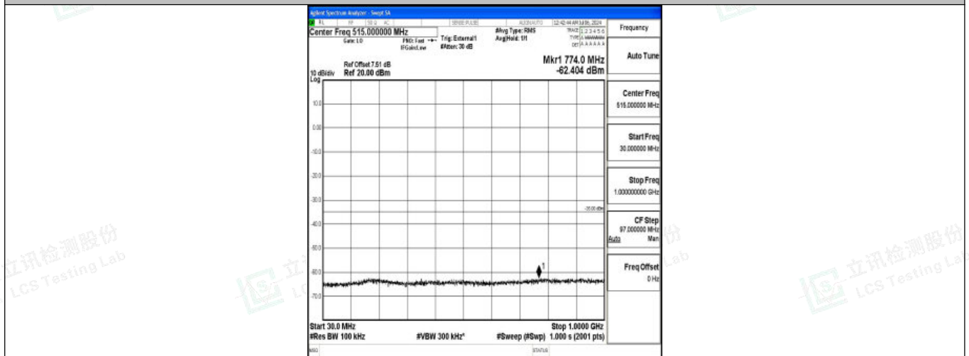
Band38_20MHz_QPSK_38000_1RB#0_30~1000_30~1000
