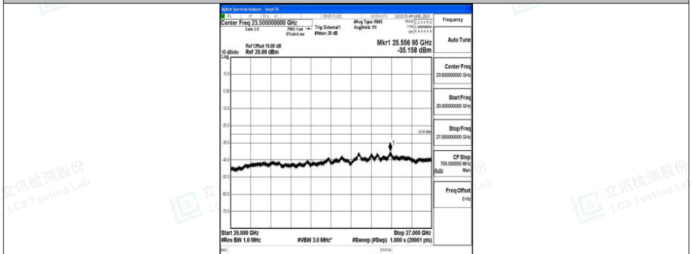
Band38_10MHz_QPSK_38200_1RB#0_20000~27000_20000~27000
