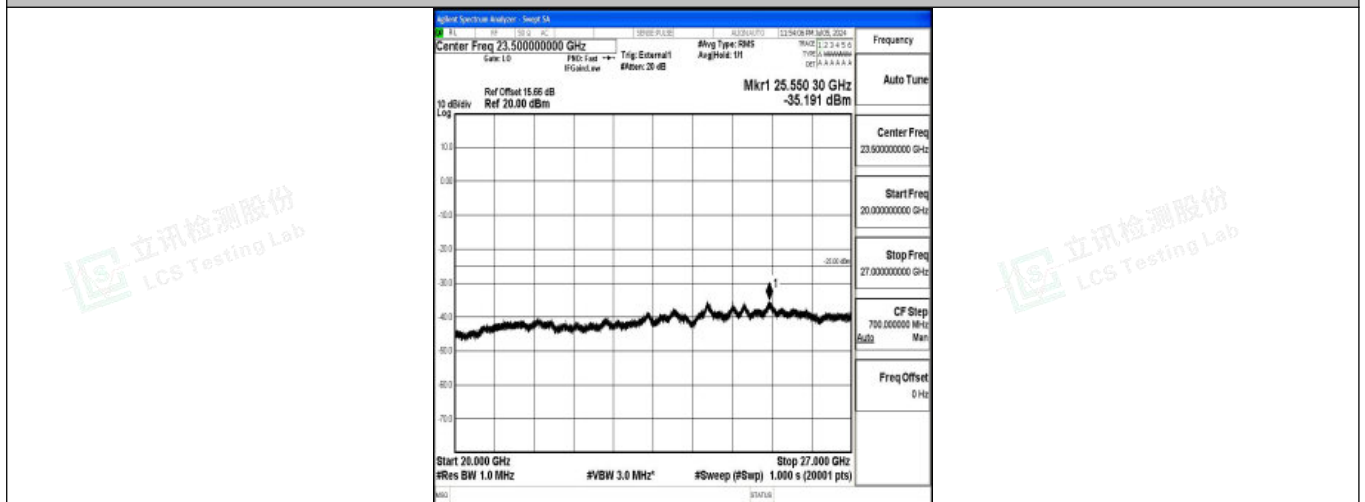
Band38_10MHz_QPSK_37800_1RB#0_20000~27000_20000~27000
