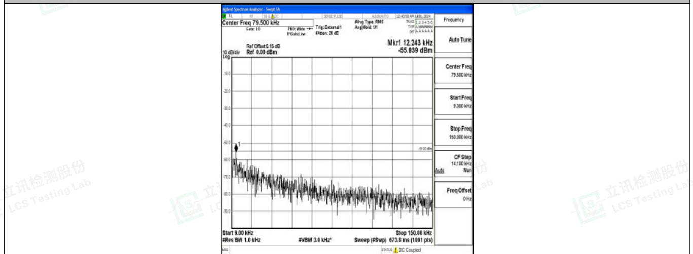
Band38_20MHz_16QAM_38000_1RB#0_0.009~0.15_0.009~0.15
