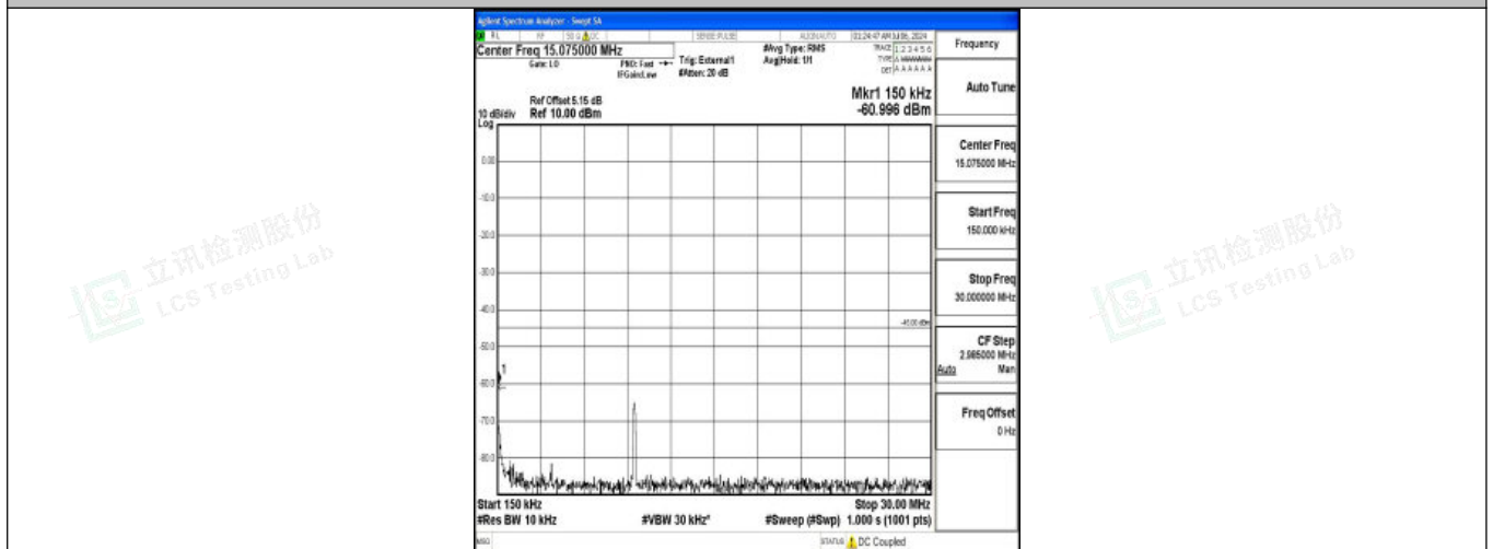
Band38_15MHz_QPSK_37825_1RB#0_0.15~30_0.15~30
