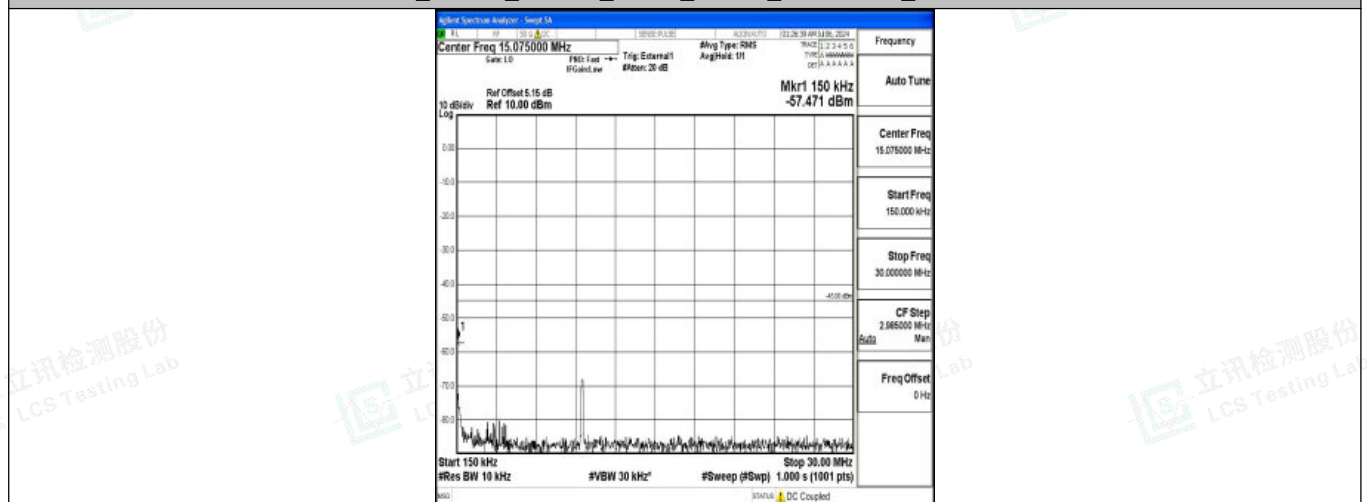
Band38_15MHz_16QAM_37825_1RB#0_0.15~30_0.15~30
