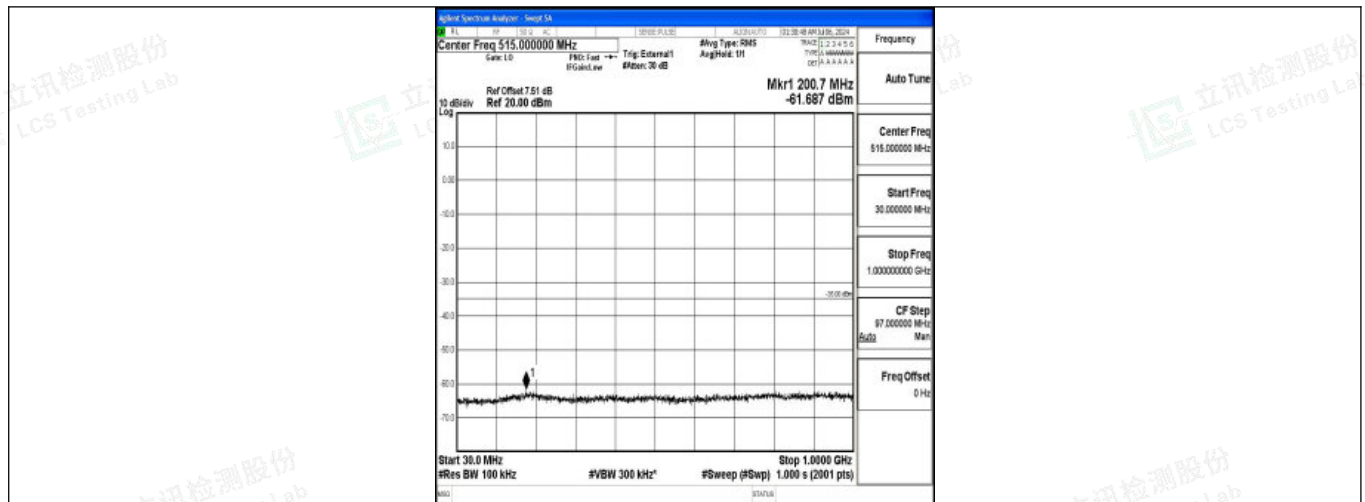
Band38_15MHz_16QAM_38000_1RB#0_30~1000_30~1000
