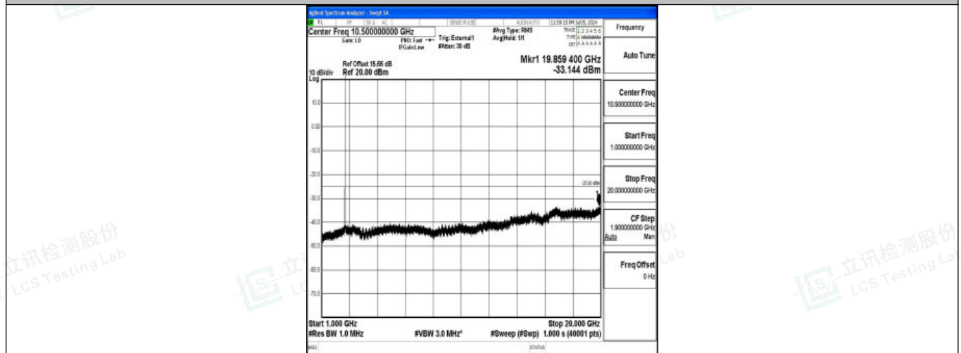
Band38_10MHz_16QAM_38000_1RB#0_1000~20000_1000~20000
