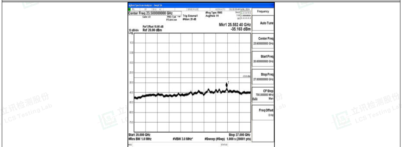
Band38_15MHz_QPSK_38175_1RB#0_20000~27000_20000~27000
