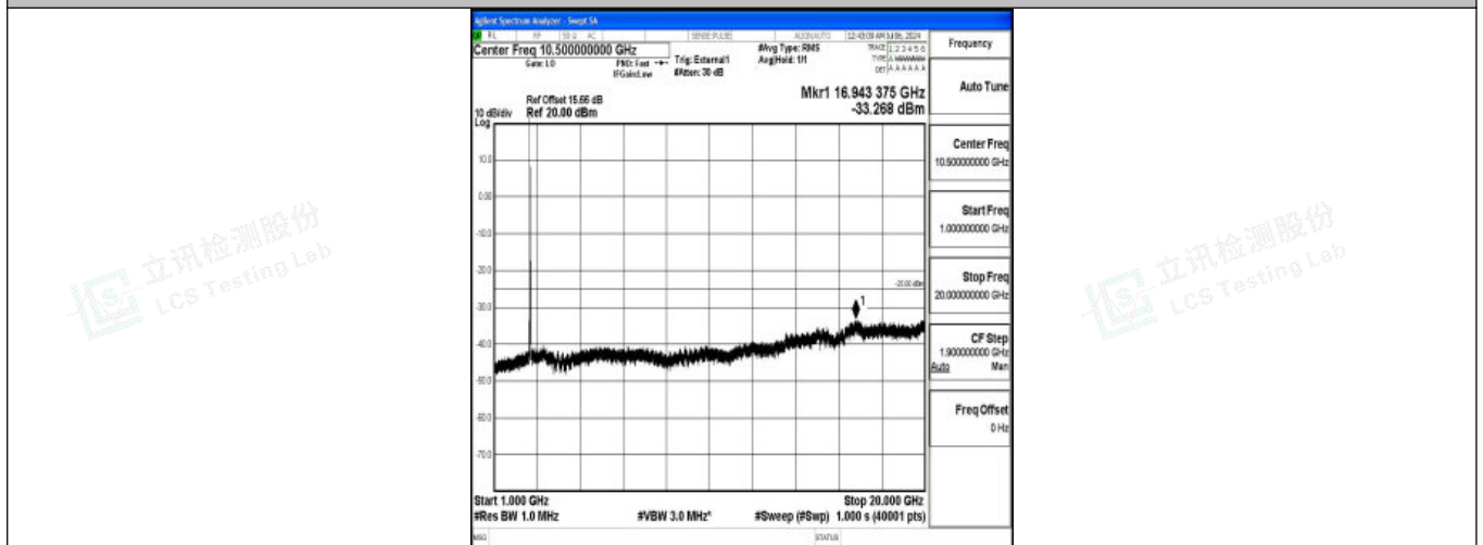
Band38_20MHz_QPSK_38000_1RB#0_1000~20000_1000~20000
