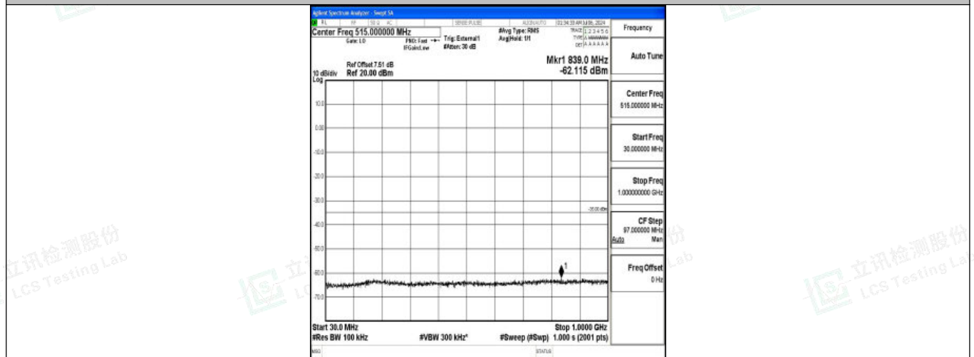
Band38_15MHz_16QAM_38175_1RB#0_30~1000_30~1000
