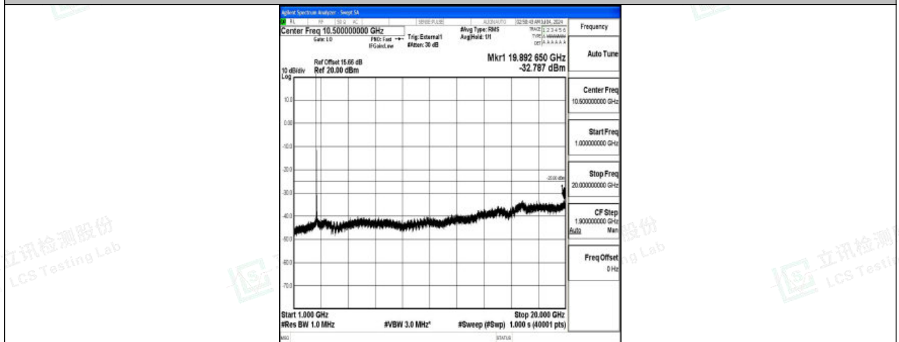
Band41_20MHz_16QAM_40620_1RB#0_1000~20000_1000~20000
