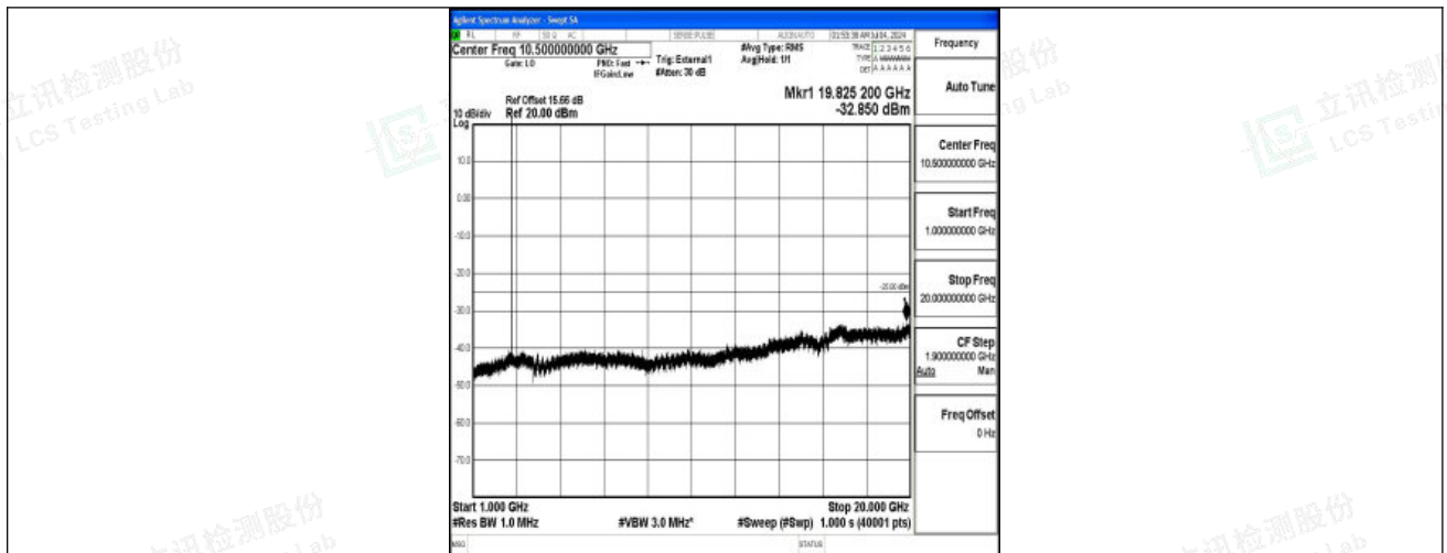
Band41_10MHz_QPSK_41540_1RB#0_1000~20000_1000~20000
