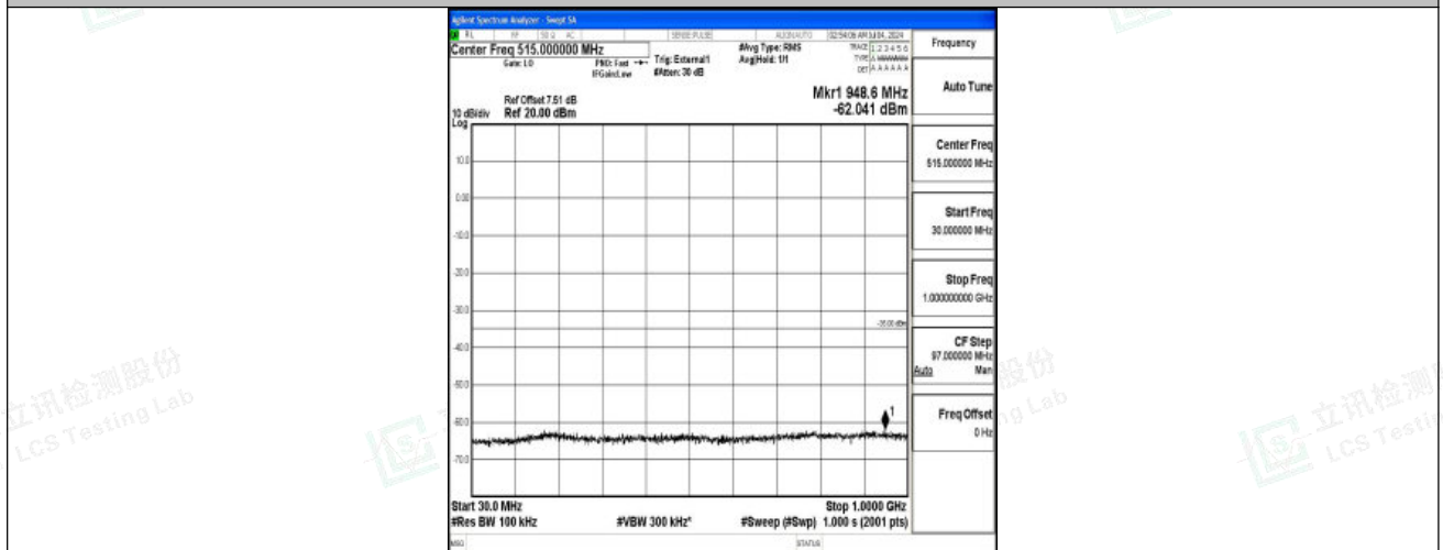
Band41_20MHz_16QAM_41490_1RB#0_30~1000_30~1000
