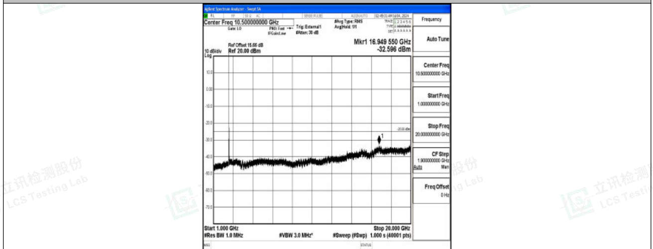
Band41_20MHz_QPSK_39750_1RB#0_1000~20000_1000~20000
