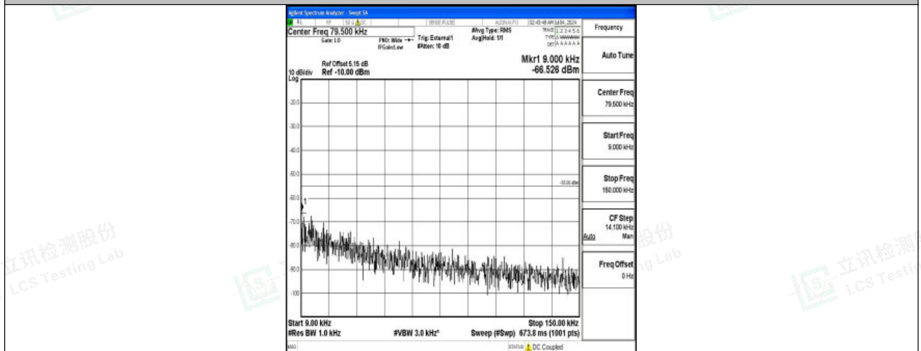
Band41_20MHz_QPSK_39750_1RB#0_0.009~0.15_0.009~0.15
