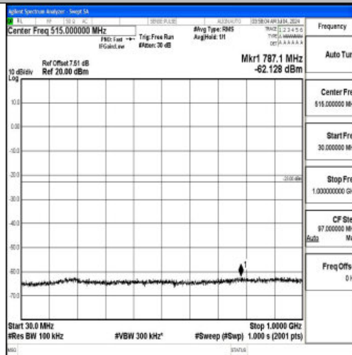
Band66_5MHz_QPSK_131997_1RB#0_30~1000_30~1000
