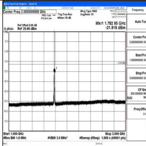
Band66_1.4MHz_16QAM_132665_1RB#0_1000~3000_1000~3000
