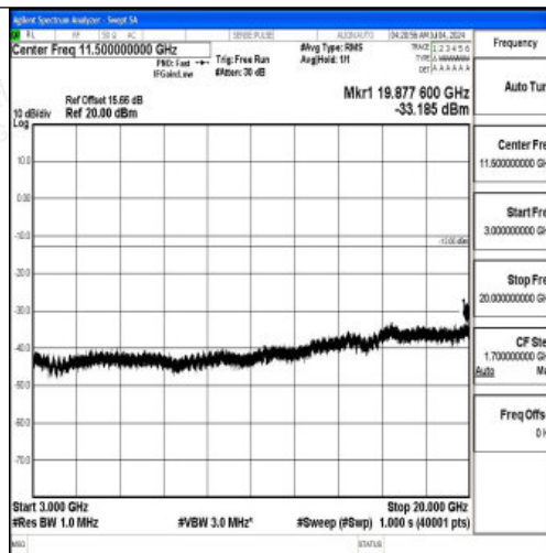
Band66_10MHz_QPSK_132622_1RB#0_3000~20000_3000~20000
