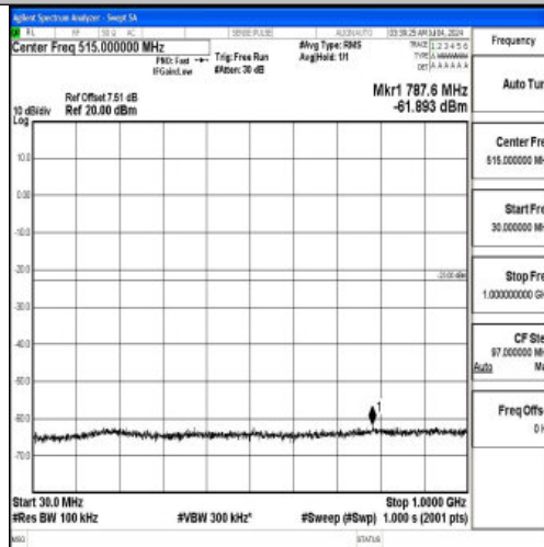
Band66_3MHz_16QAM_132322_1RB#0_30~1000_30~1000
