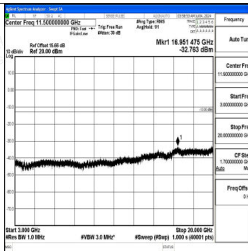
Band66_5MHz_16QAM_131997_1RB#0_3000~20000_3000~20000
