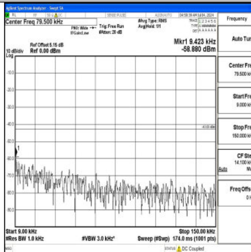
Band66_20MHz_QPSK_132572_1RB#0_0.009~0.15_0.009~0.15
