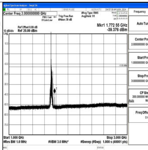
Band66_20MHz_QPSK_132072_1RB#0_1000~3000_1000~3000
