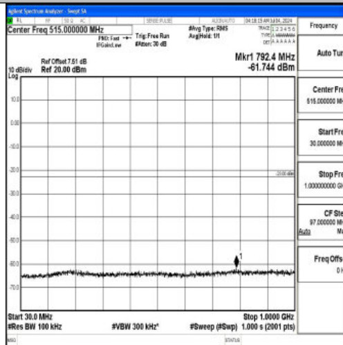
Band66_10MHz_QPSK_132022_1RB#0_30~1000_30~1000
