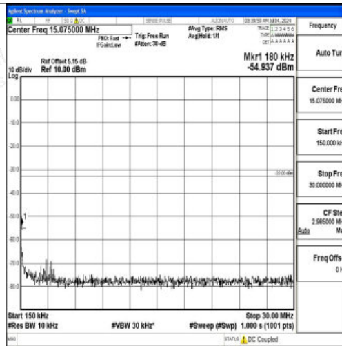
Band66_3MHz_QPSK_132657_1RB#0_0.15~30_0.15~30
