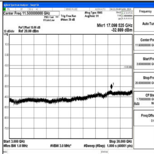
Band66_10MHz_16QAM_132622_1RB#0_3000~20000_3000~20000
