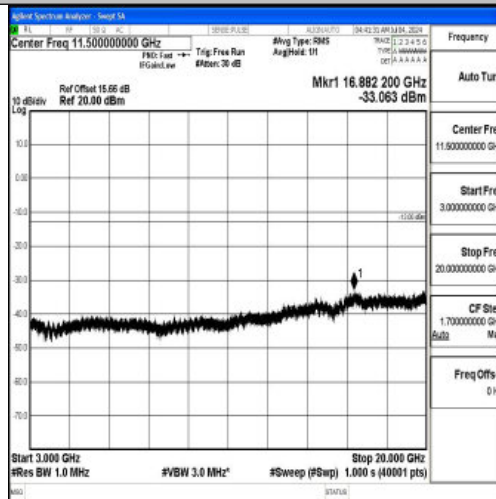
Band66_15MHz_16QAM_132597_1RB#0_3000~20000_3000~20000
