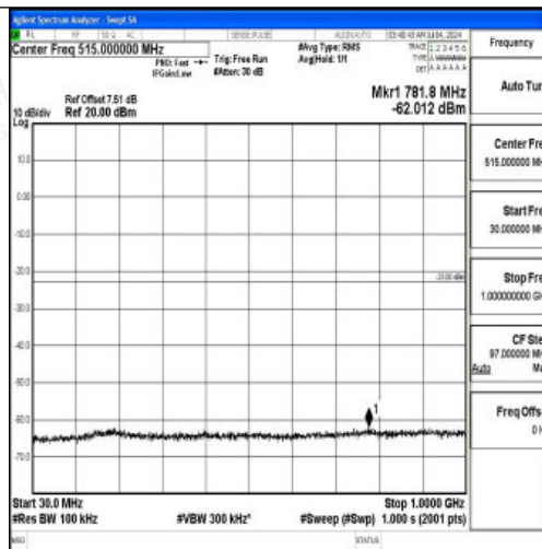
Band66_3MHz_16QAM_132657_1RB#0_30~1000_30~1000
