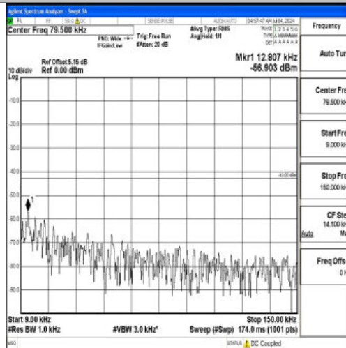
Band66_20MHz_16QAM_132072_1RB#0_0.009~0.15_0.009~0.15
