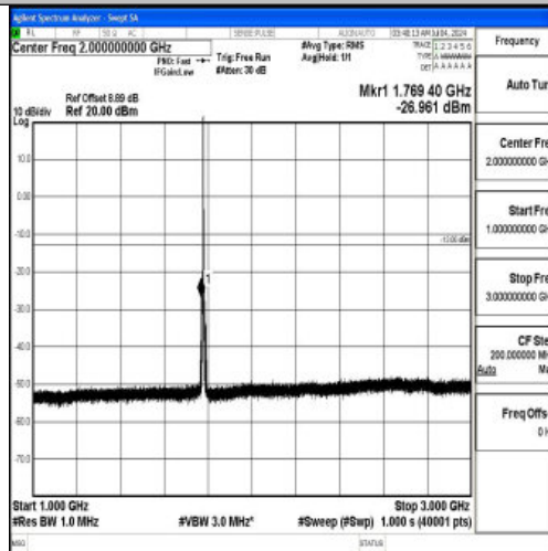
Band66_3MHz_QPSK_132657_1RB#0_1000~3000_1000~3000
