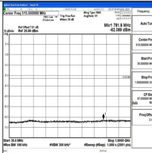
Band66_3MHz_QPSK_131987_1RB#0_30~1000_30~1000
