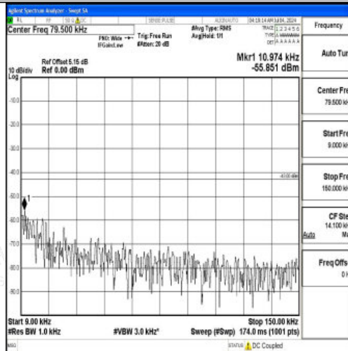
Band66_10MHz_QPSK_132322_1RB#0_0.009~0.15_0.009~0.15
