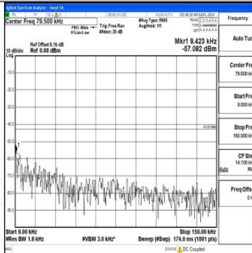
Band66_3MHz_16QAM_132657_1RB#0_0.009~0.15_0.009~0.15
