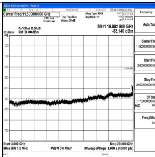
Band66_3MHz_QPSK_132657_1RB#0_3000~20000_3000~20000
