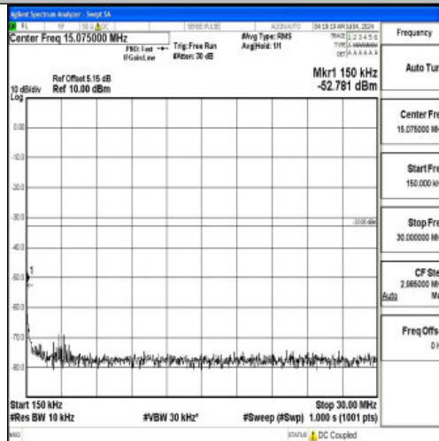
Band66_10MHz_QPSK_132322_1RB#0_0.15~30_0.15~30
