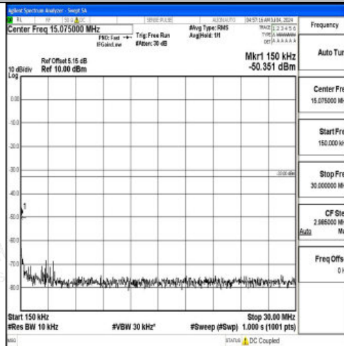
Band66_20MHz_QPSK_132072_1RB#0_0.15~30_0.15~30
