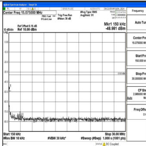
Band66_10MHz_16QAM_132622_1RB#0_0.15~30_0.15~30
