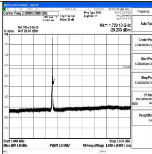
Band66_3MHz_QPSK_131987_1RB#0_1000~3000_1000~3000
