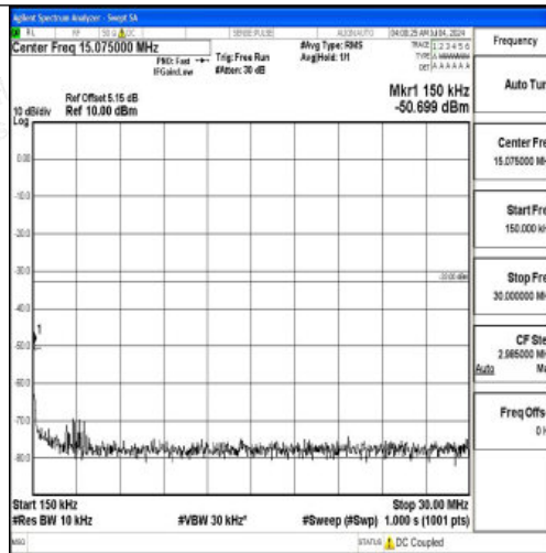
Band66_5MHz_QPSK_132647_1RB#0_0.15~30_0.15~30
