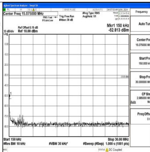
Band66_20MHz_16QAM_132072_1RB#0_0.15~30_0.15~30
