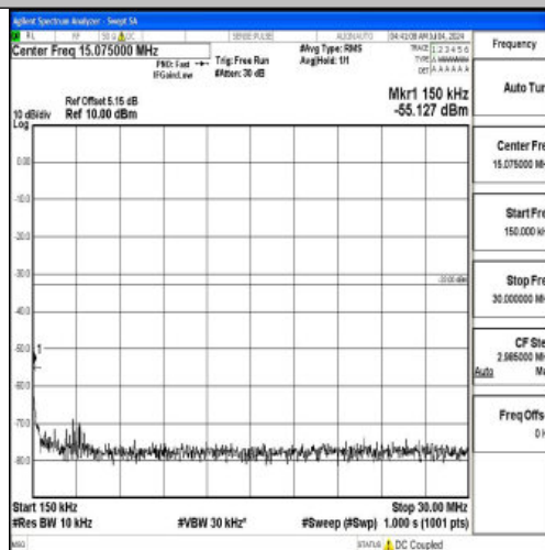
Band66_15MHz_16QAM_132597_1RB#0_0.15~30_0.15~30
