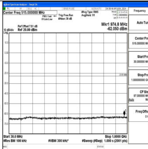
Band66_15MHz_16QAM_132047_1RB#0_30~1000_30~1000
