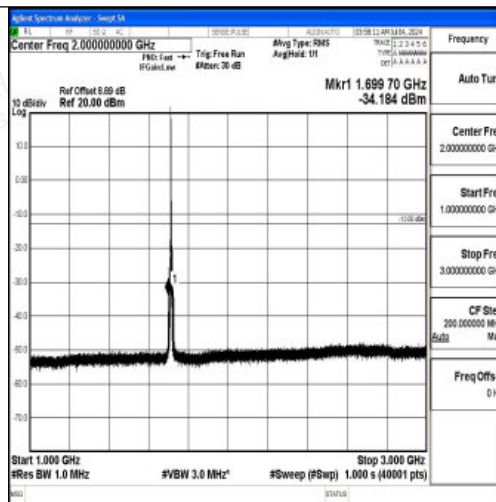
Band66_5MHz_QPSK_131997_1RB#0_1000~3000_1000~3000
