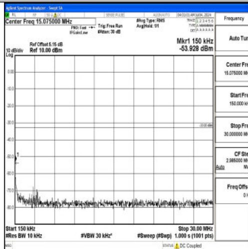
Band66_5MHz_16QAM_132647_1RB#0_0.15~30_0.15~30
