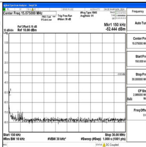
Band66_10MHz_QPSK_132622_1RB#0_0.15~30_0.15~30
