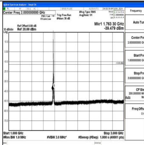
Band66_5MHz_QPSK_132647_1RB#0_1000~3000_1000~3000
