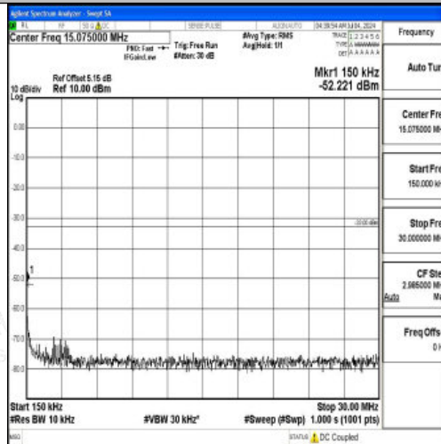
Band66_15MHz_16QAM_132322_1RB#0_0.15~30_0.15~30
