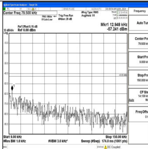
Band66_3MHz_QPSK_132657_1RB#0_0.009~0.15_0.009~0.15
