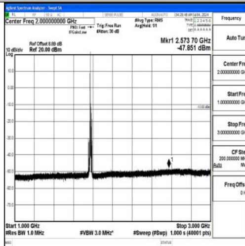
Band66_10MHz_QPSK_132622_1RB#0_1000~3000_1000~3000
