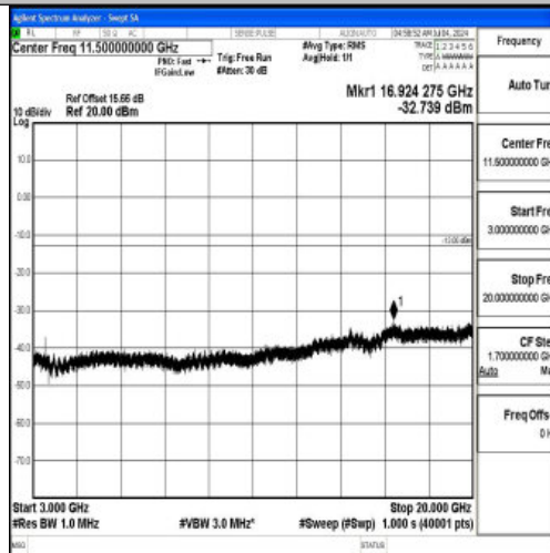
Band66_20MHz_QPSK_132322_1RB#0_3000~20000_3000~20000
