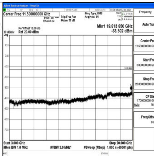
Band66_5MHz_QPSK_132647_1RB#0_3000~20000_3000~20000
