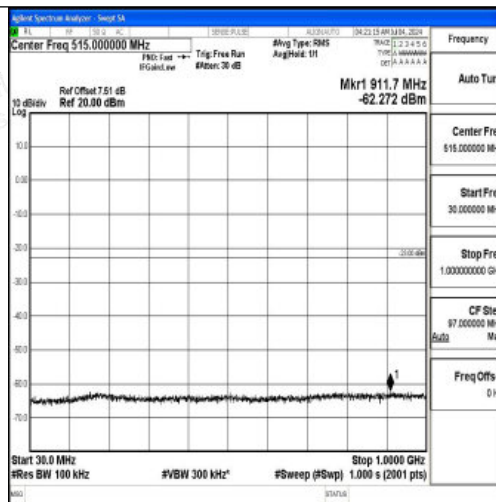
Band66_10MHz_16QAM_132622_1RB#0_30~1000_30~1000
