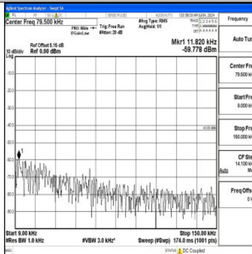
Band66_3MHz_16QAM_131987_1RB#0_0.009~0.15_0.009~0.15
