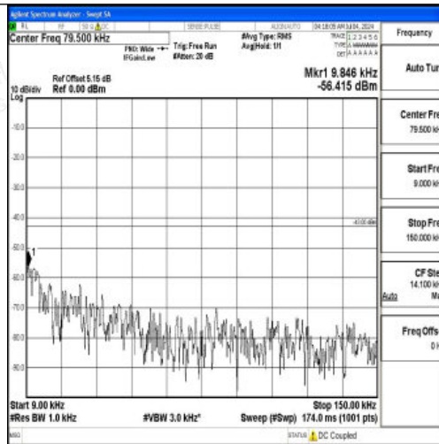
Band66_10MHz_QPSK_132022_1RB#0_0.009~0.15_0.009~0.15
