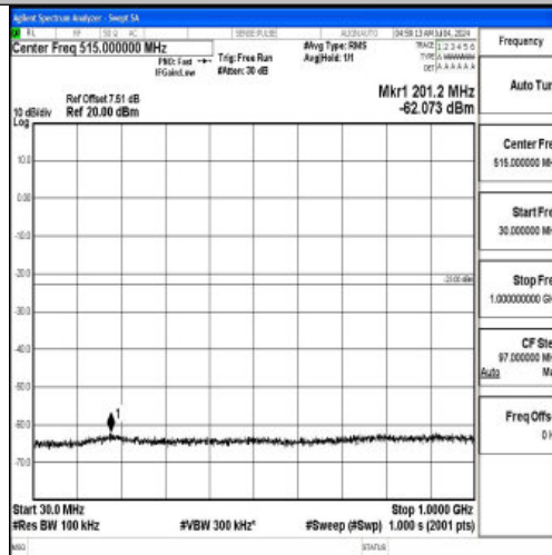
Band66_20MHz_16QAM_132322_1RB#0_30~1000_30~1000
