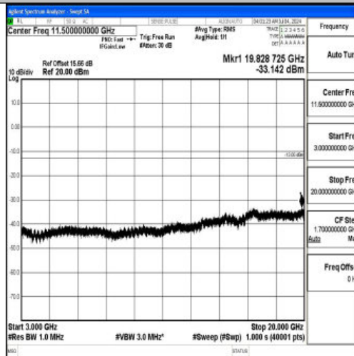
Band66_5MHz_16QAM_132647_1RB#0_3000~20000_3000~20000
