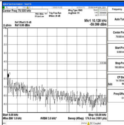
Band66_5MHz_16QAM_131997_1RB#0_0.009~0.15_0.009~0.15
