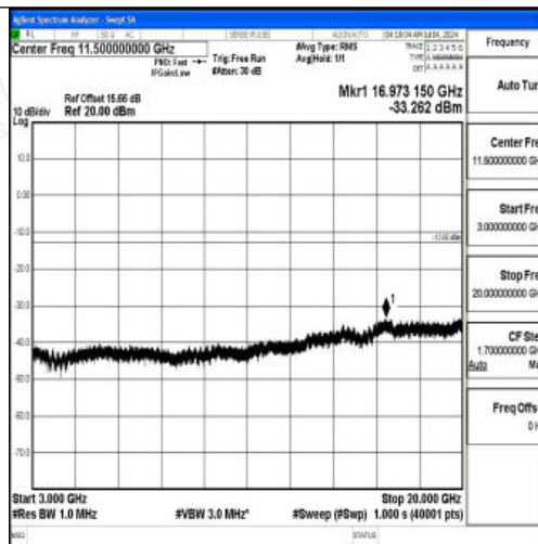
Band66_10MHz_16QAM_132022_1RB#0_3000~20000_3000~20000
