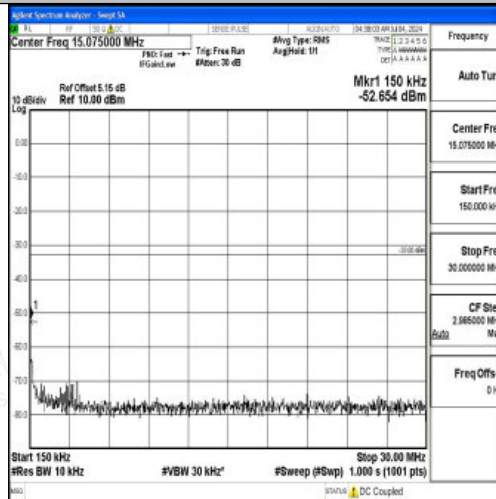
Band66_15MHz_QPSK_132047_1RB#0_0.15~30_0.15~30
