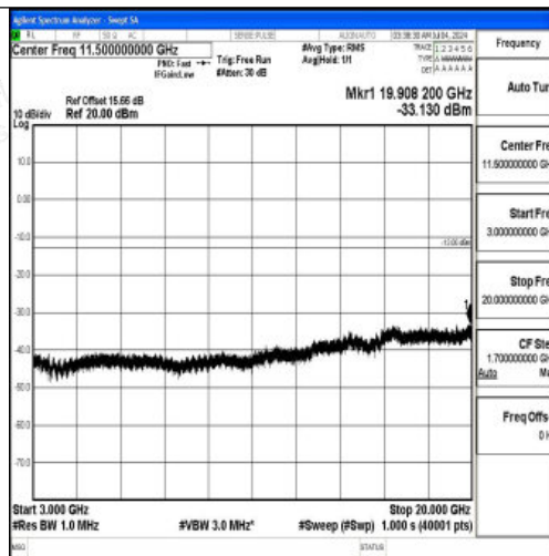
Band66_3MHz_16QAM_131987_1RB#0_3000~20000_3000~20000
