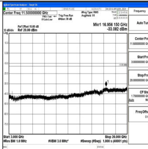
Band66_10MHz_QPSK_132322_1RB#0_3000~20000_3000~20000
