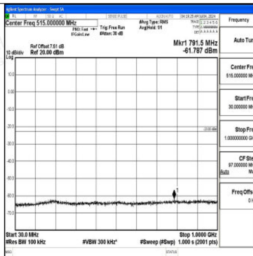
Band66_10MHz_QPSK_132322_1RB#0_30~1000_30~1000
