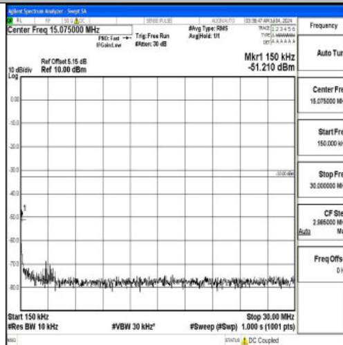
Band66_3MHz_QPSK_132322_1RB#0_0.15~30_0.15~30
