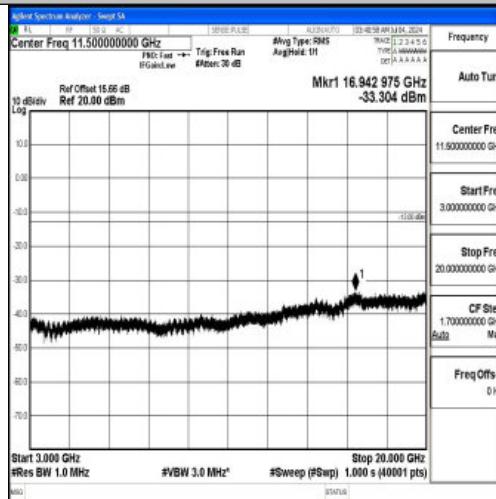
Band66_3MHz_16QAM_132657_1RB#0_3000~20000_3000~20000
