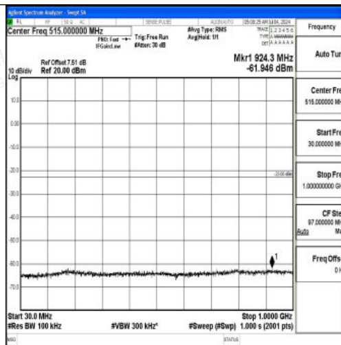
Band66_20MHz_16QAM_132572_1RB#0_30~1000_30~1000
