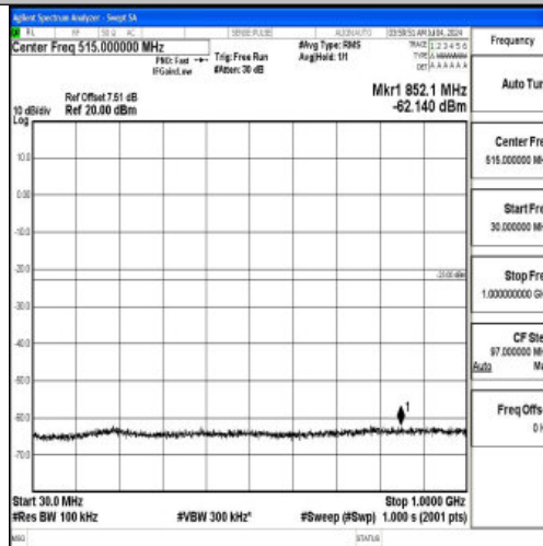
Band66_5MHz_16QAM_132322_1RB#0_30~1000_30~1000
