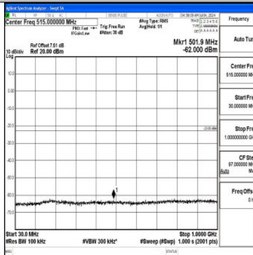
Band66_15MHz_QPSK_132047_1RB#0_30~1000_30~1000
