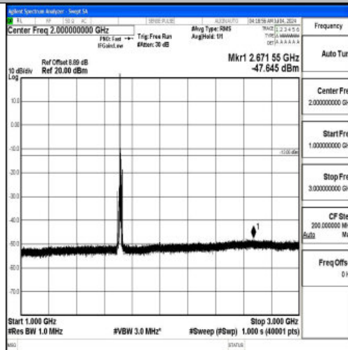
Band66_10MHz_16QAM_132022_1RB#0_1000~3000_1000~3000
