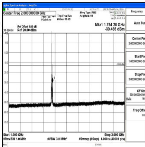
Band66_3MHz_16QAM_132322_1RB#0_1000~3000_1000~3000
