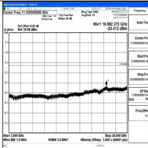
Band66_5MHz_QPSK_131997_1RB#0_3000~20000_3000~20000
