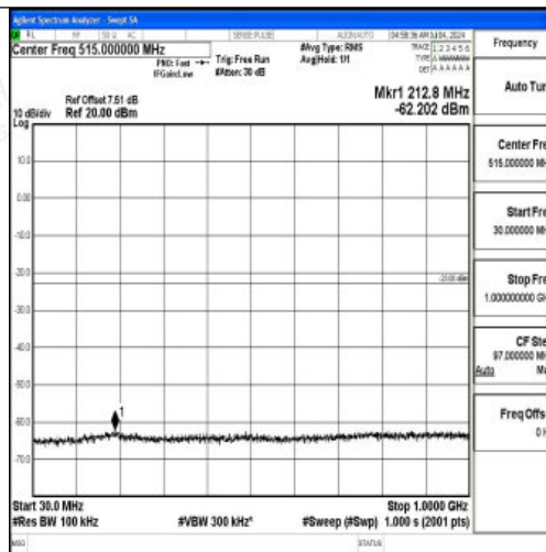
Band66_20MHz_QPSK_132322_1RB#0_30~1000_30~1000
