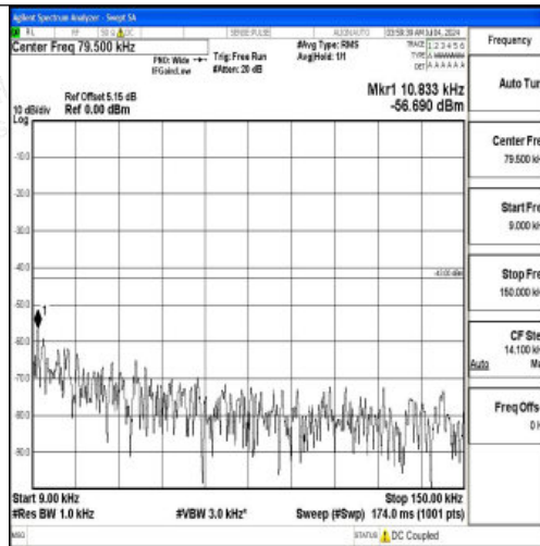
Band66_5MHz_16QAM_132322_1RB#0_0.009~0.15_0.009~0.15
