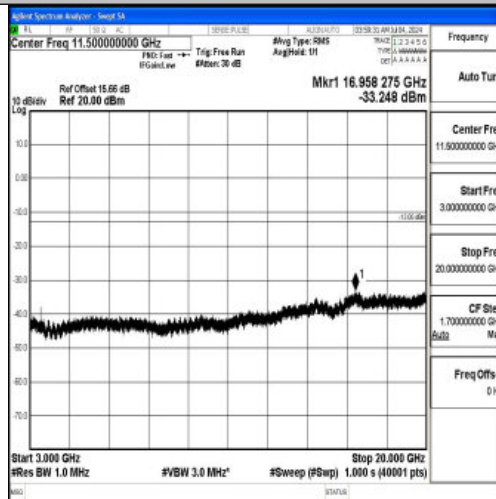
Band66_5MHz_QPSK_132322_1RB#0_3000~20000_3000~20000
