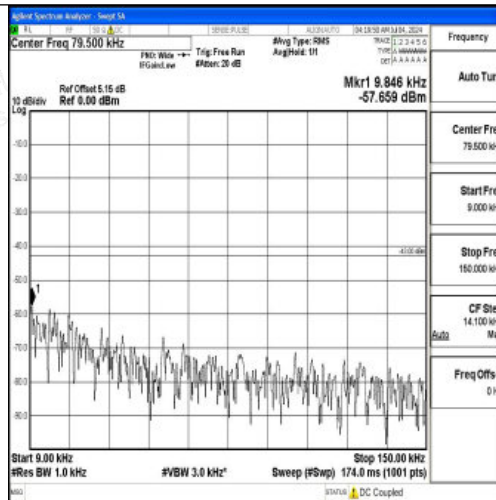
Band66_10MHz_16QAM_132322_1RB#0_0.009~0.15_0.009~0.15
