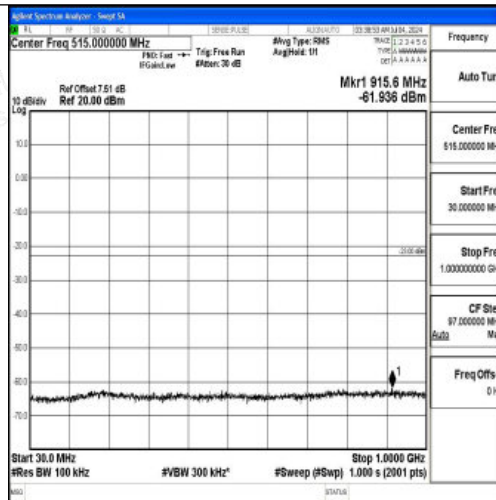
Band66_3MHz_QPSK_132322_1RB#0_30~1000_30~1000
