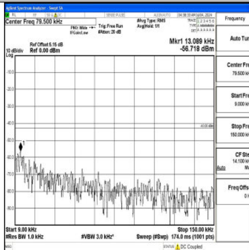
Band66_15MHz_16QAM_132047_1RB#0_0.009~0.15_0.009~0.15
