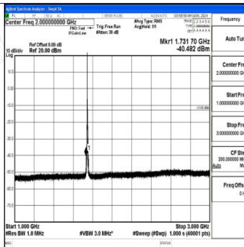
Band66_5MHz_16QAM_132322_1RB#0_1000~3000_1000~3000
