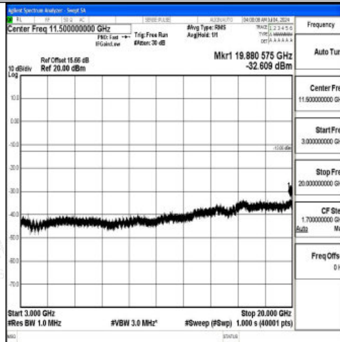
Band66_5MHz_16QAM_132322_1RB#0_3000~20000_3000~20000
