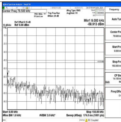
Band66_15MHz_QPSK_132047_1RB#0_0.009~0.15_0.009~0.15
