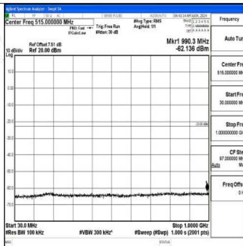
Band66_15MHz_16QAM_132597_1RB#0_30~1000_30~1000
