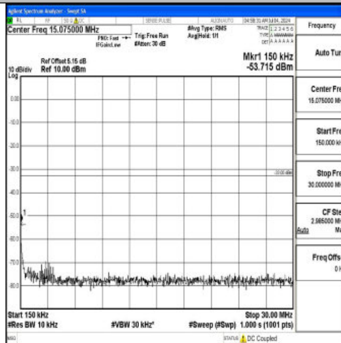
Band66_20MHz_QPSK_132322_1RB#0_0.15~30_0.15~30
