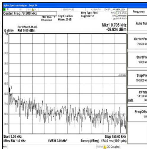
Band66_20MHz_QPSK_132072_1RB#0_0.009~0.15_0.009~0.15
