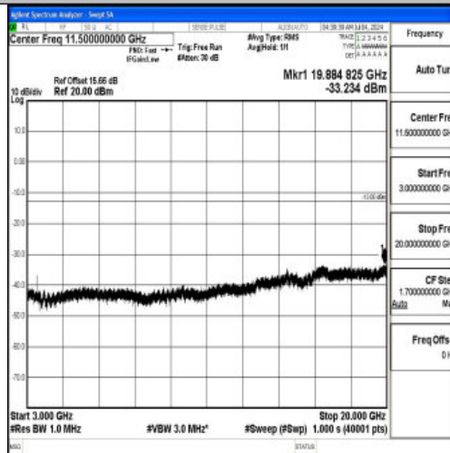
Band66_15MHz_QPSK_132322_1RB#0_3000~20000_3000~20000
