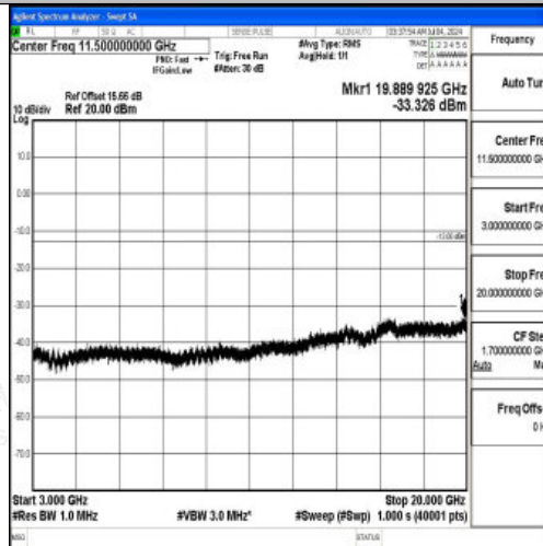
Band66_3MHz_QPSK_131987_1RB#0_3000~20000_3000~20000
