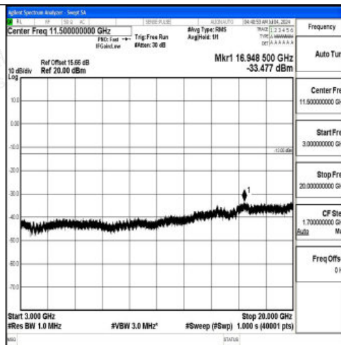
Band66_15MHz_QPSK_132597_1RB#0_3000~20000_3000~20000
