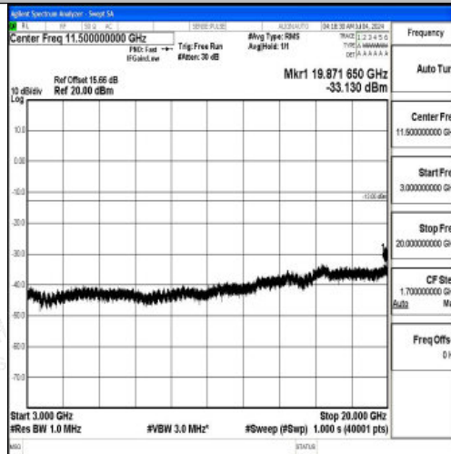
Band66_10MHz_QPSK_132022_1RB#0_3000~20000_3000~20000
