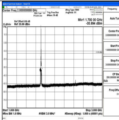
Band66_5MHz_16QAM_131997_1RB#0_1000~3000_1000~3000
