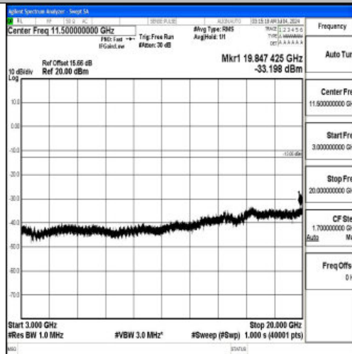
Band66_1.4MHz_16QAM_132665_1RB#0_3000~20000_3000~20000
