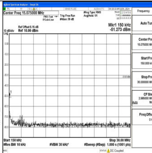
Band66_10MHz_QPSK_132022_1RB#0_0.15~30_0.15~30
