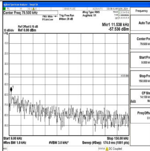
Band66_3MHz_QPSK_132322_1RB#0_0.009~0.15_0.009~0.15
