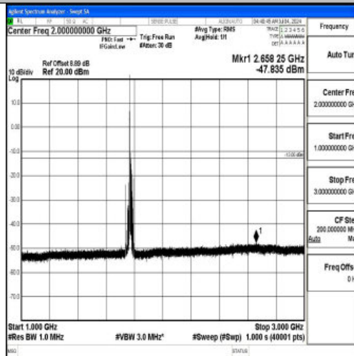
Band66_15MHz_QPSK_132597_1RB#0_1000~3000_1000~3000
