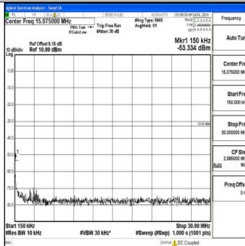
Band66_5MHz_QPSK_132322_1RB#0_0.15~30_0.15~30
