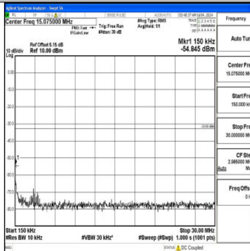
Band66_3MHz_16QAM_132657_1RB#0_0.15~30_0.15~30
