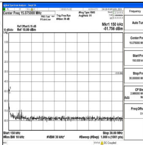
Band66_10MHz_16QAM_132022_1RB#0_0.15~30_0.15~30
