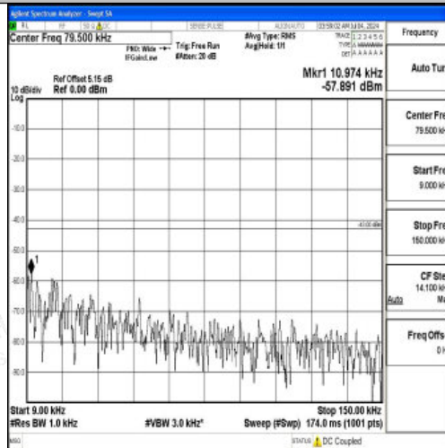
Band66_5MHz_QPSK_132322_1RB#0_0.009~0.15_0.009~0.15
