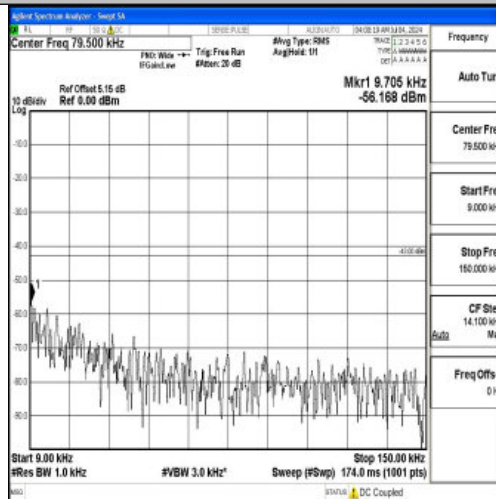
Band66_5MHz_QPSK_132647_1RB#0_0.009~0.15_0.009~0.15
