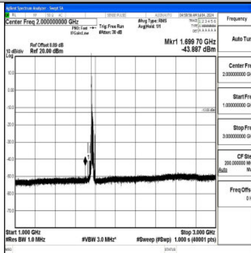
Band66_20MHz_QPSK_132572_1RB#0_1000~3000_1000~3000
