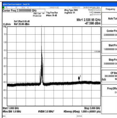
Band66_20MHz_16QAM_132322_1RB#0_1000~3000_1000~3000
