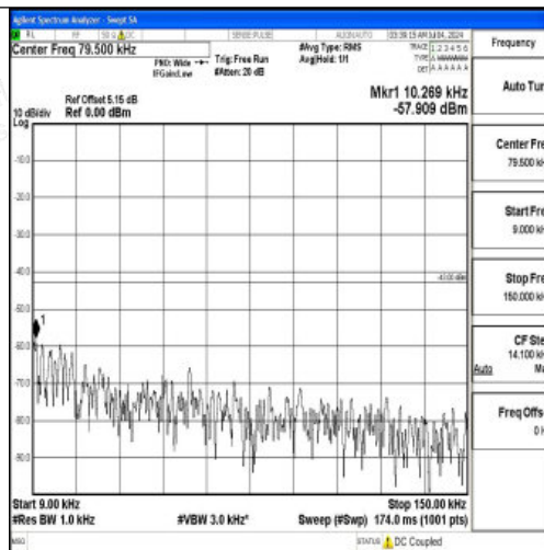
Band66_3MHz_16QAM_132322_1RB#0_0.009~0.15_0.009~0.15
