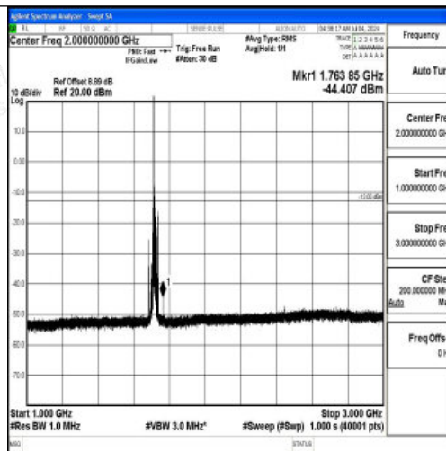
Band66_15MHz_QPSK_132047_1RB#0_1000~3000_1000~3000
