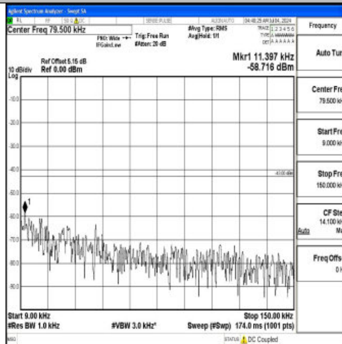
Band66_15MHz_QPSK_132597_1RB#0_0.009~0.15_0.009~0.15
