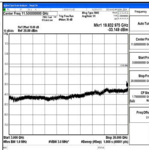
Band66_1.4MHz_QPSK_132665_1RB#0_3000~20000_3000~20000
