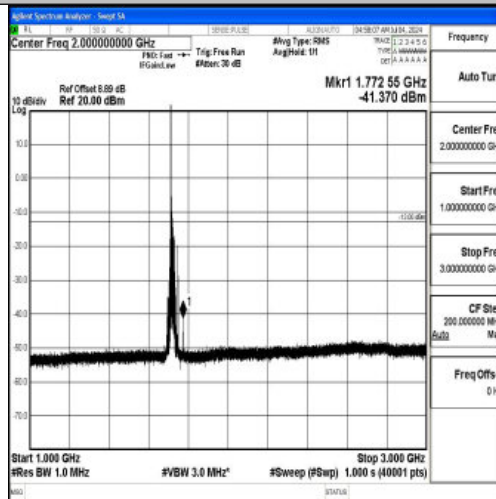
Band66_20MHz_16QAM_132072_1RB#0_1000~3000_1000~3000
