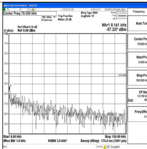
Band66_20MHz_16QAM_132322_1RB#0_0.009~0.15_0.009~0.15
