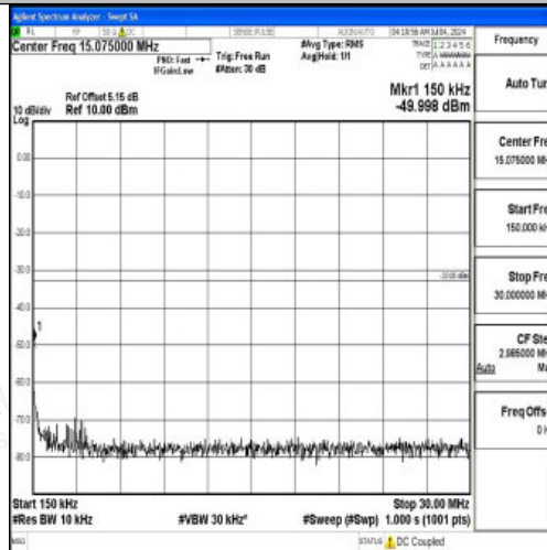
Band66_10MHz_16QAM_132322_1RB#0_0.15~30_0.15~30
