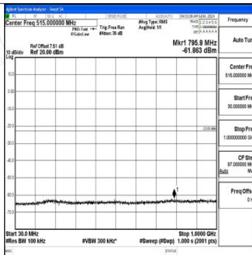
Band66_5MHz_16QAM_132647_1RB#0_30~1000_30~1000
