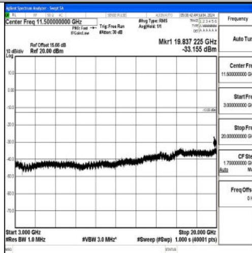
Band66_20MHz_16QAM_132572_1RB#0_3000~20000_3000~20000
