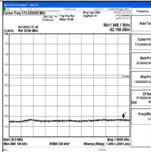
Band66_15MHz_16QAM_132322_1RB#0_30~1000_30~1000
