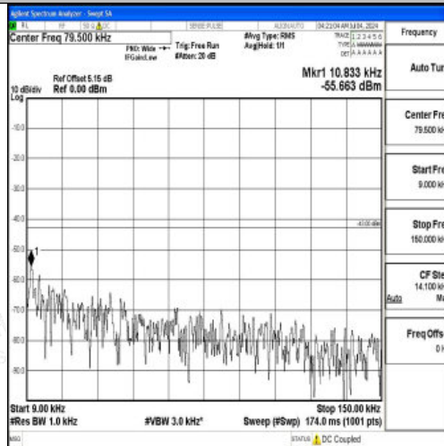
Band66_10MHz_16QAM_132622_1RB#0_0.009~0.15_0.009~0.15
