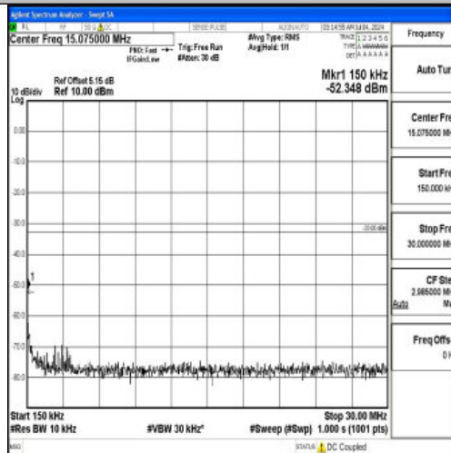
Band66_1.4MHz_16QAM_132665_1RB#0_0.15~30_0.15~30
