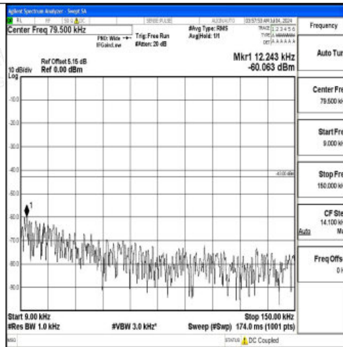
Band66_5MHz_QPSK_131997_1RB#0_0.009~0.15_0.009~0.15
