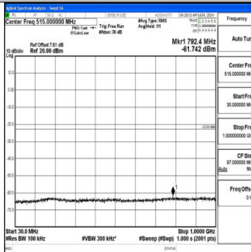
Band66_10MHz_16QAM_132322_1RB#0_30~1000_30~1000
