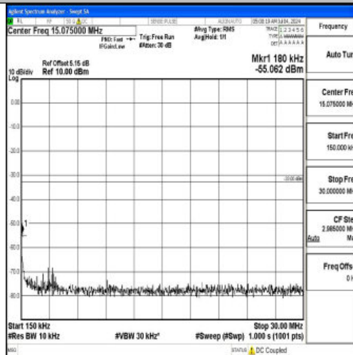
Band66_20MHz_16QAM_132572_1RB#0_0.15~30_0.15~30
