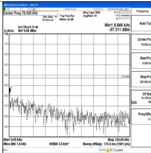
Band66_15MHz_16QAM_132322_1RB#0_0.009~0.15_0.009~0.15
