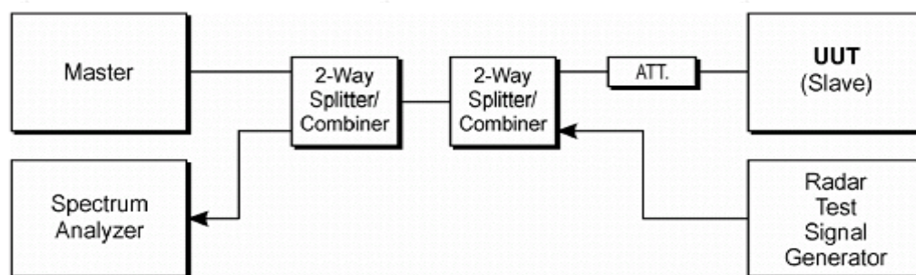
Figure 7-1. Test Setup
