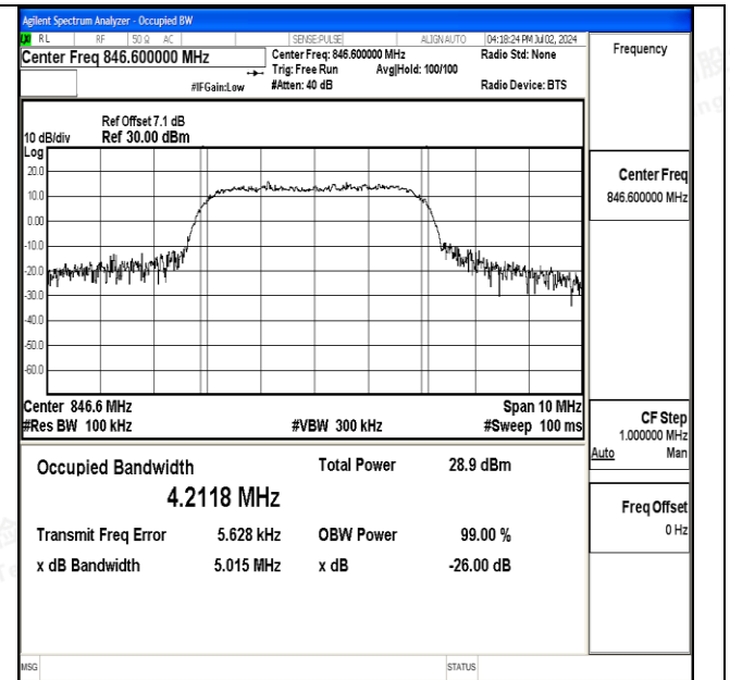
Channel 4233 / 846.6 MHz
