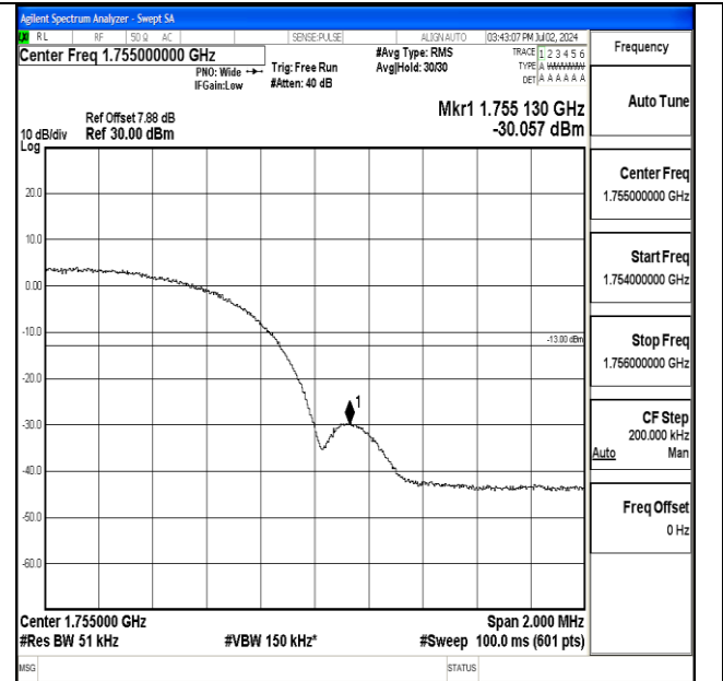
Channel 1513 / 1752.6 MHz
