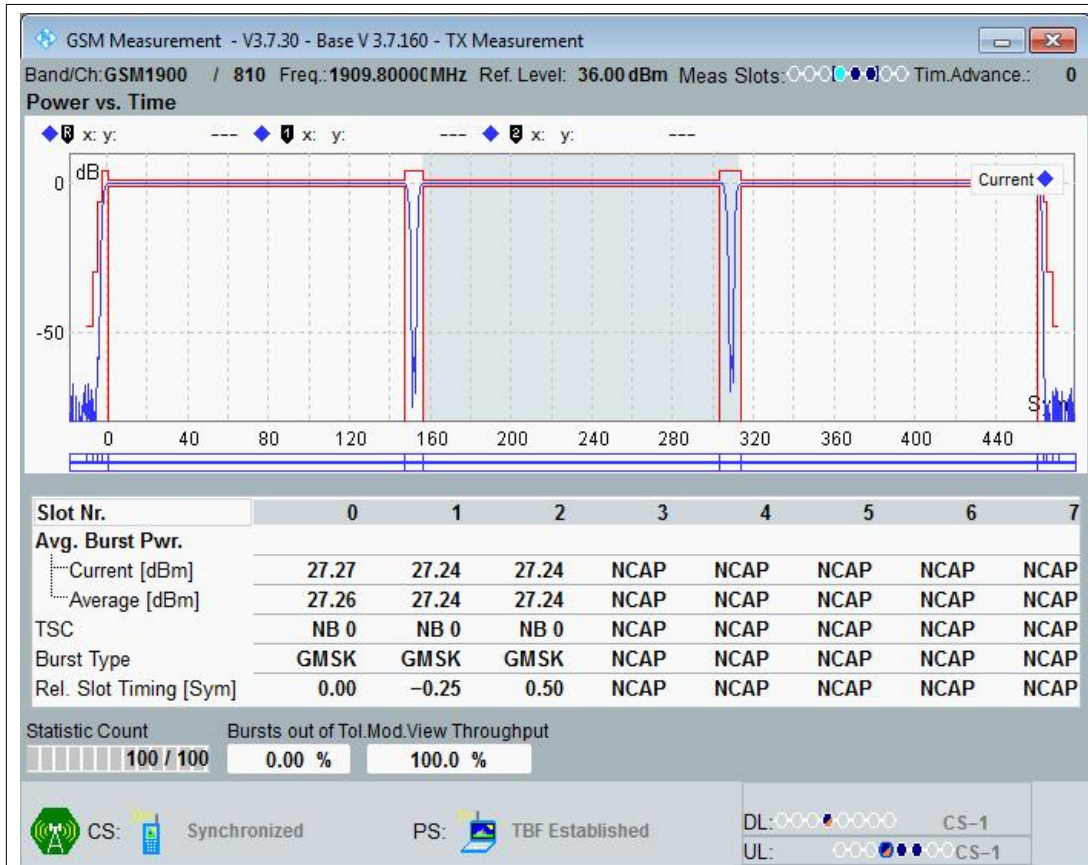
EGPRS1900 3 Slot Channel=810 3 Slot
