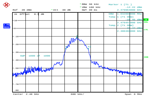
High 1.032MHz
