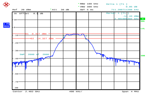
Low 0.711MHz
