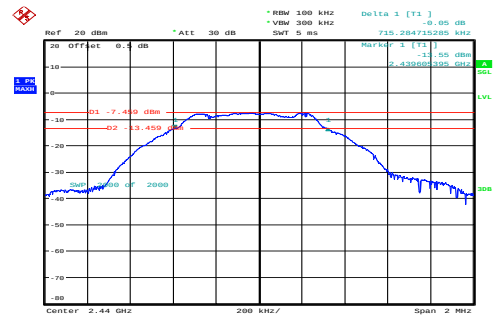
Middle 0.715MHz
