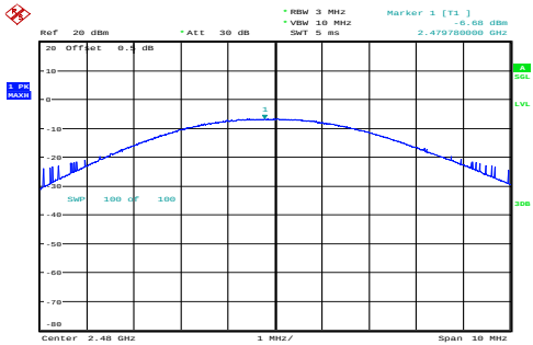
High -6.68dBm
