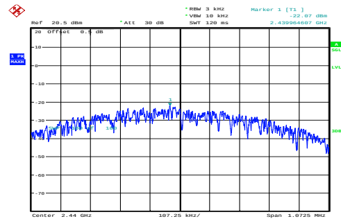
Middle -22.07dBm/3kHz
