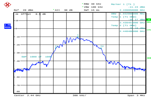
Middle 1.032MHz
