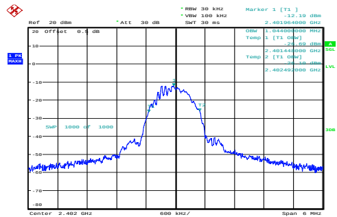
Low 1.044MHz
