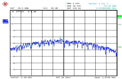
High -23.30dBm/3kHz
