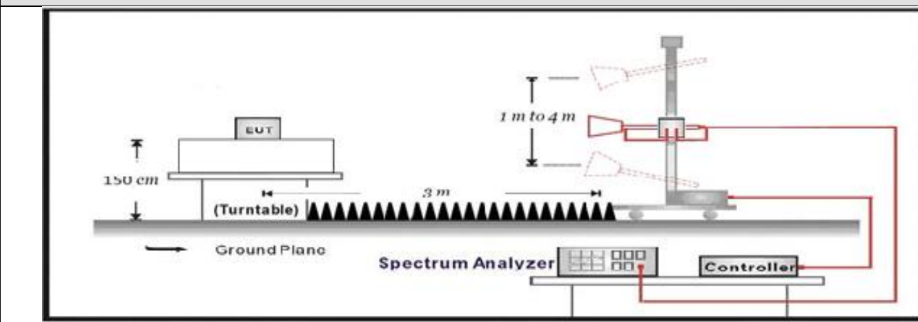
Above 1GHz Test Setup:
