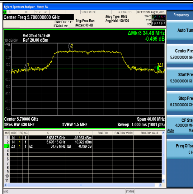
11N20SISO-Ant1-5700
