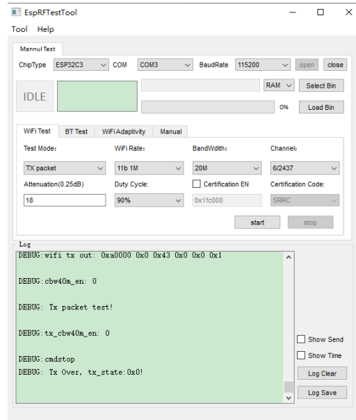
Software Setting Diagram
