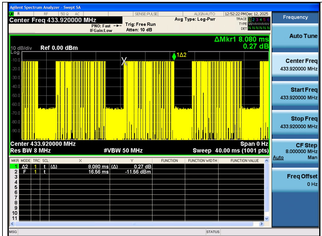
Test_Graph_Full Cycle Testing Demonstration_433.92MHz, GFSK
