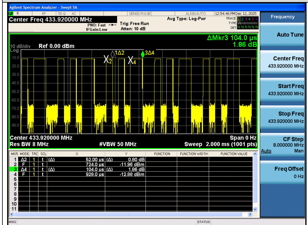
Test_Graph_Pulse_Pulse Type 1_433.92MHz, GFSK
