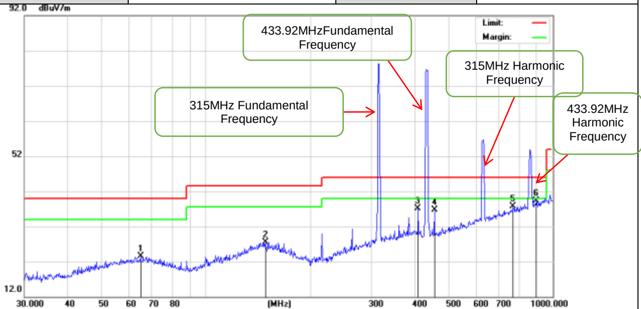
Suspected Data List_ Peak Detection
