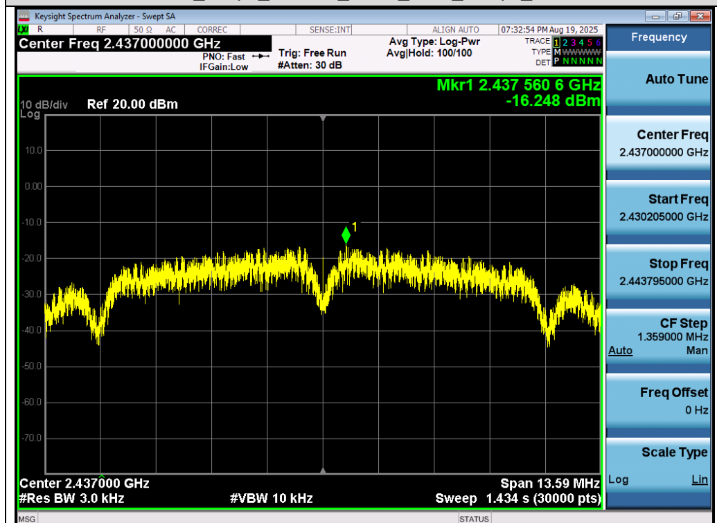
Test_Graph_802.11b_ANT1_2437_1Mbps_PSD
