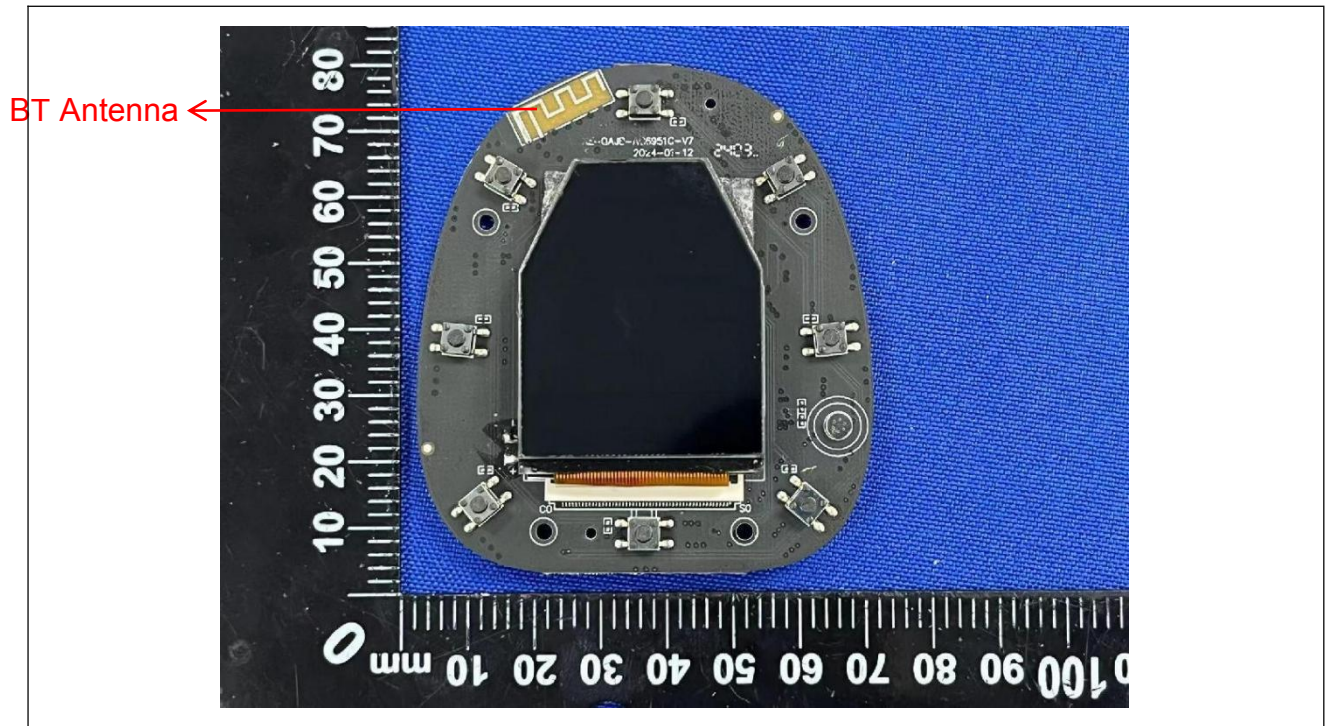
Details of: PCB components view
