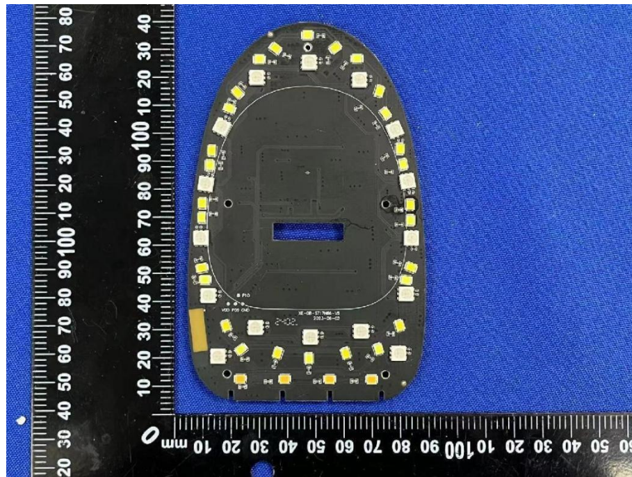
Details of: PCB components view
