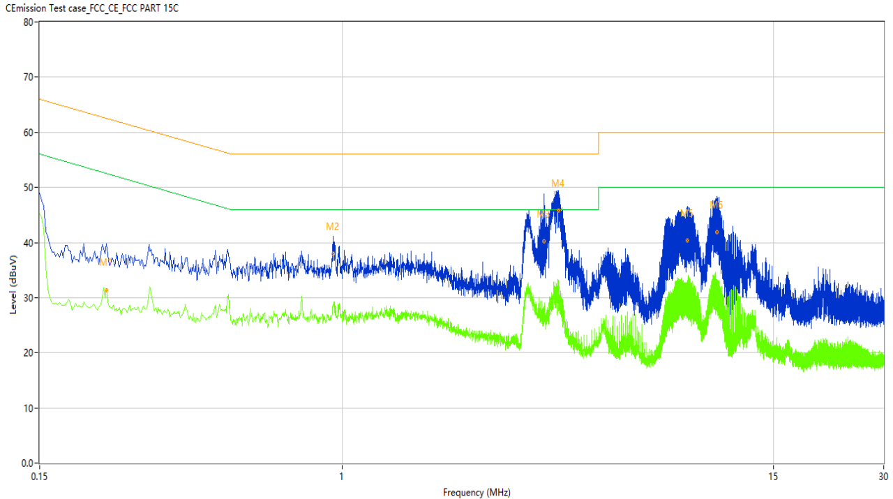
Figure 93: Conducted Emission on AC Mains, L Phase
