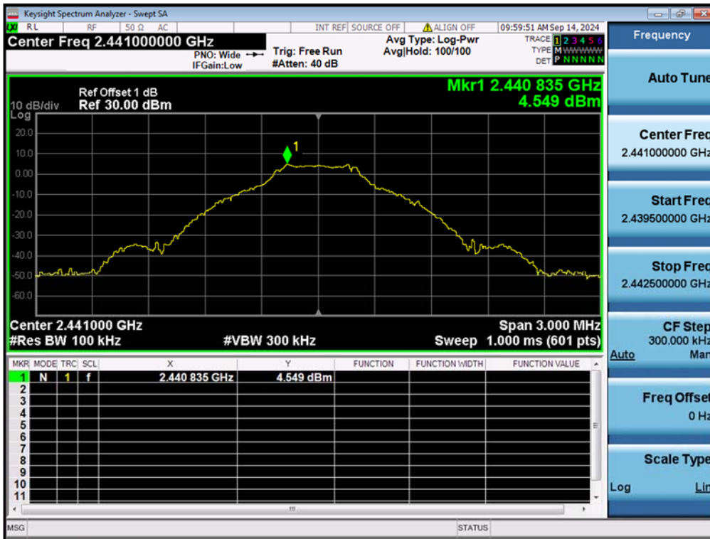
Figure 20: Conducted Spurious Emission & Authorized-band band-edge, 2441MHz, GFSK Carrier Level
