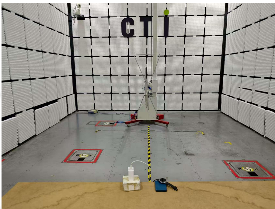
Radiated Emissions Test Setup (30MHz-1GHz)
