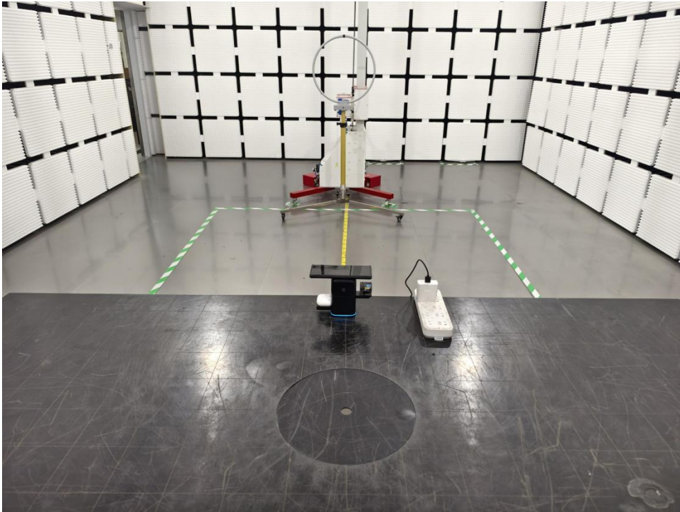
Spurious Radiation Emissions Test (9kHz<30MHz)
