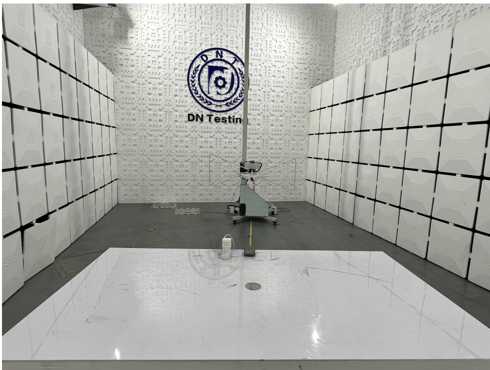
Radiated Emission Test View|(30MHz -1GHz)
