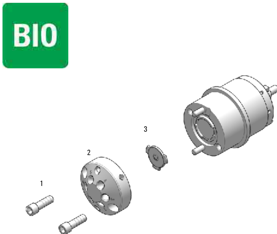
Figure 56 3-Position/6-Port FI Valve Assembly
