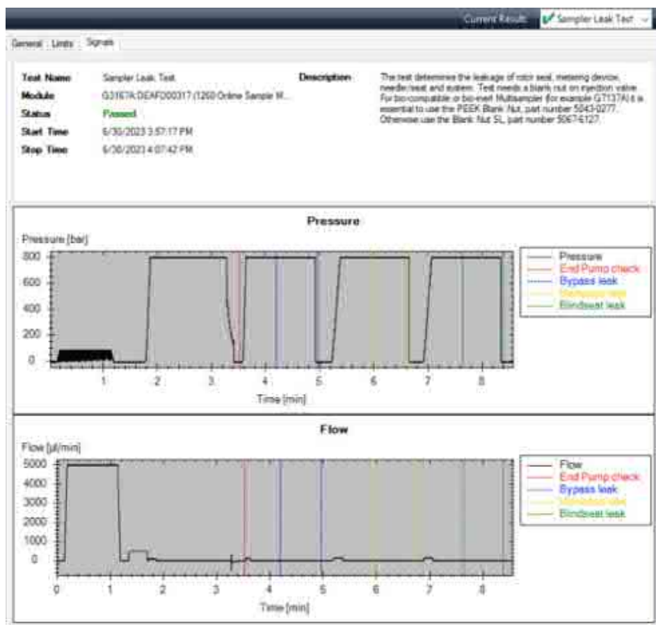
Figure 73 Sampler Leak Test passed
