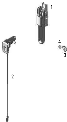
Figure 68 G3167BA Online Sample Manager Set PM Kit
