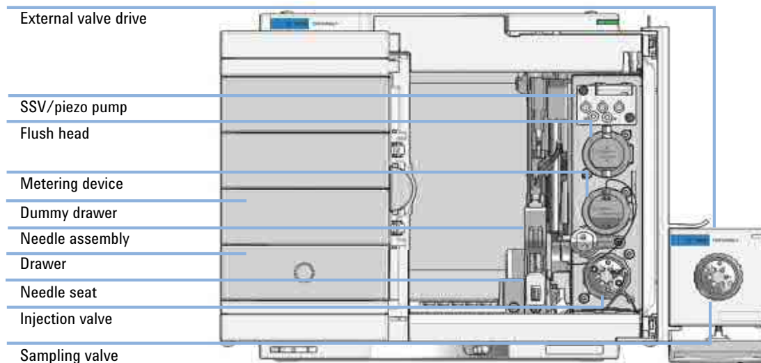
Figure 49 Main user accessible assemblies
