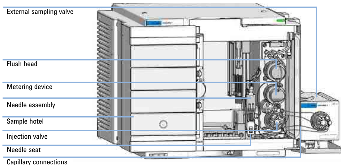
Figure 4 Overview of the hardware components of the Agilent InfinityLab Online LC Solution
