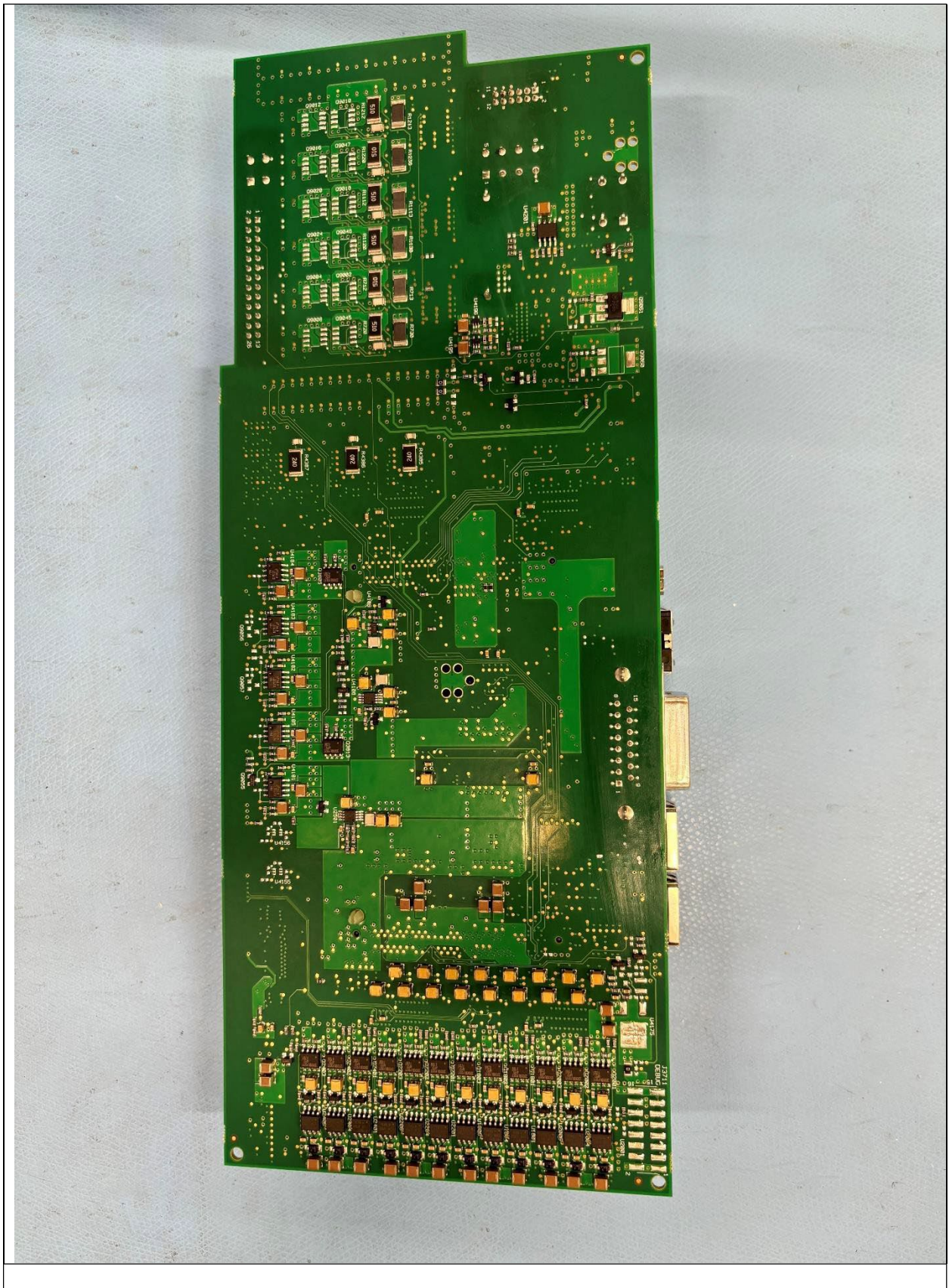
Main-Board bottom
