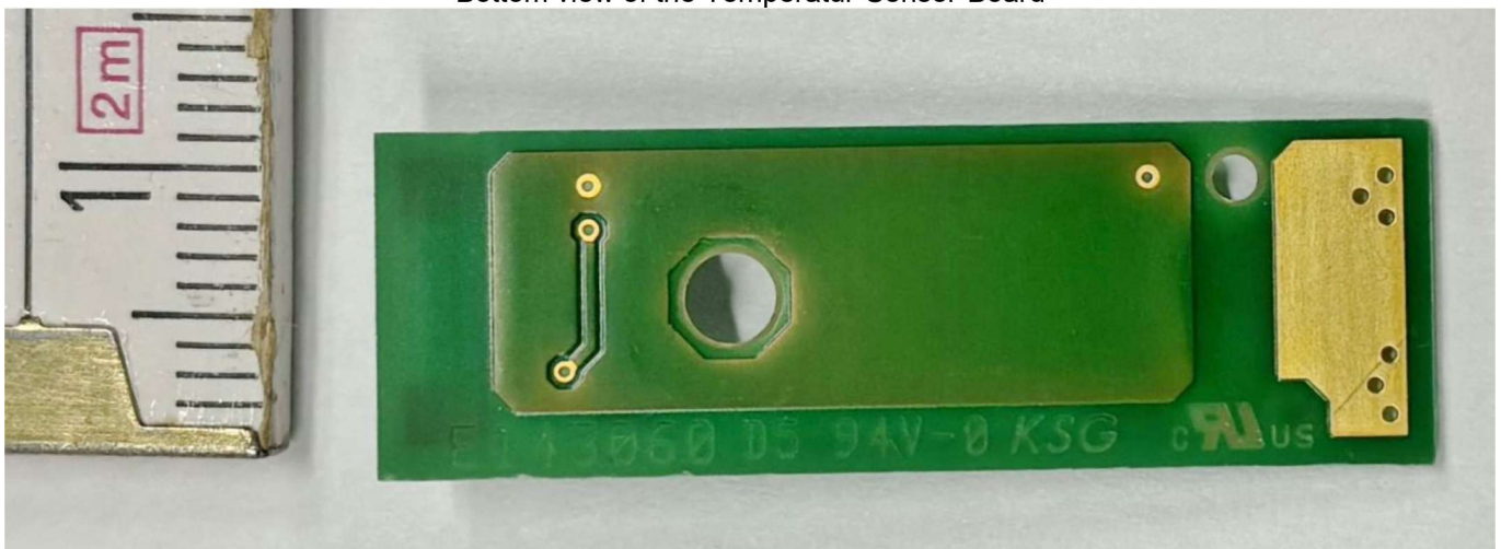
Bottom view of the Temperatur-Sensor-Board
