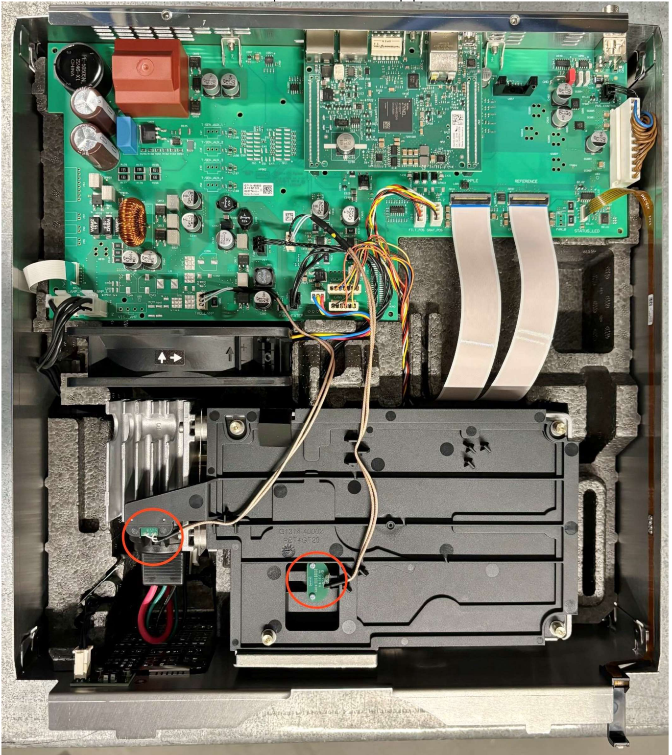
Antenna positions inside the equipment
