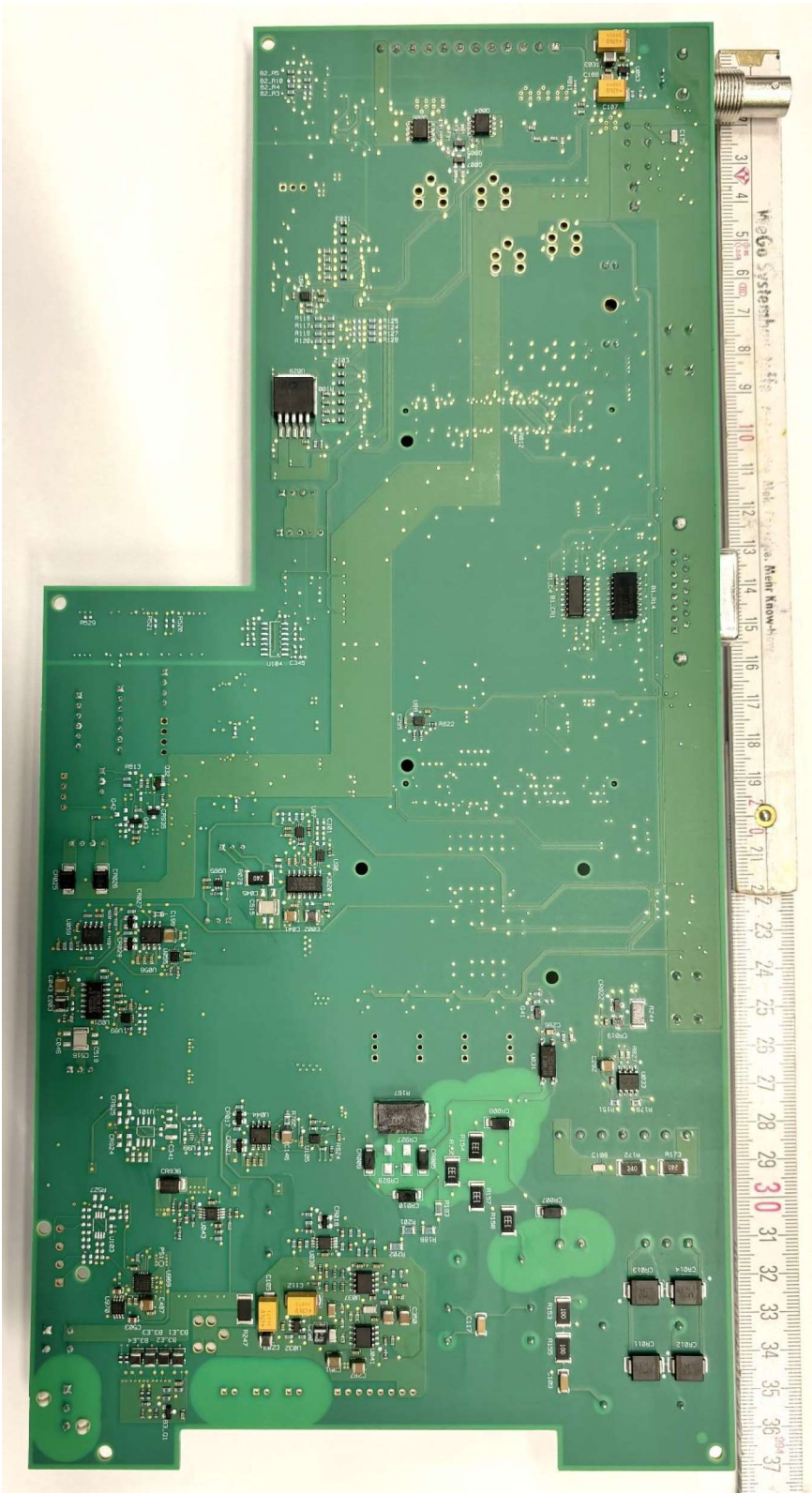
Bottom view of the Main-Board PCB
